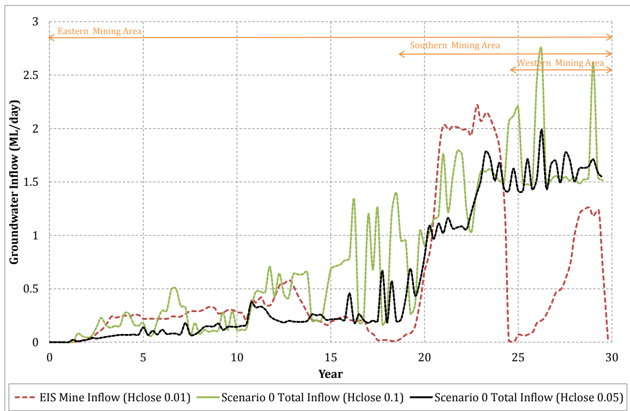
Figure 2-8 Pit seepage sensitivity to Hclose - (Scenario 0)
