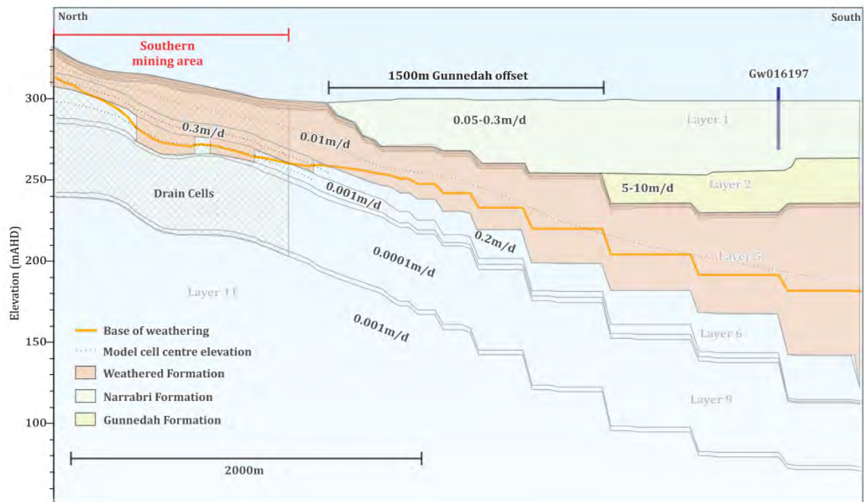
Figure 3-1 Cross-section through Southern Mining area/alluvium (Base EIS)
