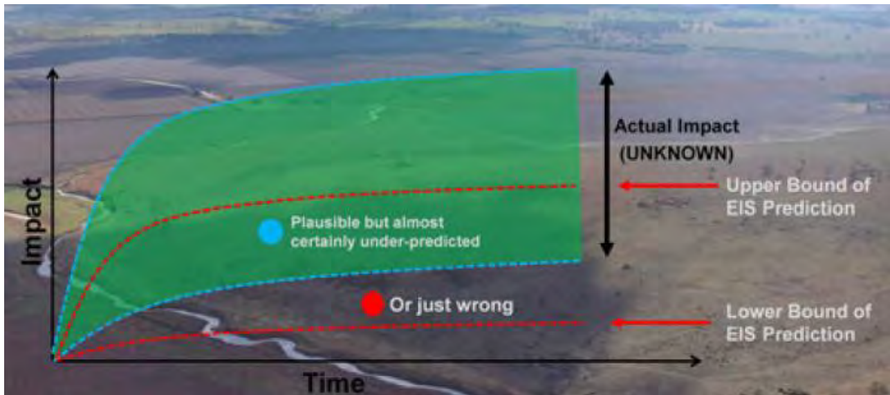
Figure 3-18 UNSW Impact Graphic
