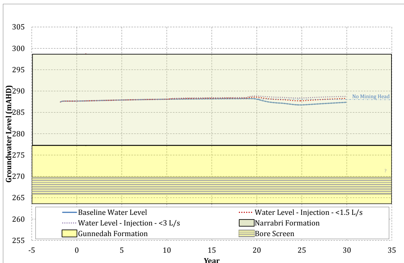
Figure 3-17 Hydrograph (GW015505) – Re-injection scenarios
