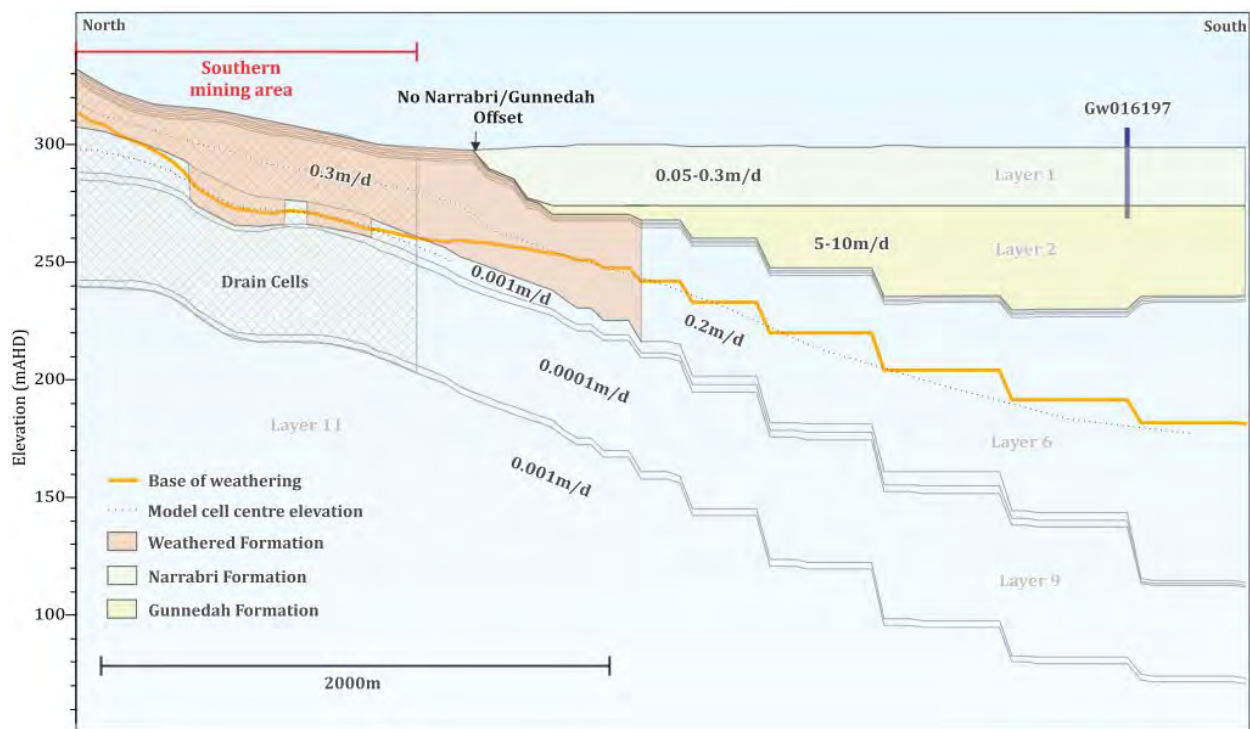
Figure 3-7 Cross section of UNSW model setup
