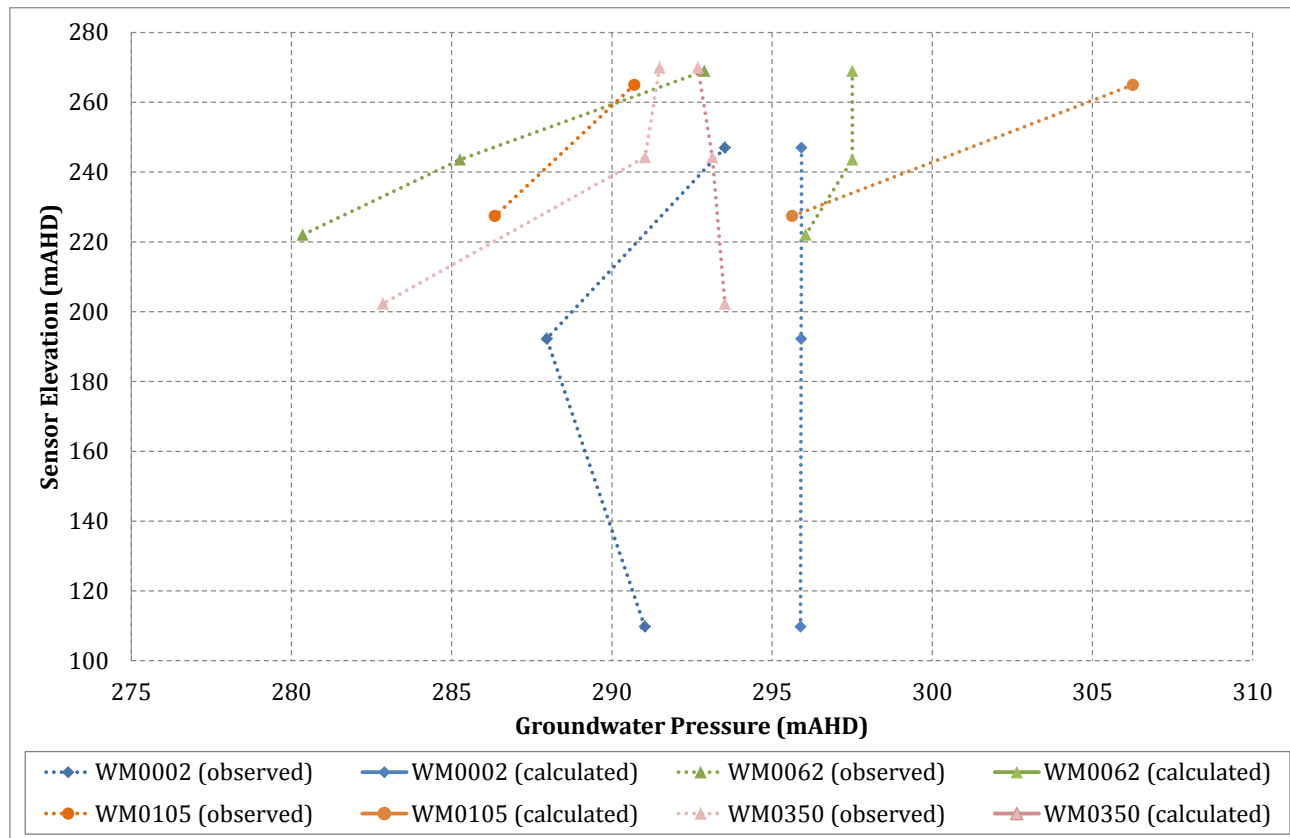
Figure 3-16 Vertical gradients (Observed vs. calculated)
