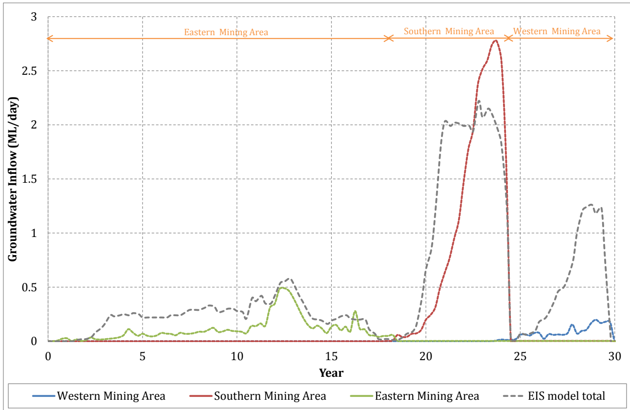
Figure 2-16 Pit seepage rates – backfilled (Scenario 11)
