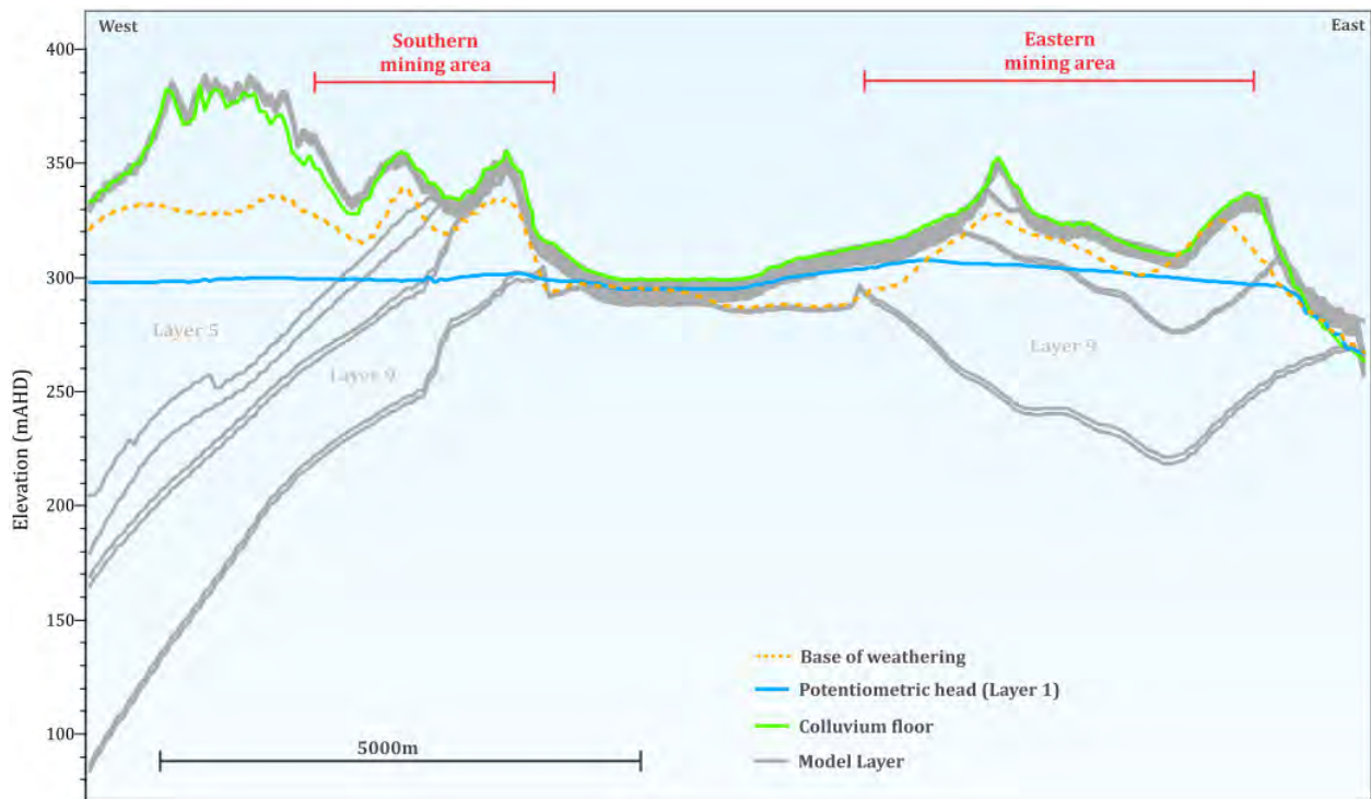
Figure 3-4 Cross-section showing colluvial extent (W-E)
