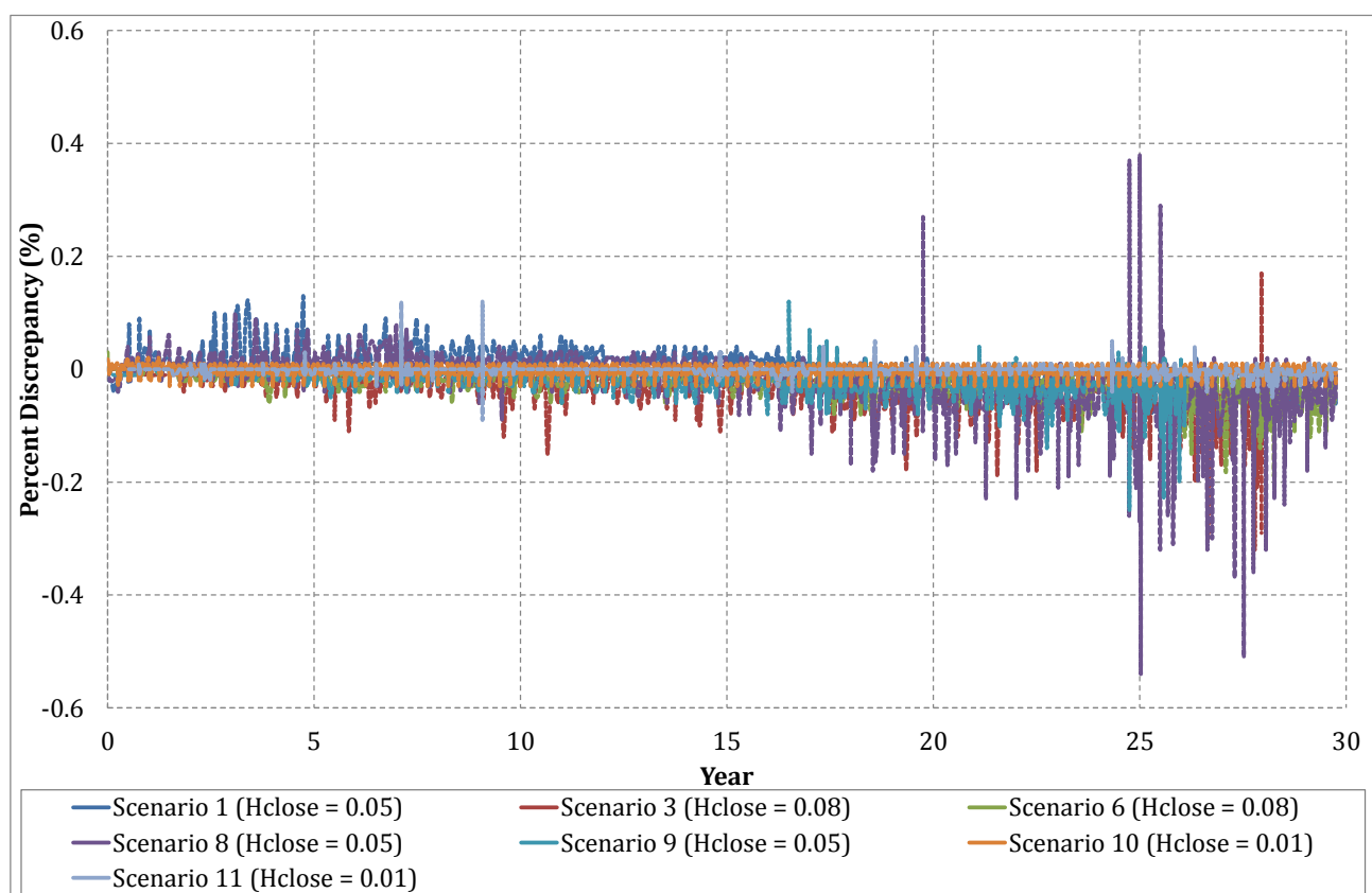
Figure 2-9 Percent discrepancy error
