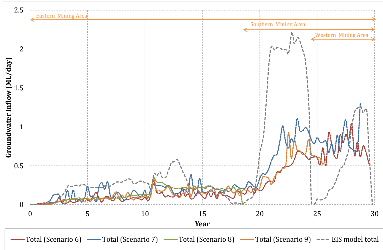
Figure 2-21 Pit seepage sensitivity
