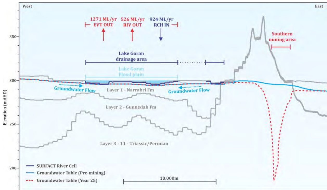
Figure 3-15 Cross section through Lake Goran
