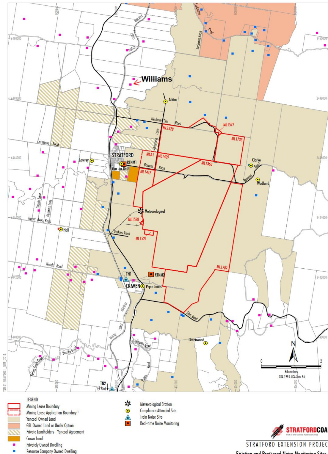
Figure 1 Existing and Proposed Noise Monitoring Locations
