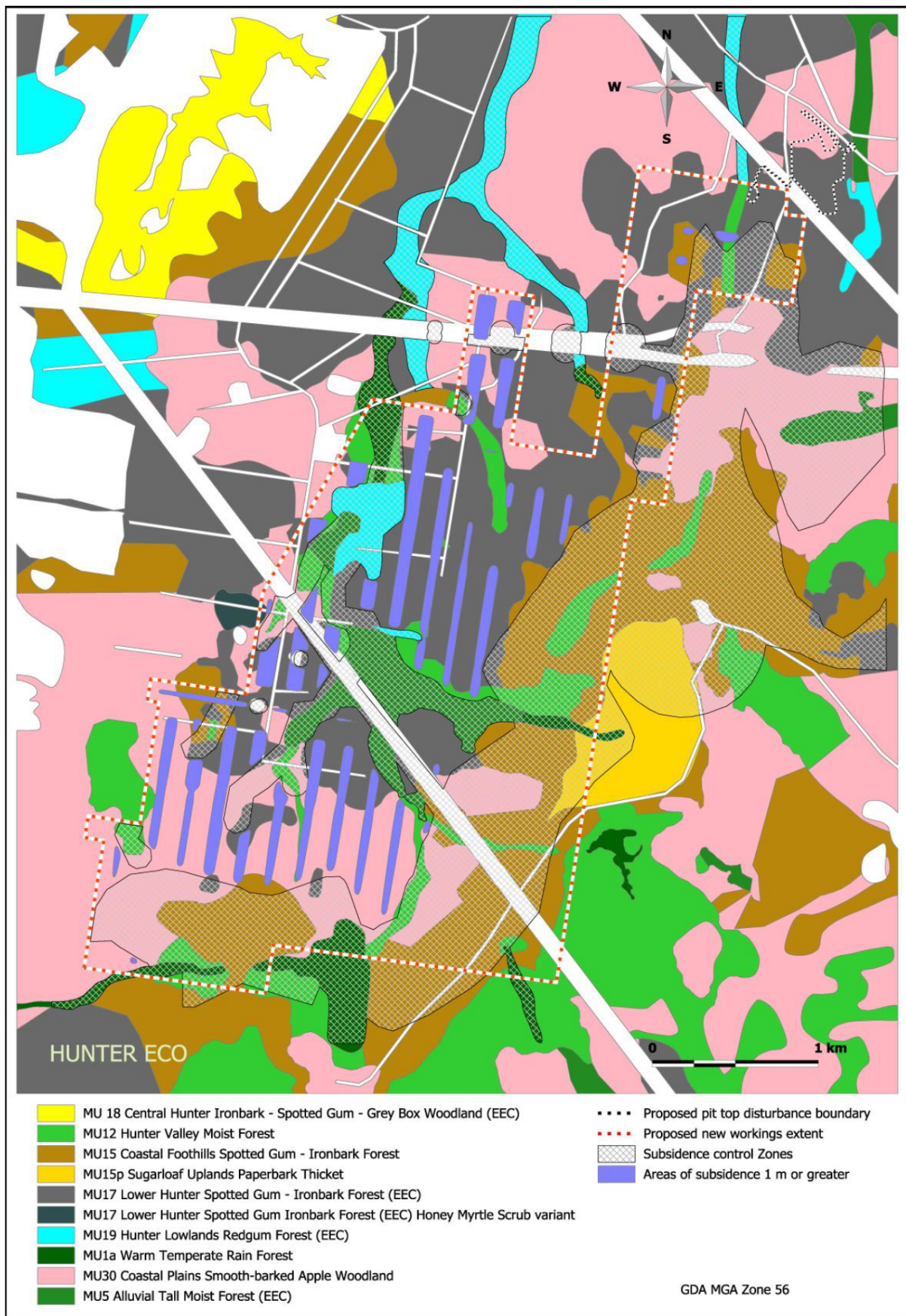
Figure 13: Vegetation Communities in the Development Area & Subsidence Control Zones
