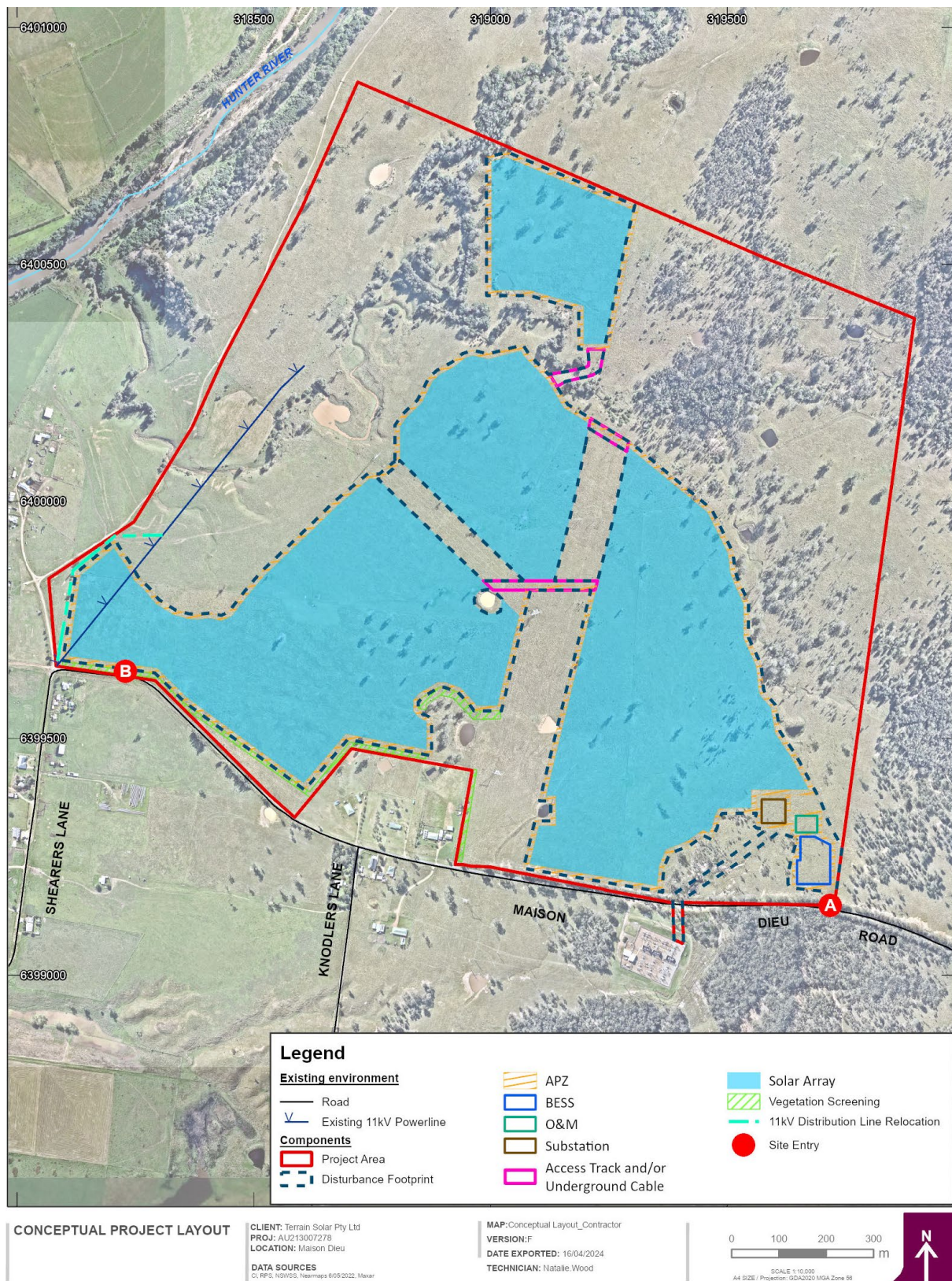
Figure 3-2 Conceptual Project Layout
