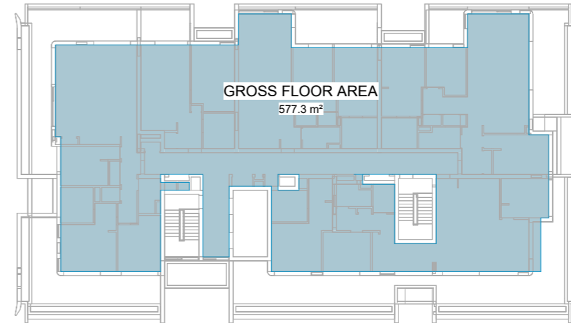
DA BUILDING B - AREA PLAN - GFA - LEVEL 03 LEVEL 03
