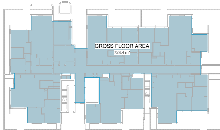
AREA PLAN (GFA) GROUND FLOOR
