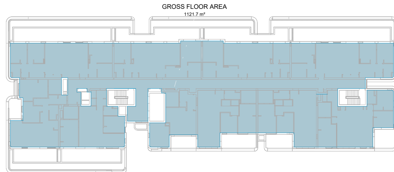
AREA PLAN (GFA) LEVEL 01
