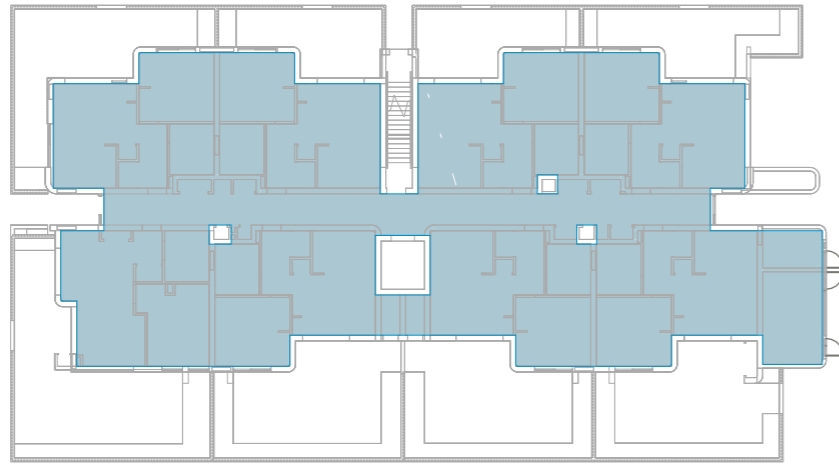
AREA PLAN (GFA) GROUND FLOOR
