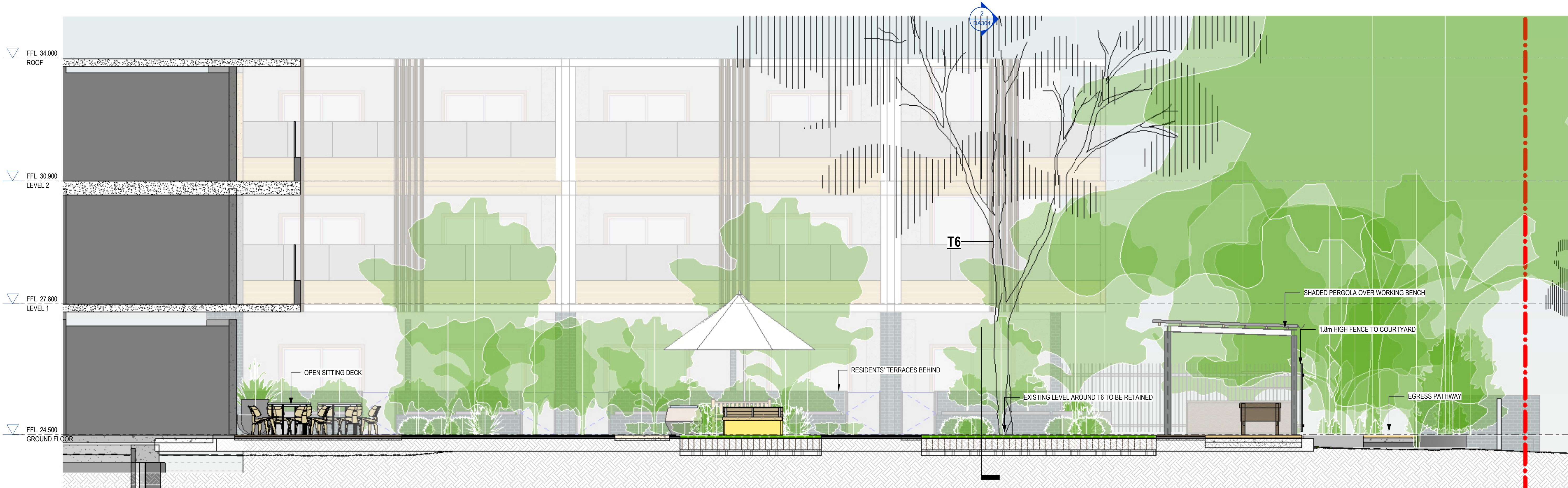
3 Boundary Section - West 2 1 : 50
