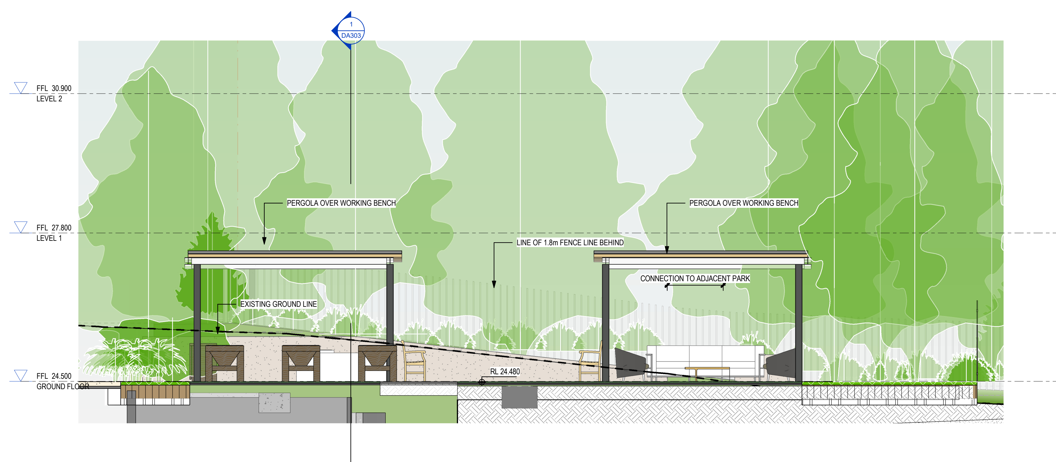
2 Boundary Section - South East 2 1 : 50
