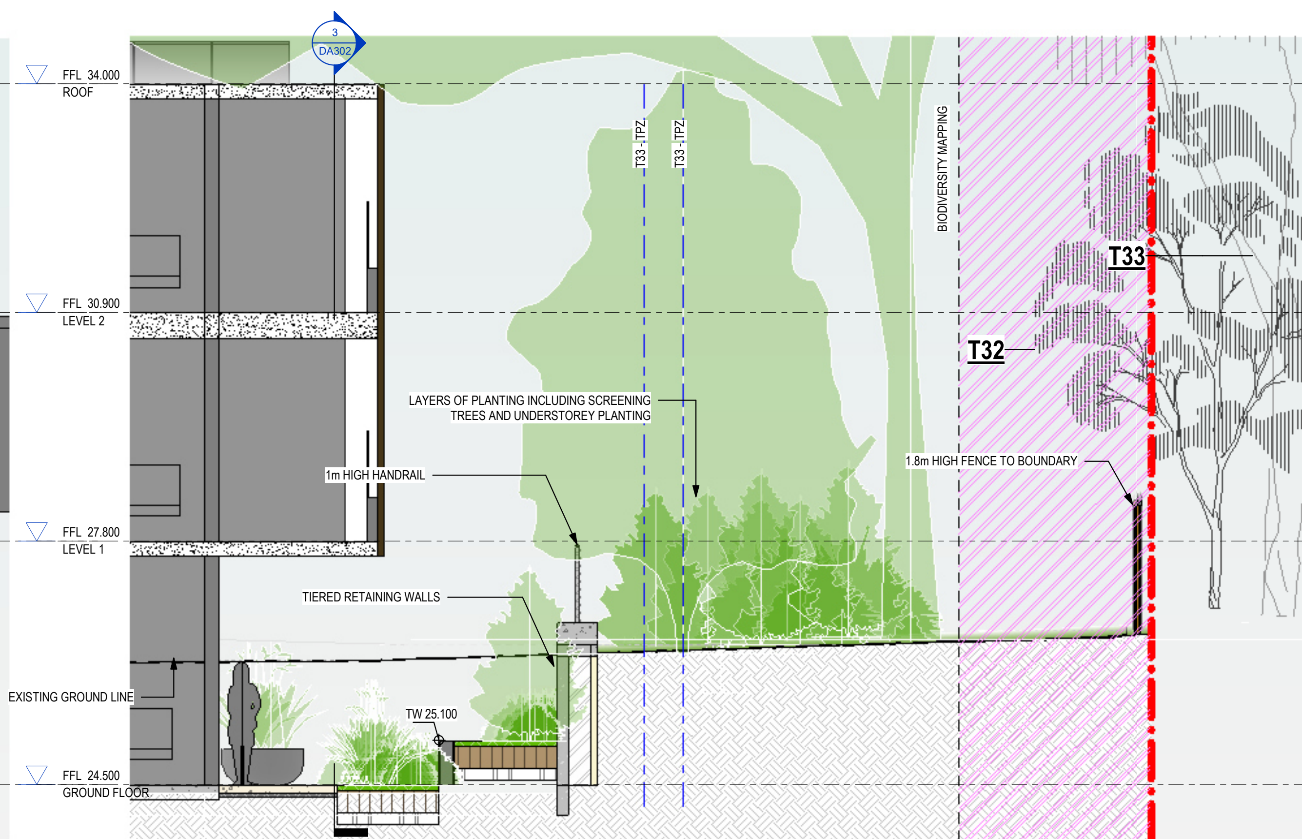
2 Boundary Section - East 2 1 : 50
