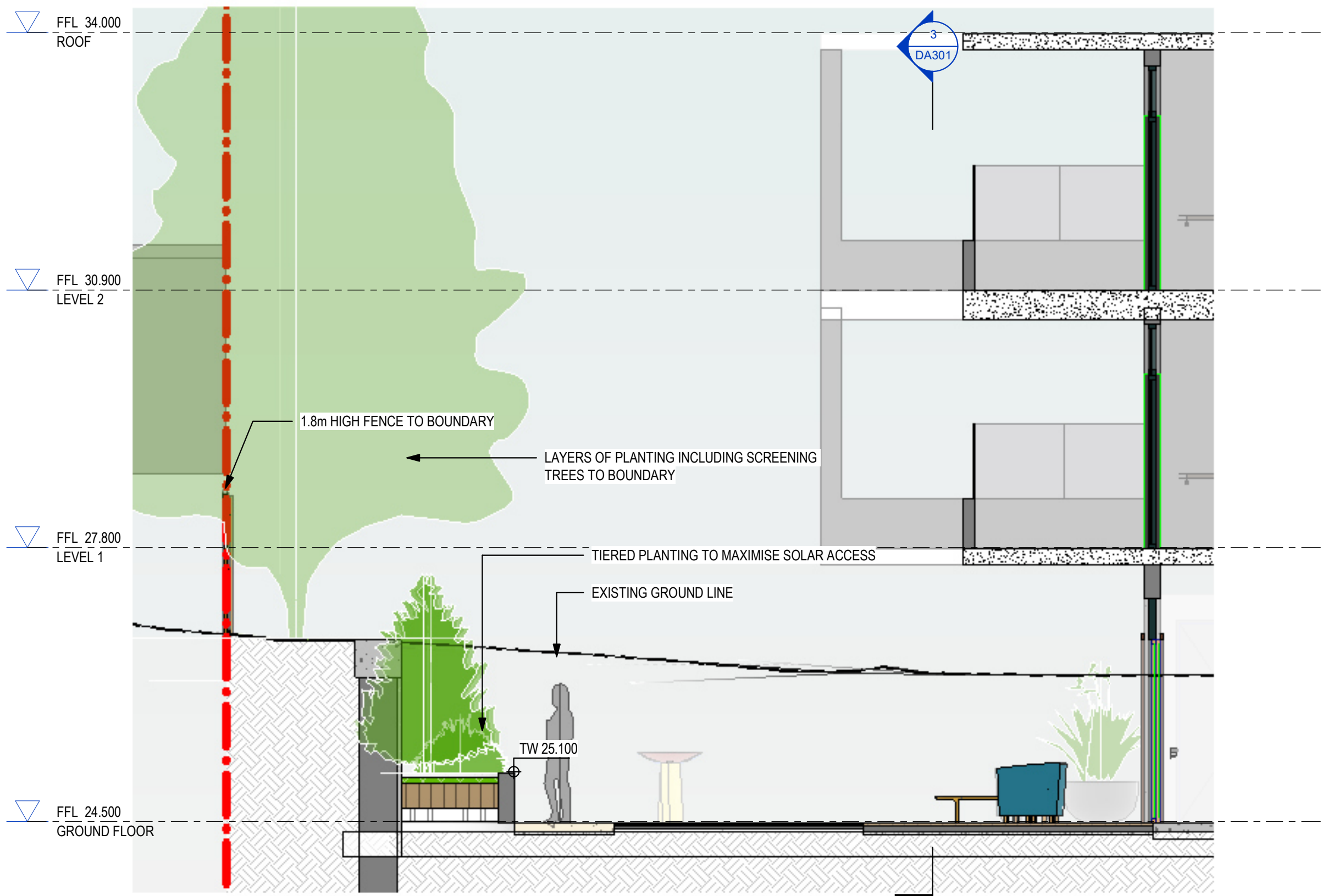
2 Boundary Section - North 2 1 : 50
