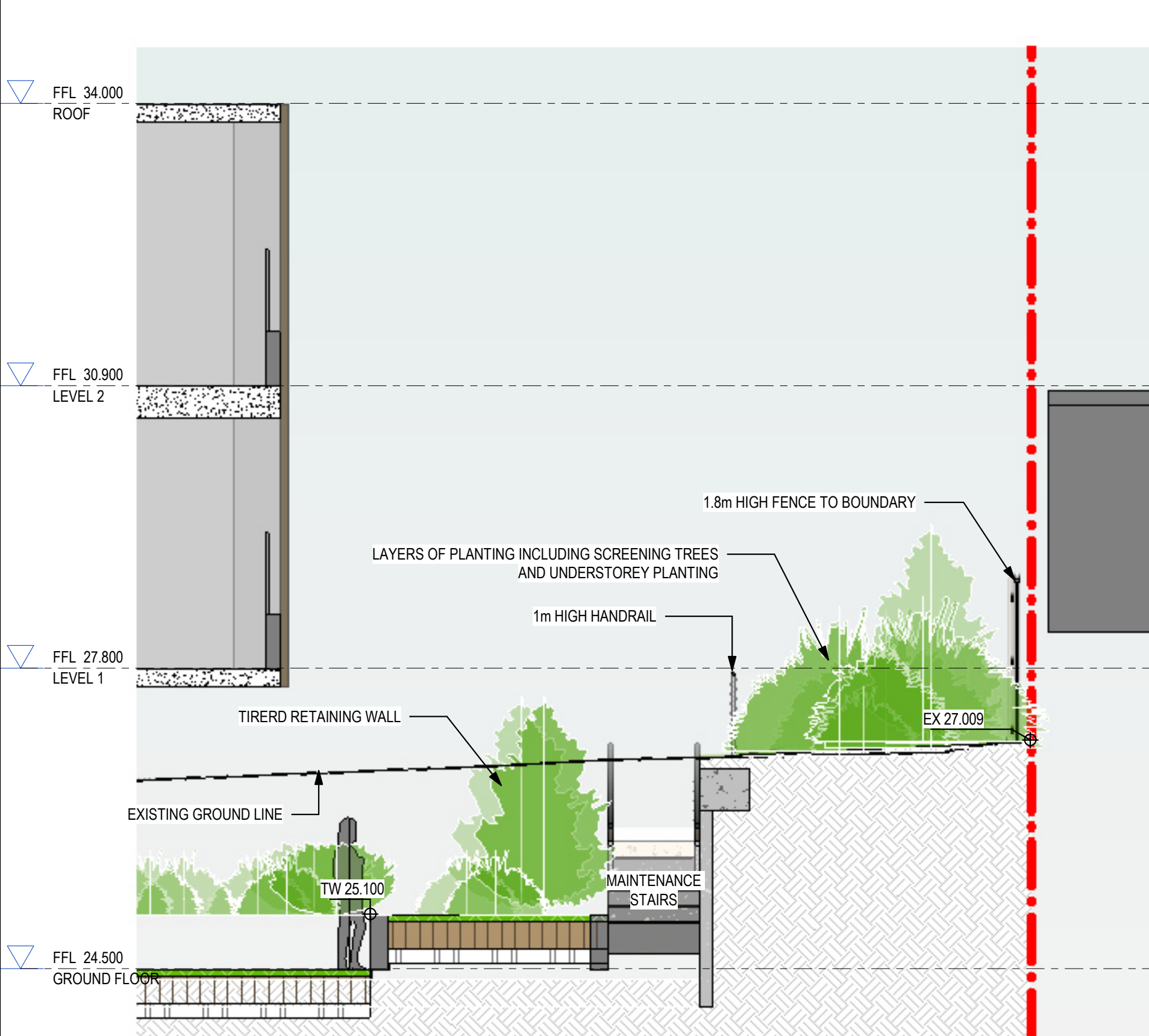
1 Boundary Section - East 1 1 : 50
