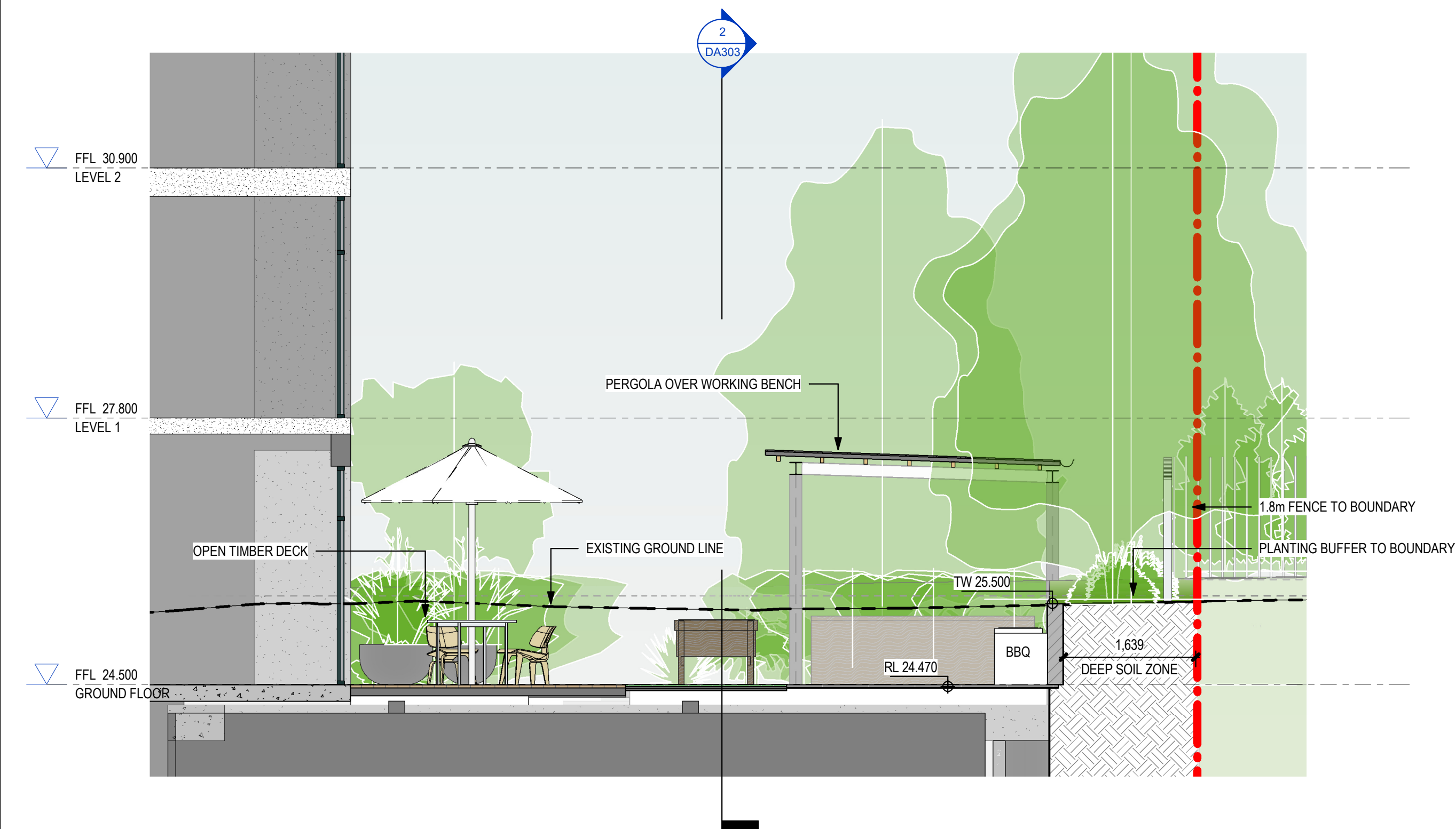
1 Boundary Section - South East 1 1 : 50
