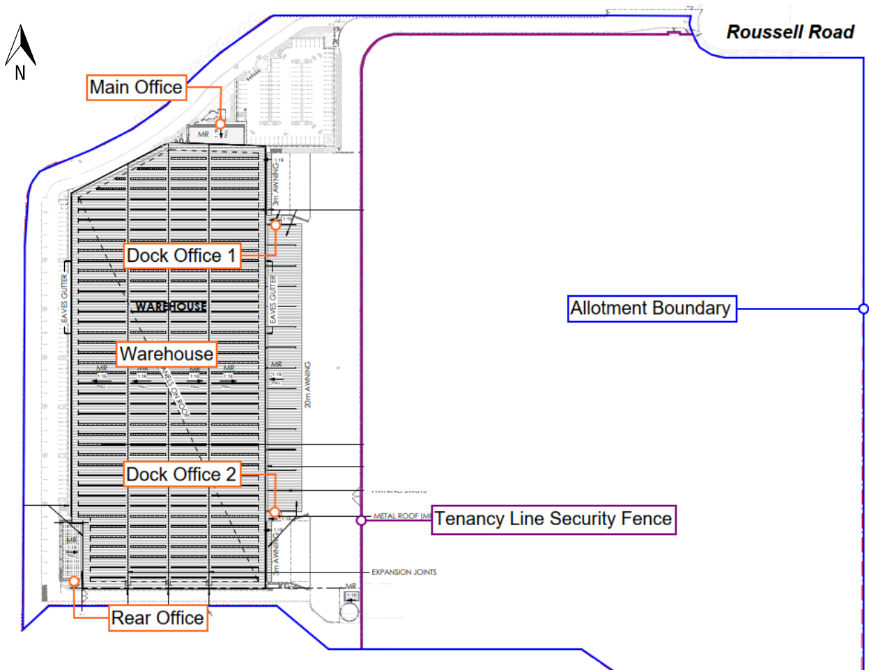
Figure 2-3: Site Plan and Building Description
