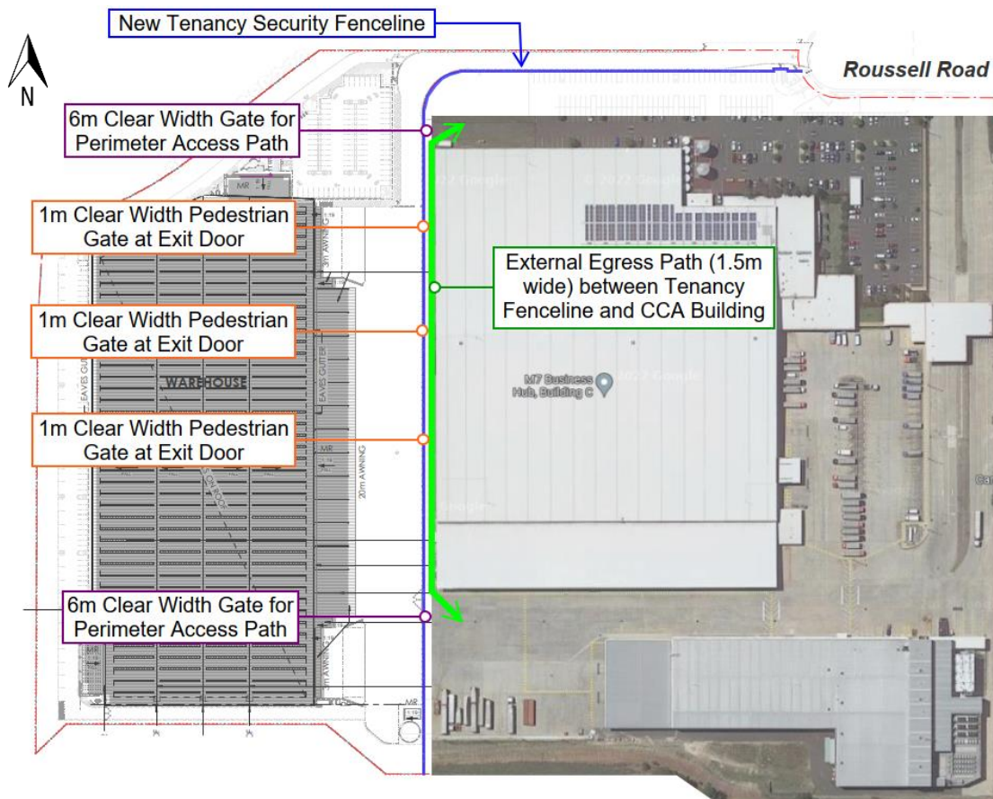
Figure 6-1: Access and Gate Requirements for the New Tenancy Security Fence
