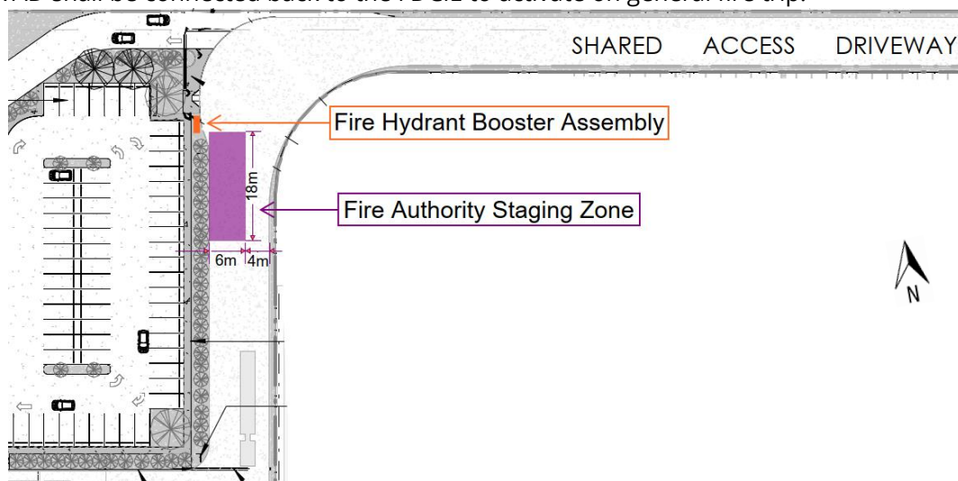
Figure 6-5: Fire Hydrant Booster Assembly & Fire Appliance Staging Zone
