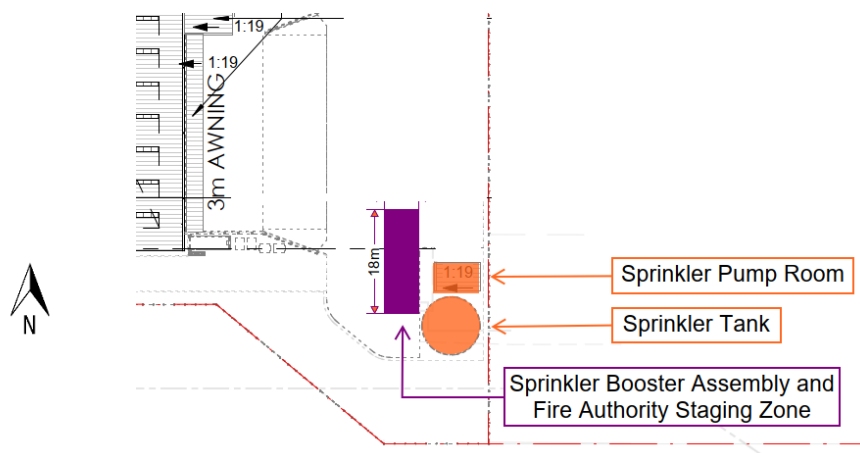
Figure 6-3: Fire Sprinkler Infrastructure & Fire Appliance Staging Zone
