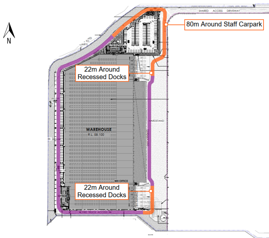
Figure 6-6: Vehicular Perimeter Access Path Around the Building
