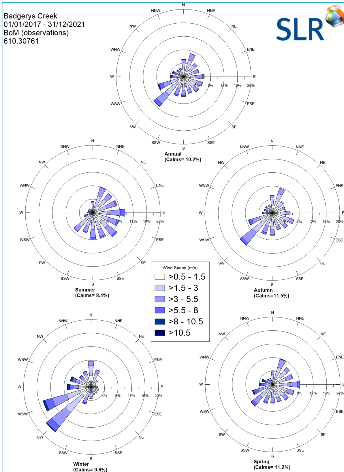
Figure 5 Annual and Seasonal Wind Roses for Badgerys Creek AWS (2017-2021)
