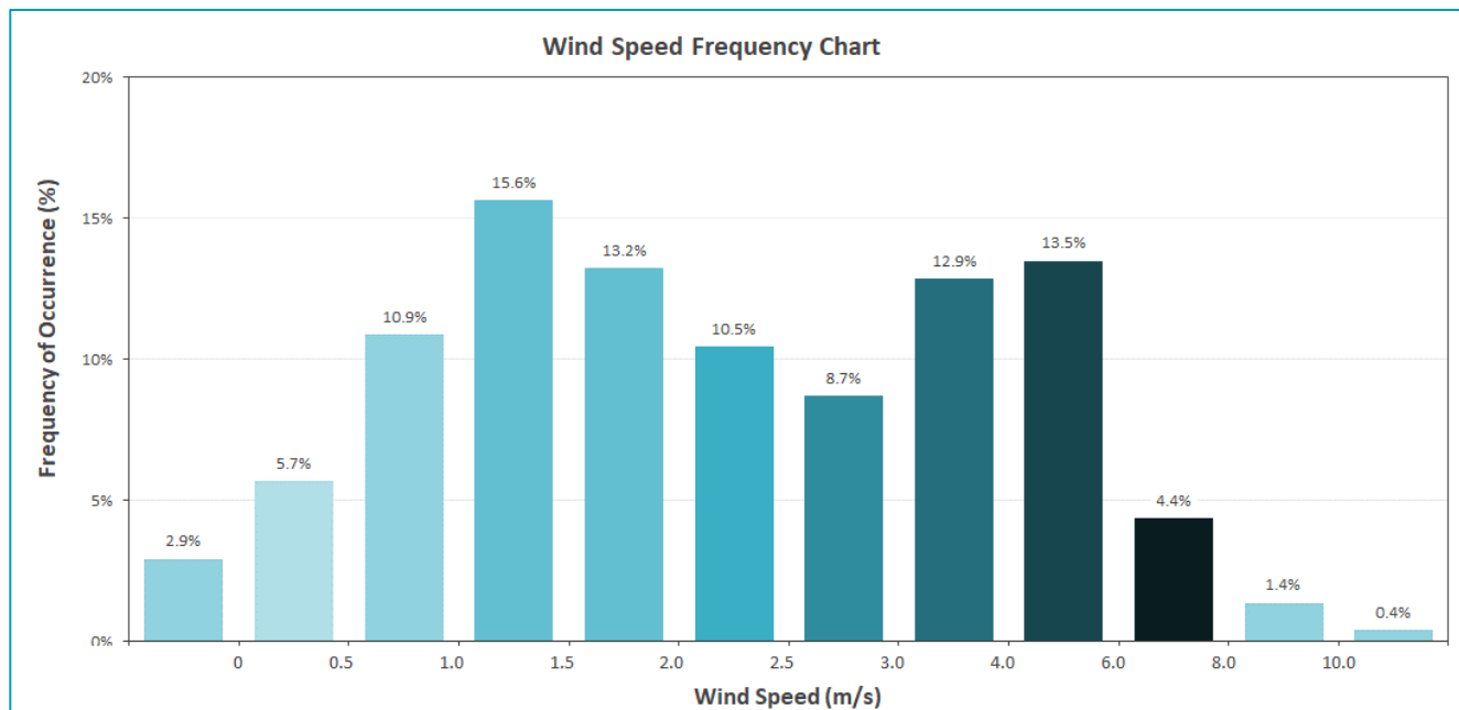
Figure 4 Wind Speed Frequency Chart for Badgerys Creek AWS (2017 – 2021)
