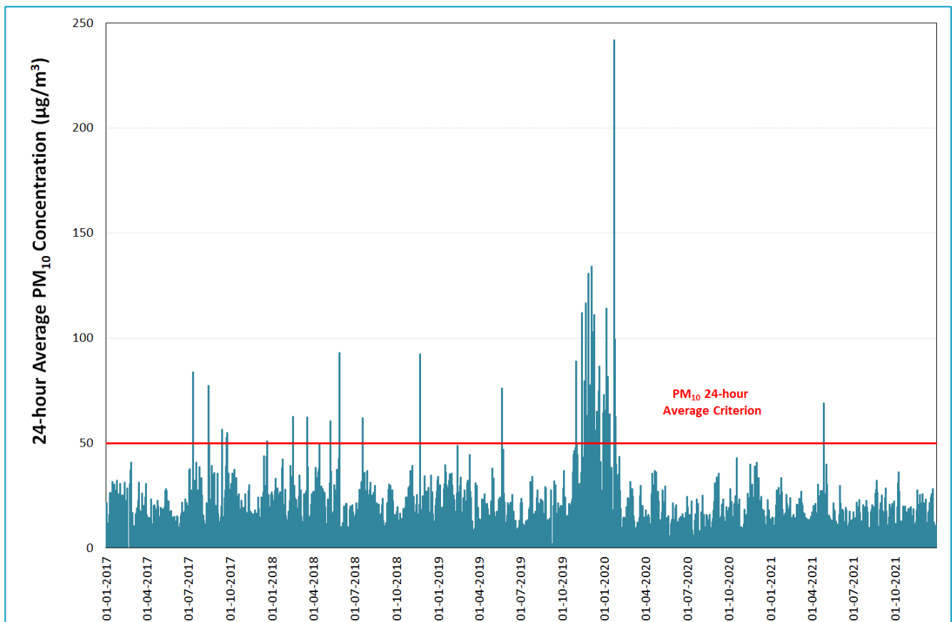
Figure 7 Measured 24-Hour Average PM_{10} Concentrations at Bringelly AQMS (2017 - 2021)
