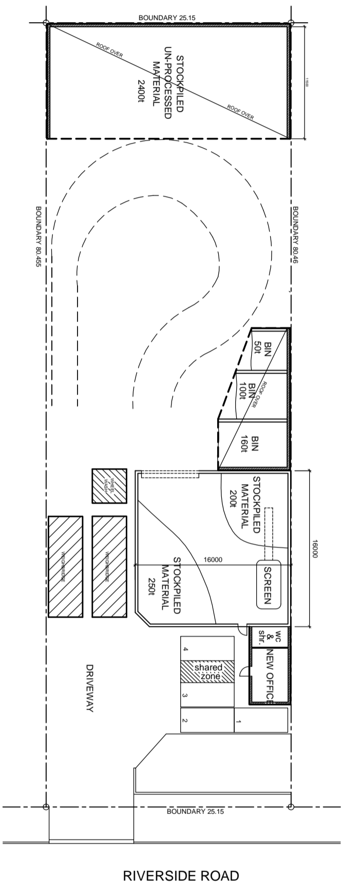
SITE AND FLOOR PLAN
