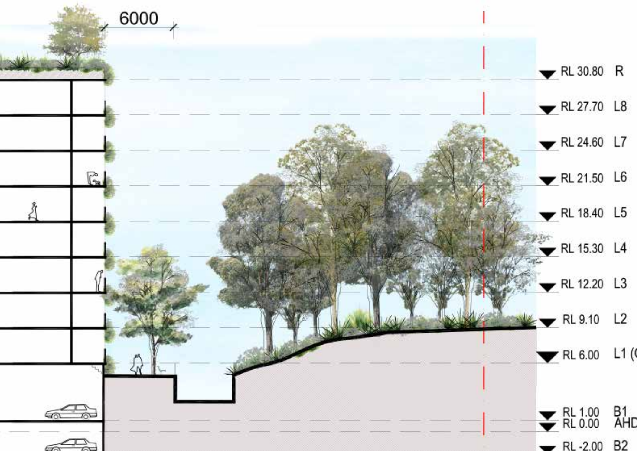
Section 4 - Clay Cliff Creek Interface
