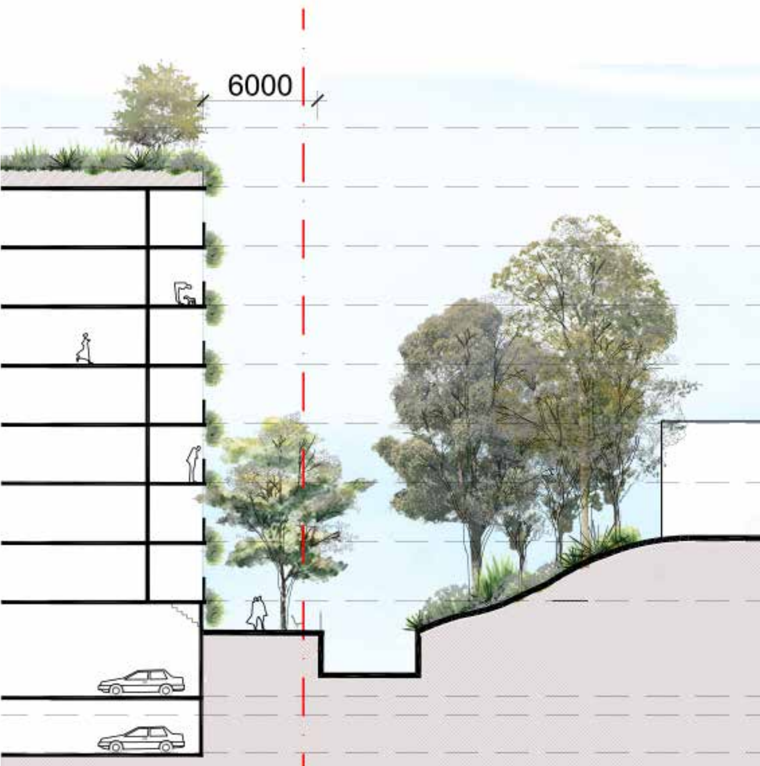
Section 1 - Clay Cliff Creek Interface
