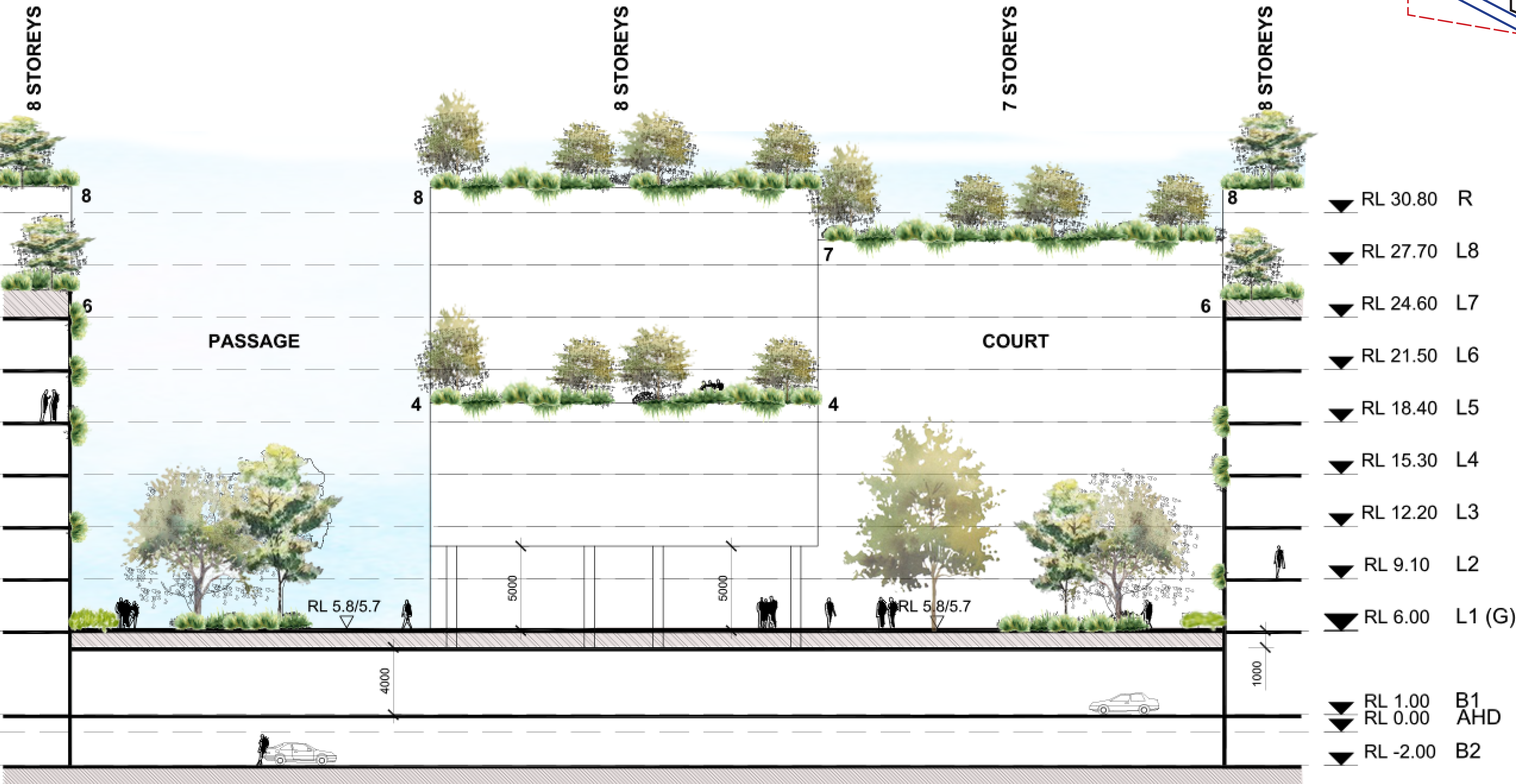
Section BB - Through Community Heart
