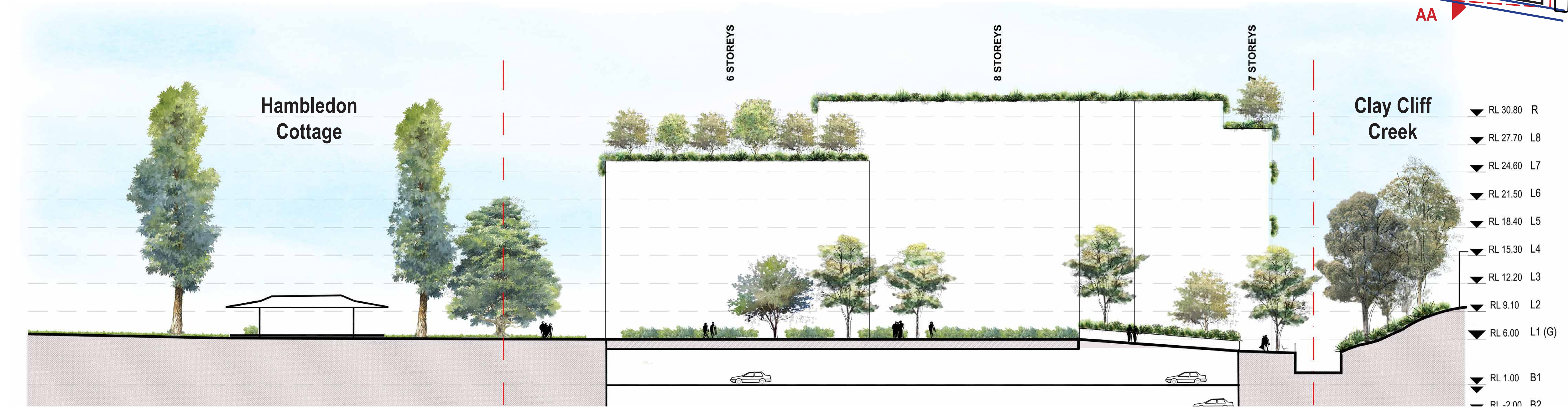
Section AA - Through Community Heart
