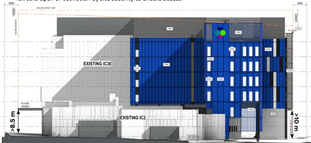
Figure 19: Northern Elevation | Overhang over the emergency vehicle path
