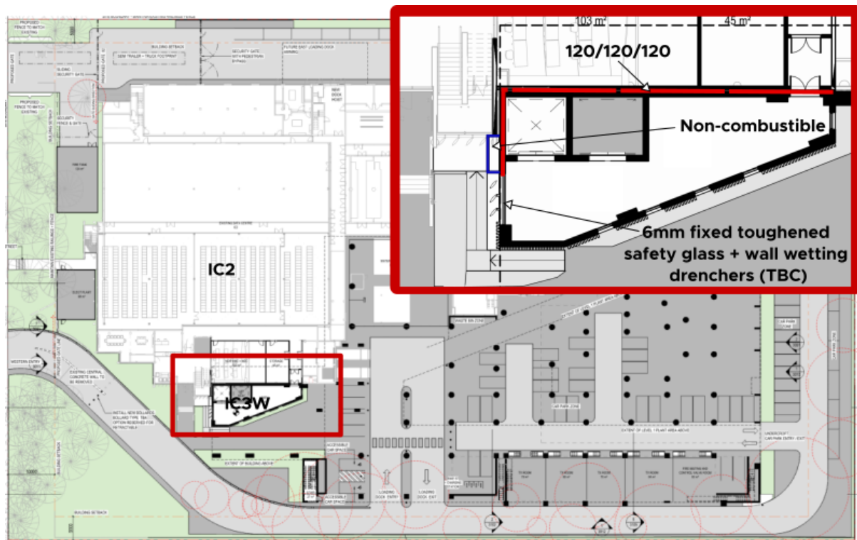
Figure 13: Exposure between administration areas of IC2 and IC3W
