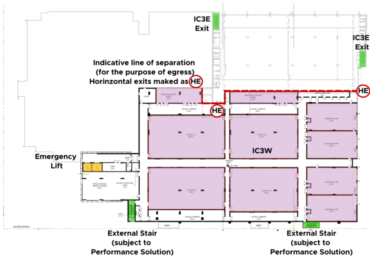
Figure 9: Indicative Compartmentation plan (Level 1 shown) – Option 1
