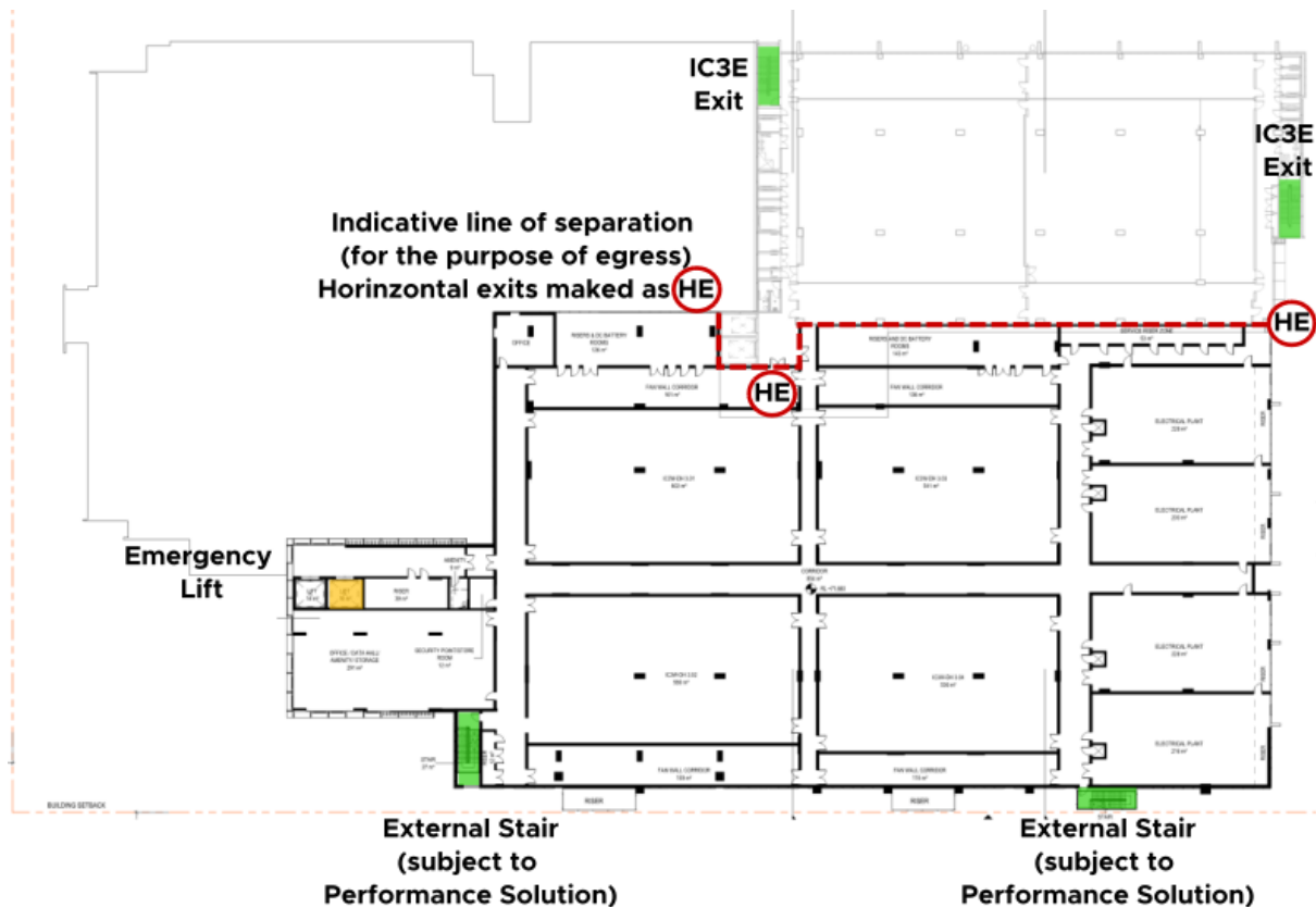
Figure 6: Level 3 Preliminary Egress Arrangement
