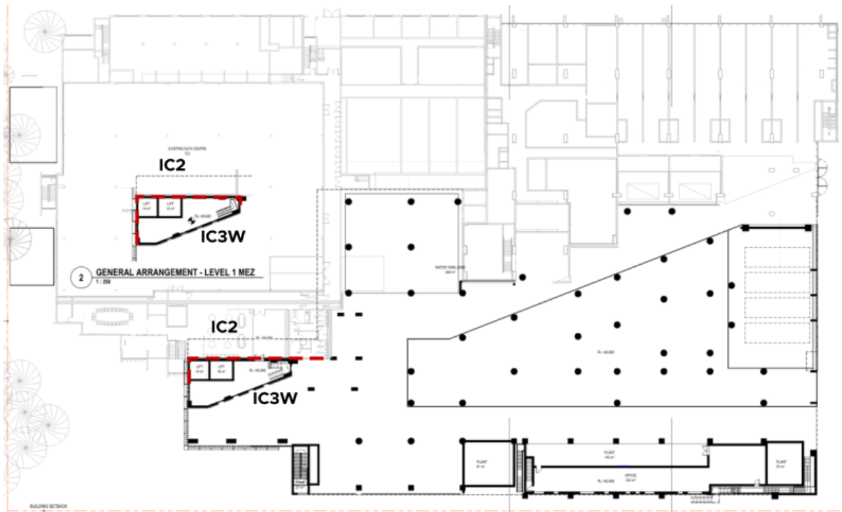
Figure 15: Egress from the Ground, Level 1 and Level 1 mezzanine office arrangement
