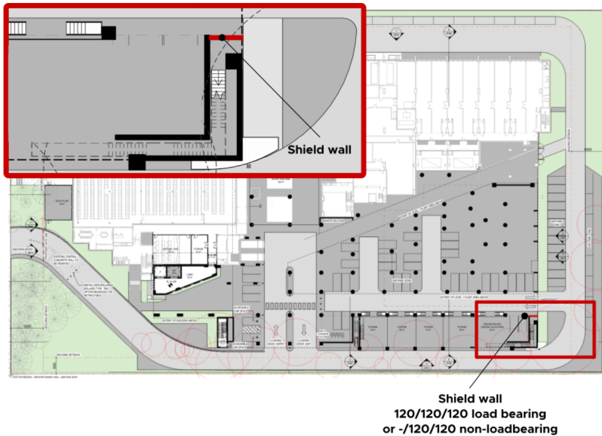
Figure 16: Protection of the External Stair from the Carpark
