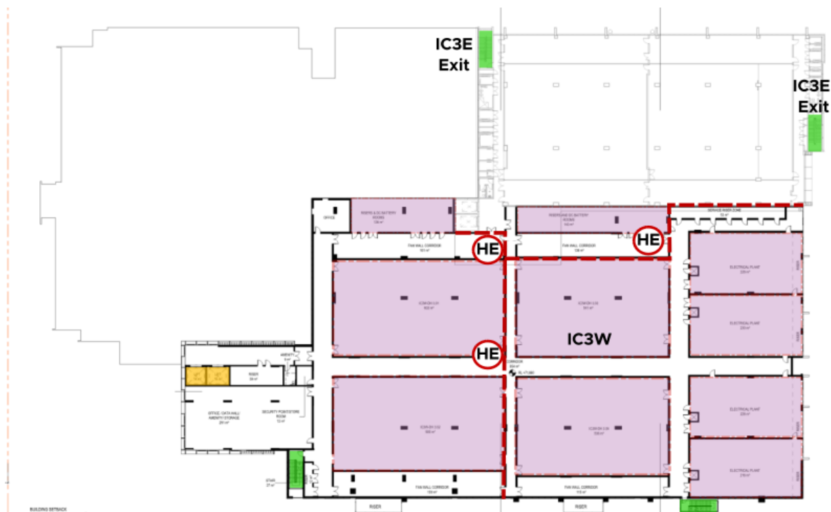
Figure 10: Indicative Compartmentation plan (Level 1 shown) – Option 2
