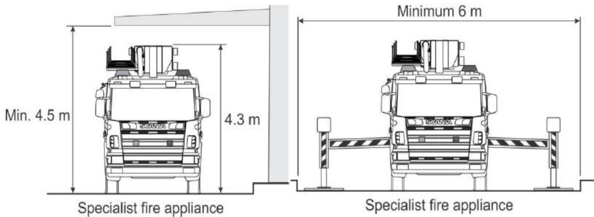
Figure 18: Overhead and width clearance requirements (from FRNSW fire safety guidelines v05)
