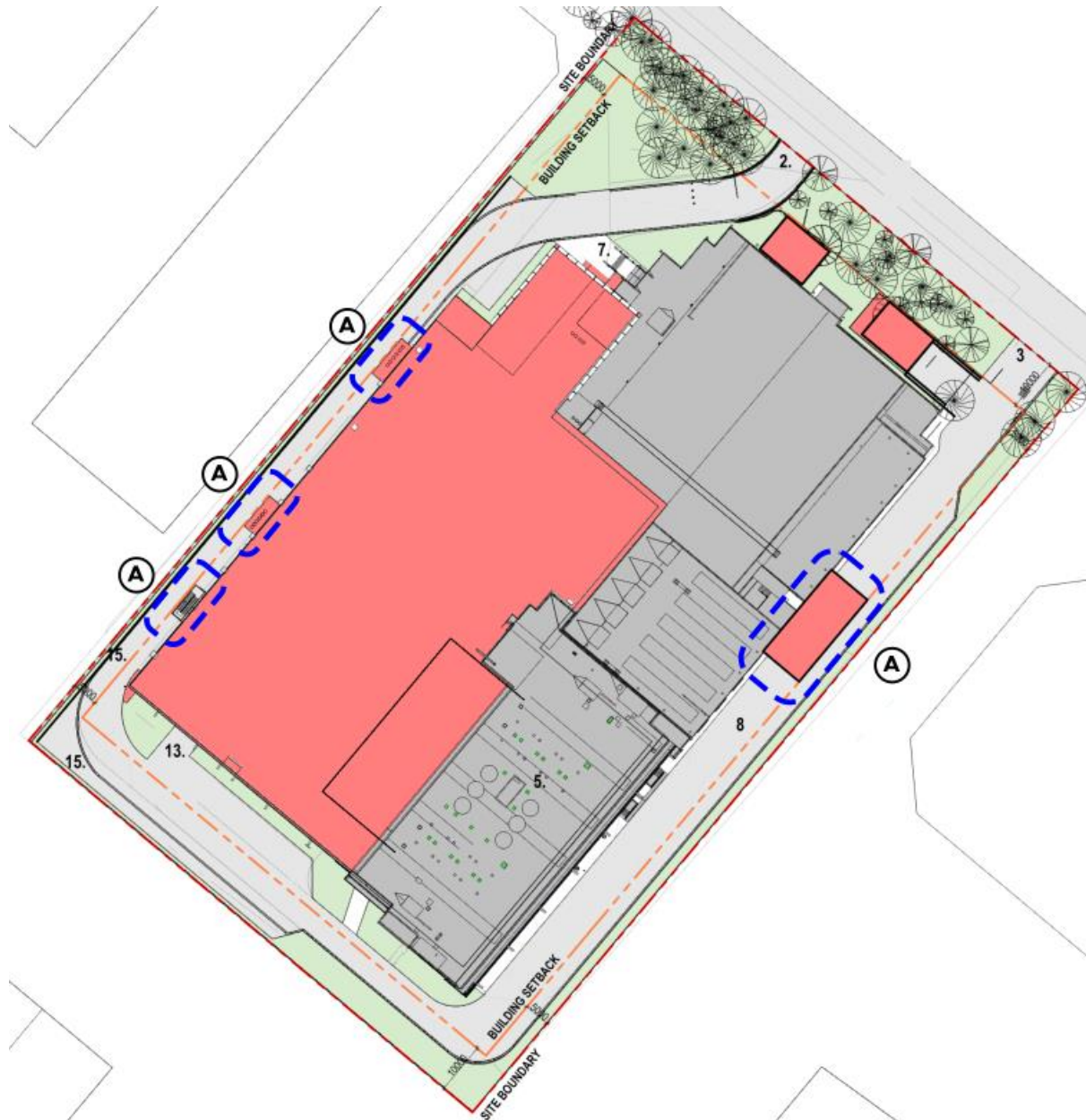
Figure 17: Overhang over the emergency vehicle path
