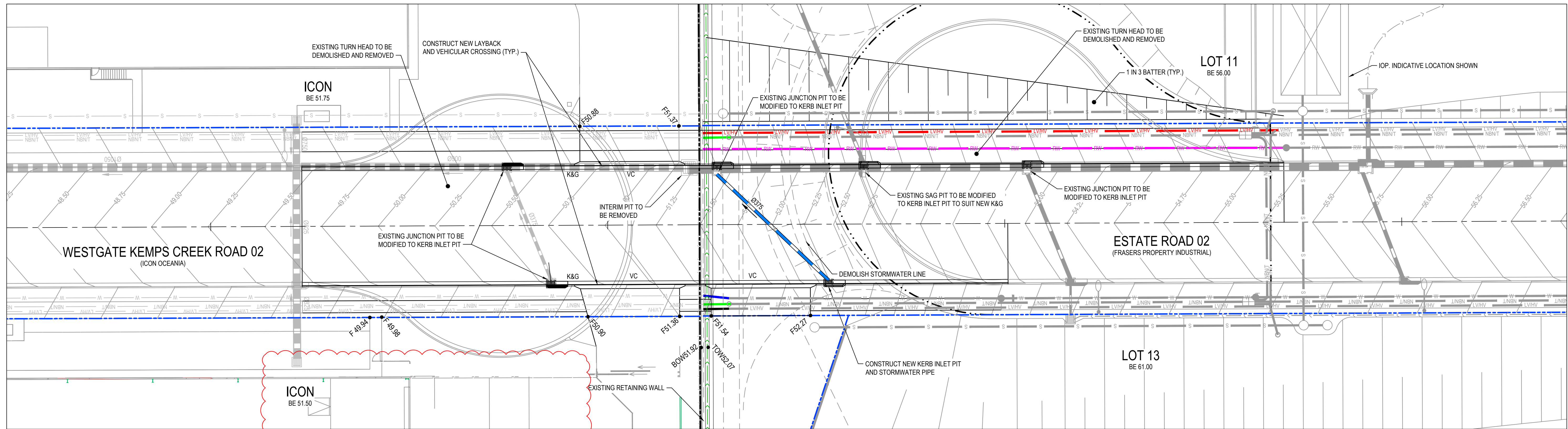
FUTURE ROADWORKS PLAN
