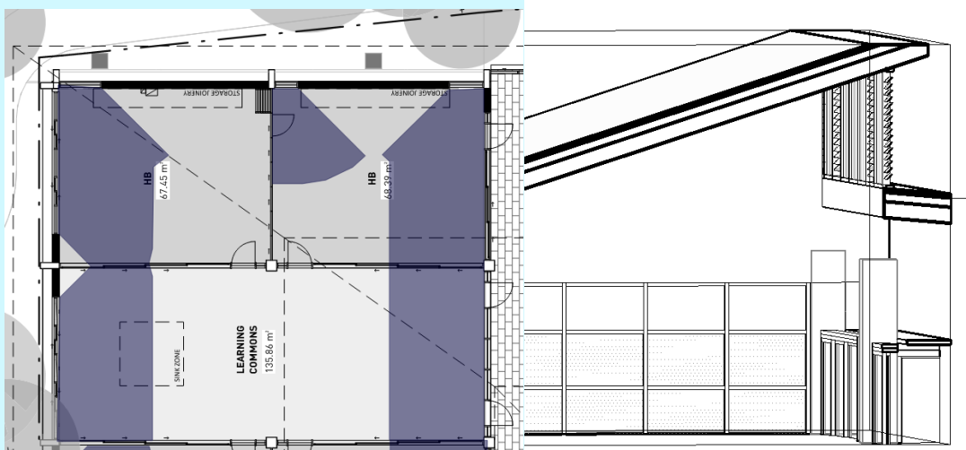
Figure 4 Example Daylight Coverage and clerestory windows
