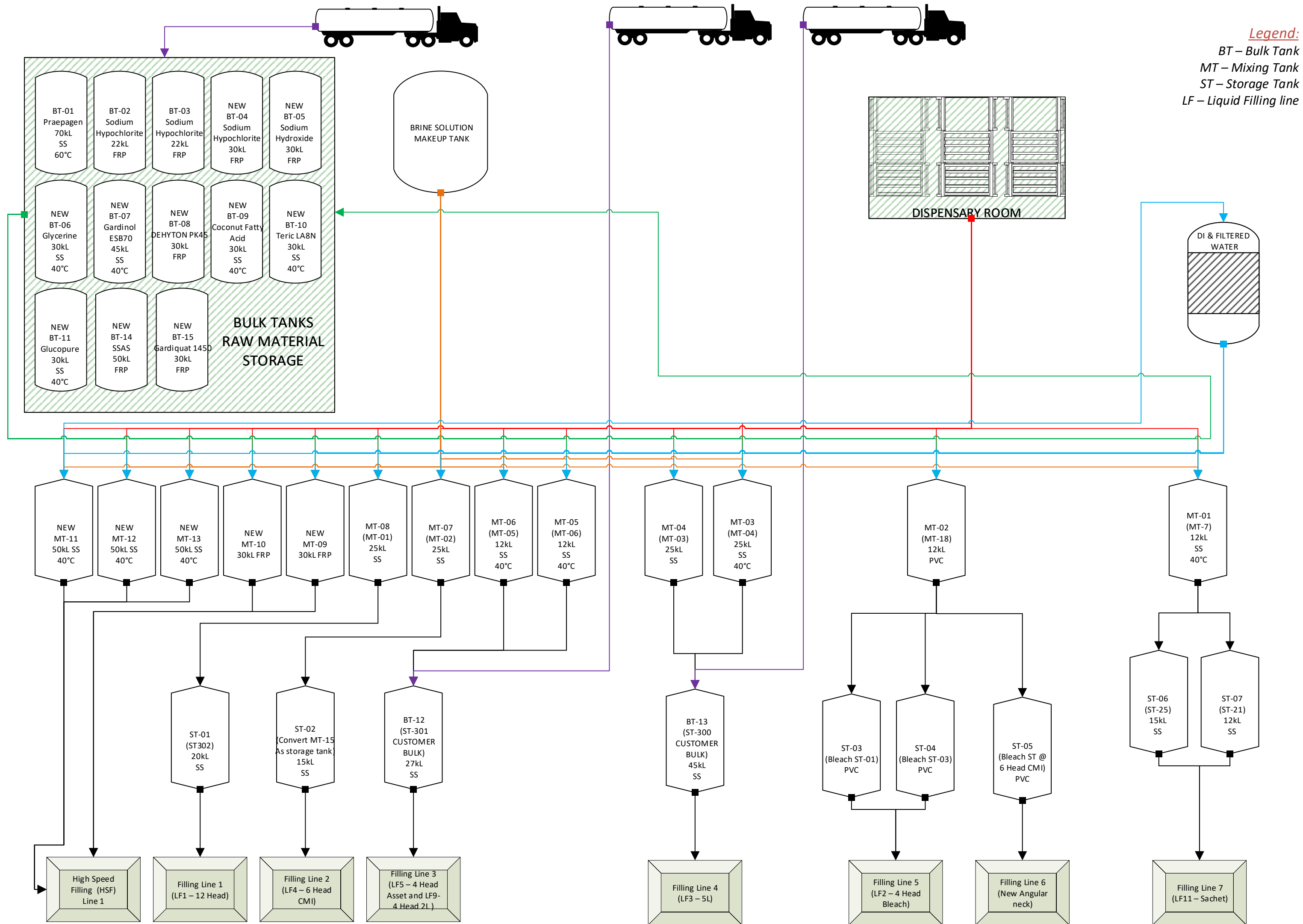
Process Flow Diagram and Representation of equipment list issued for relocation
