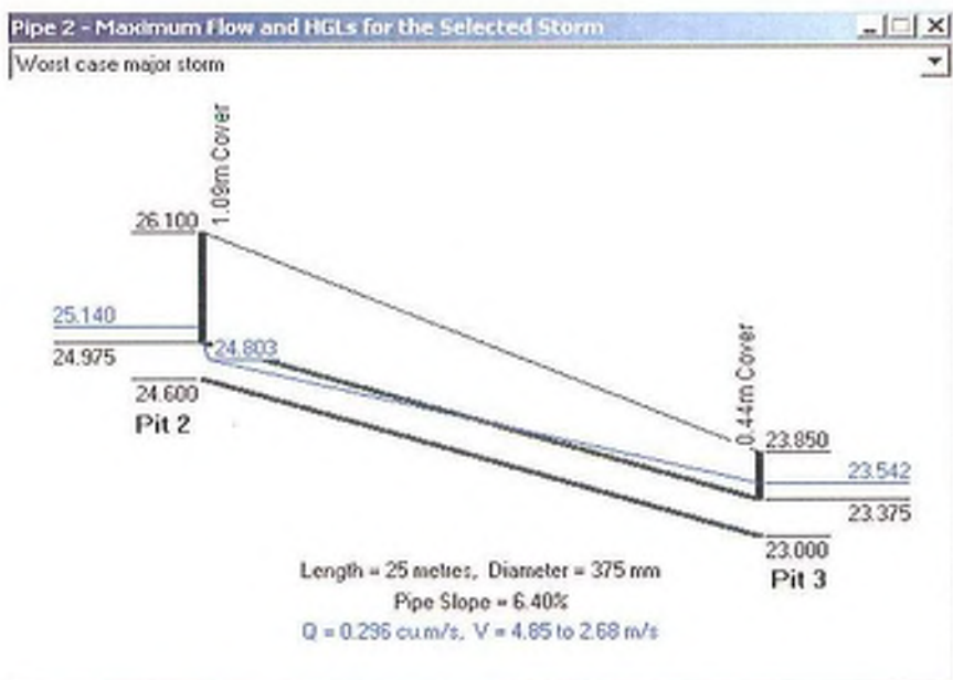
Figure 3: Hydraulic Grade Line in Pipe 2
