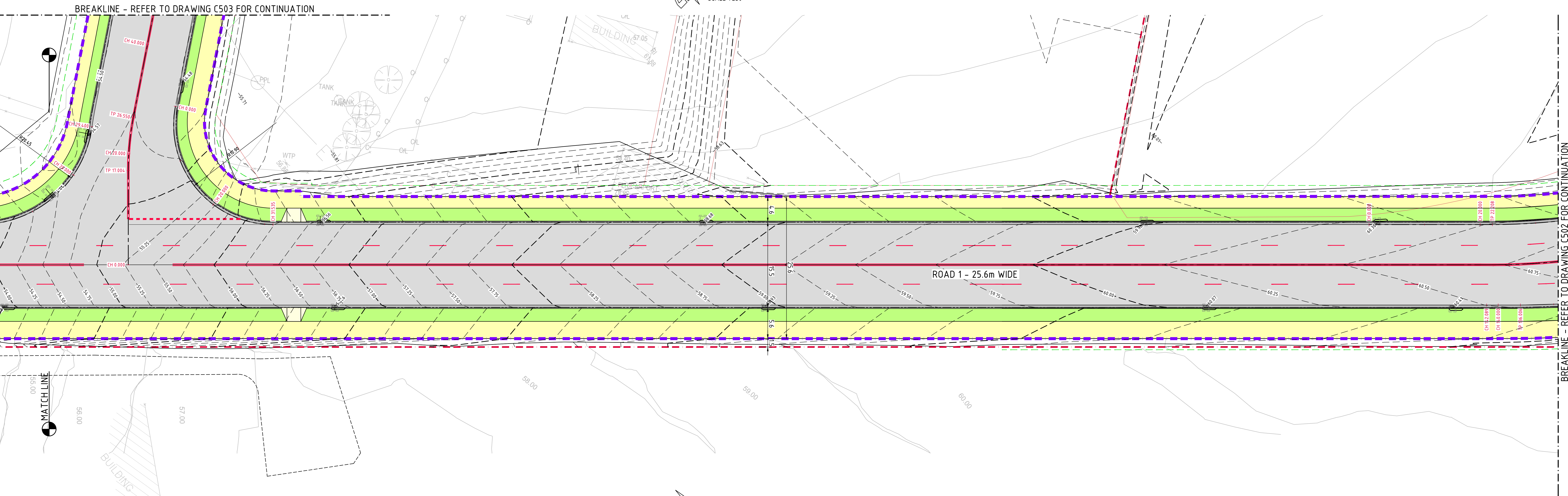
ROADWORKS PLAN - SEGMENT 2 SCALE 1:250
