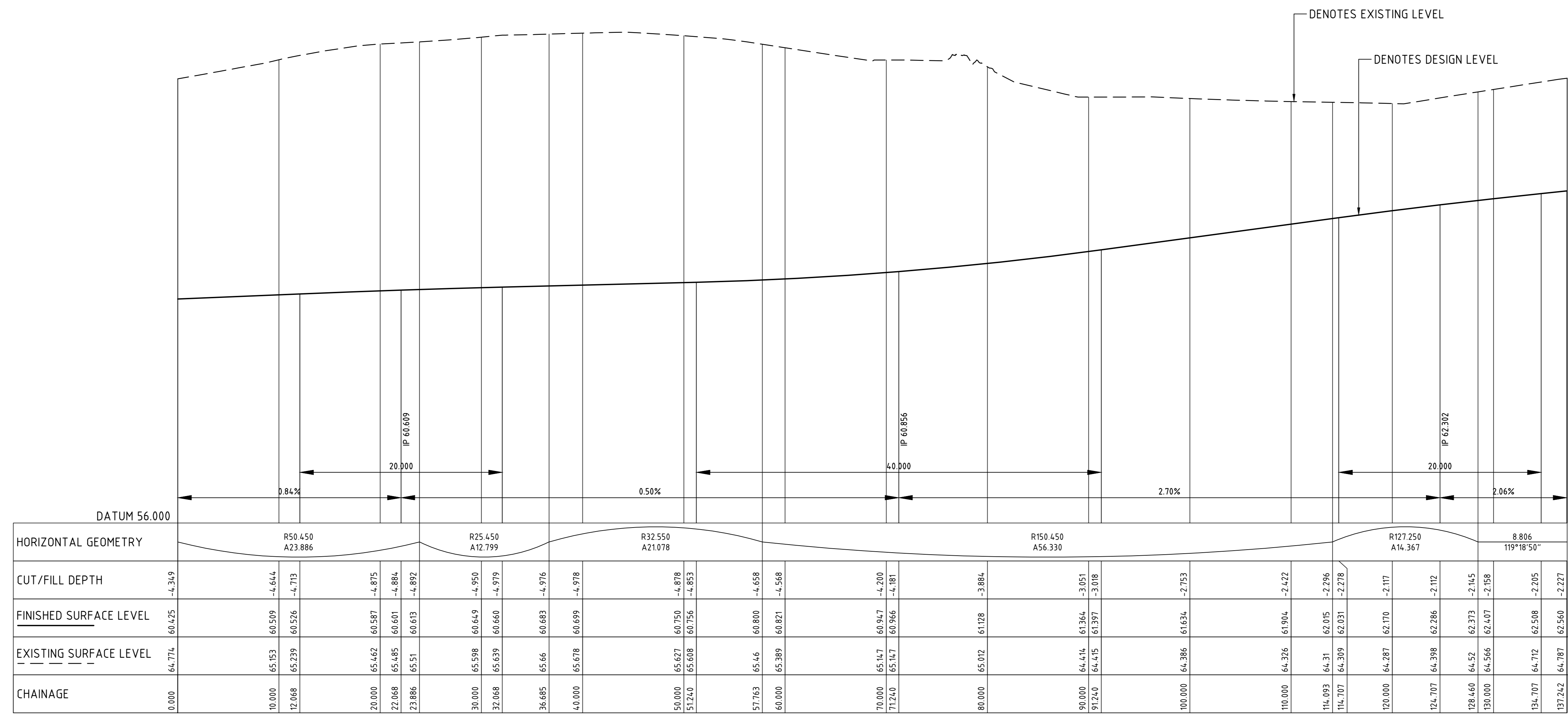
LONGITUDINAL SECTION - KR01 HORIZONTAL SCALE 1:250 VERTICAL SCALE 1:50
