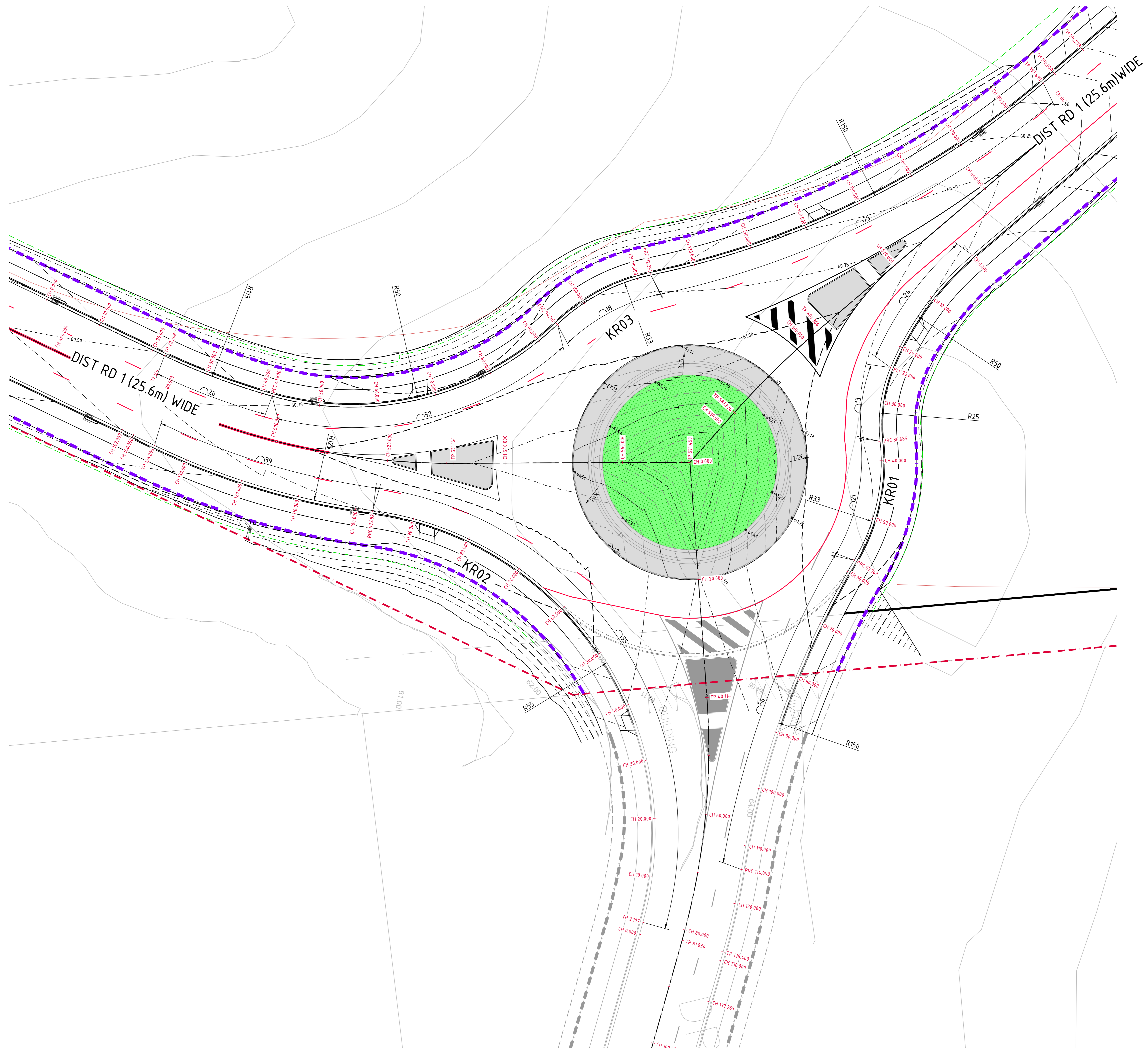
ROAD 1 & 3 ROUNDABOUT PLAN SCALE 1:250
