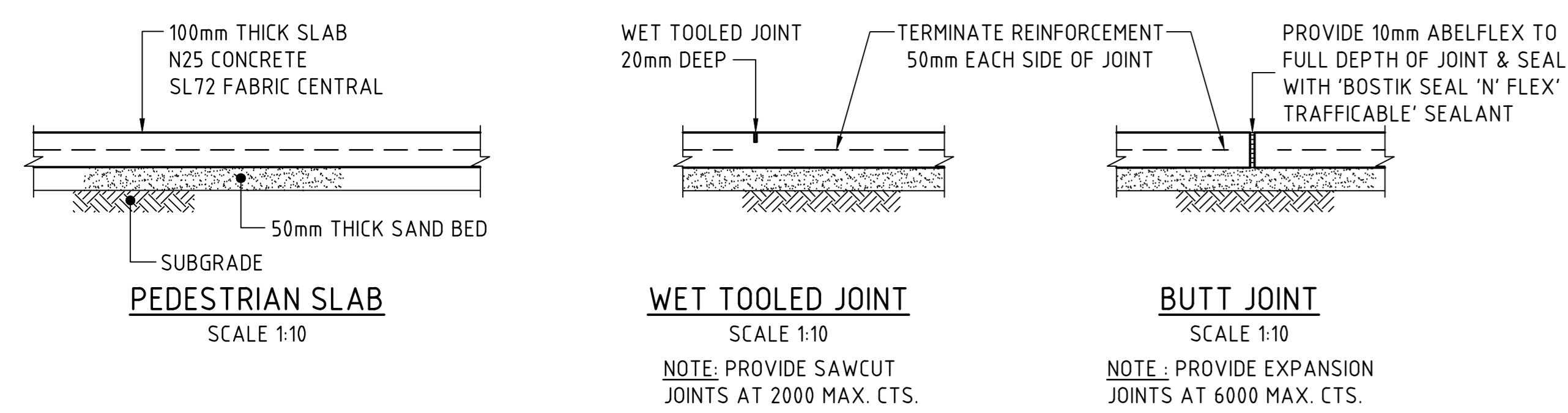
PEDESTRIAN SLAB DETAILS
