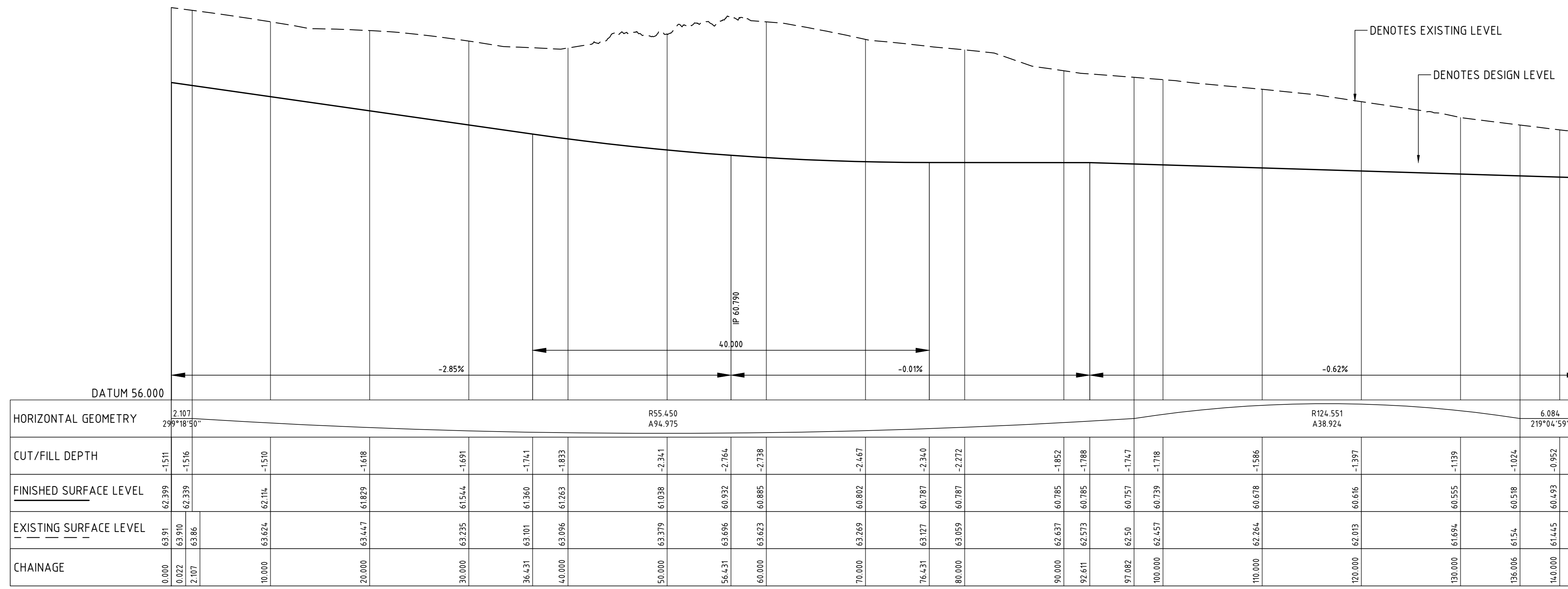
LONGITUDINAL SECTION - KR02 HORIZONTAL SCALE 1:250 VERTICAL SCALE 1:50
