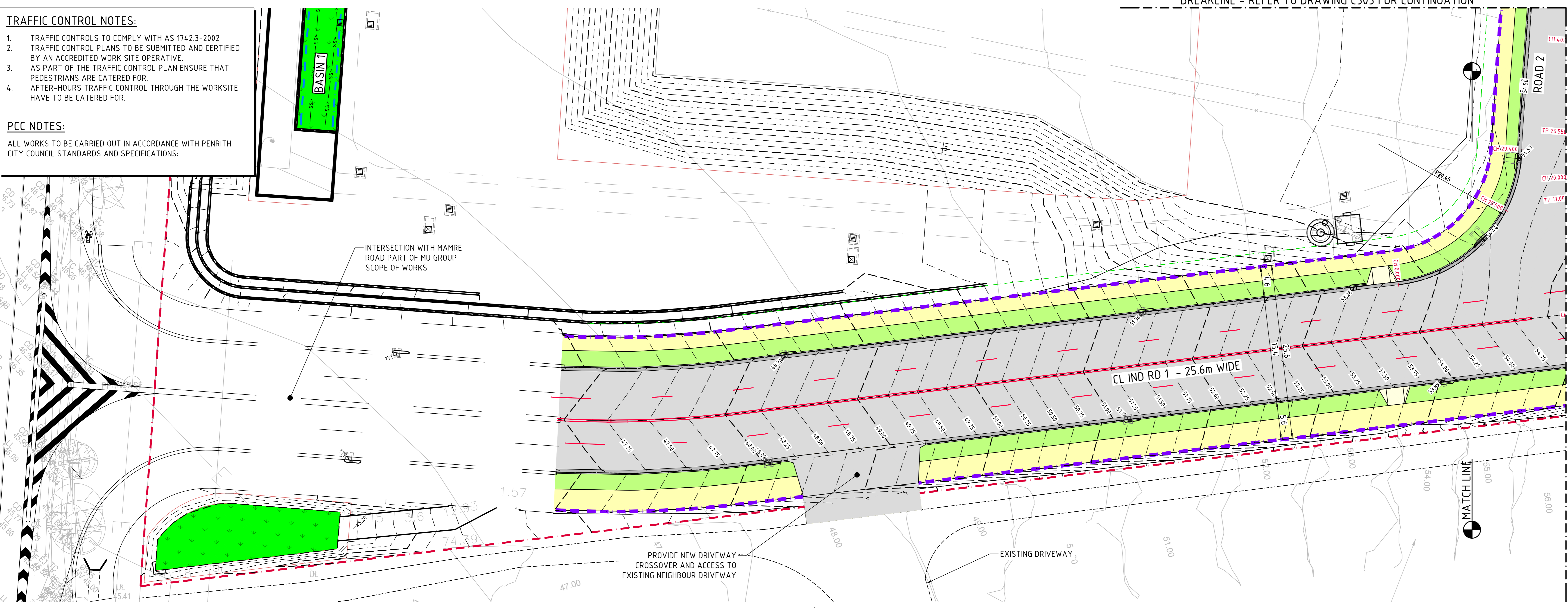
ROADWORKS PLAN - SEGMENT 1 SCALE 1:250
