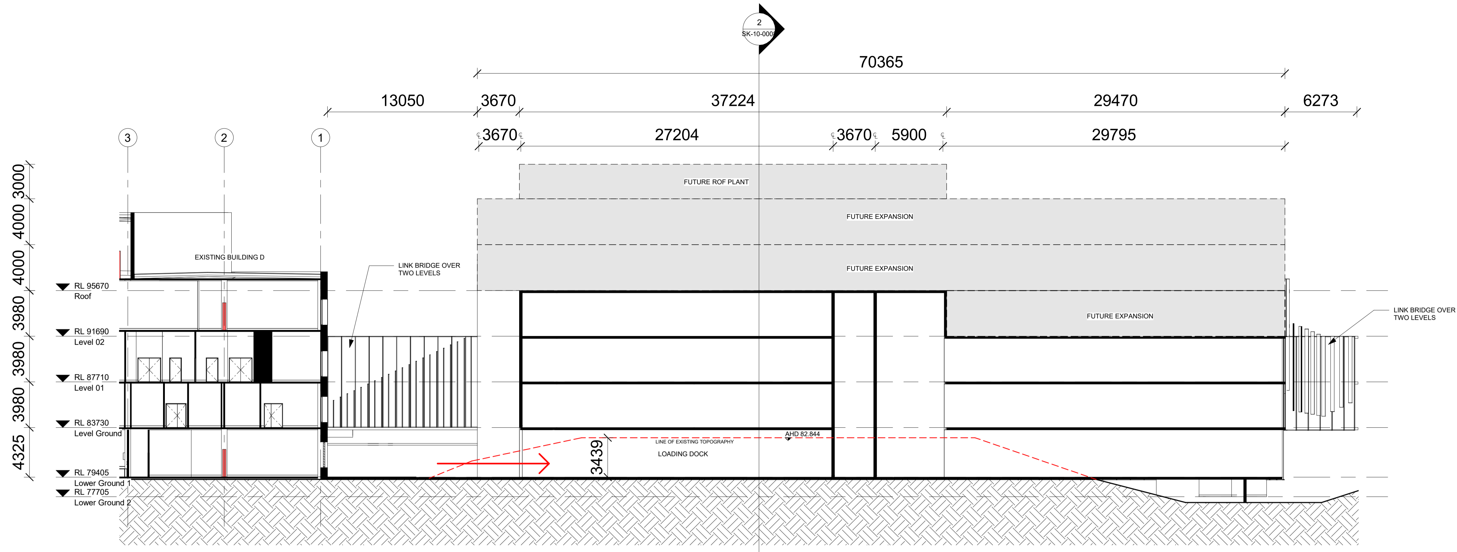
1 Section 1 1:200
