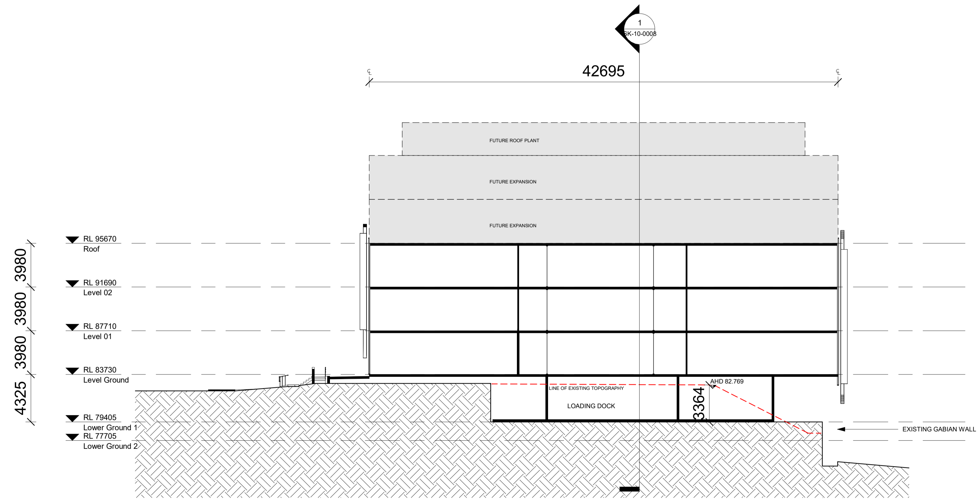
2 Section 2 1:200
