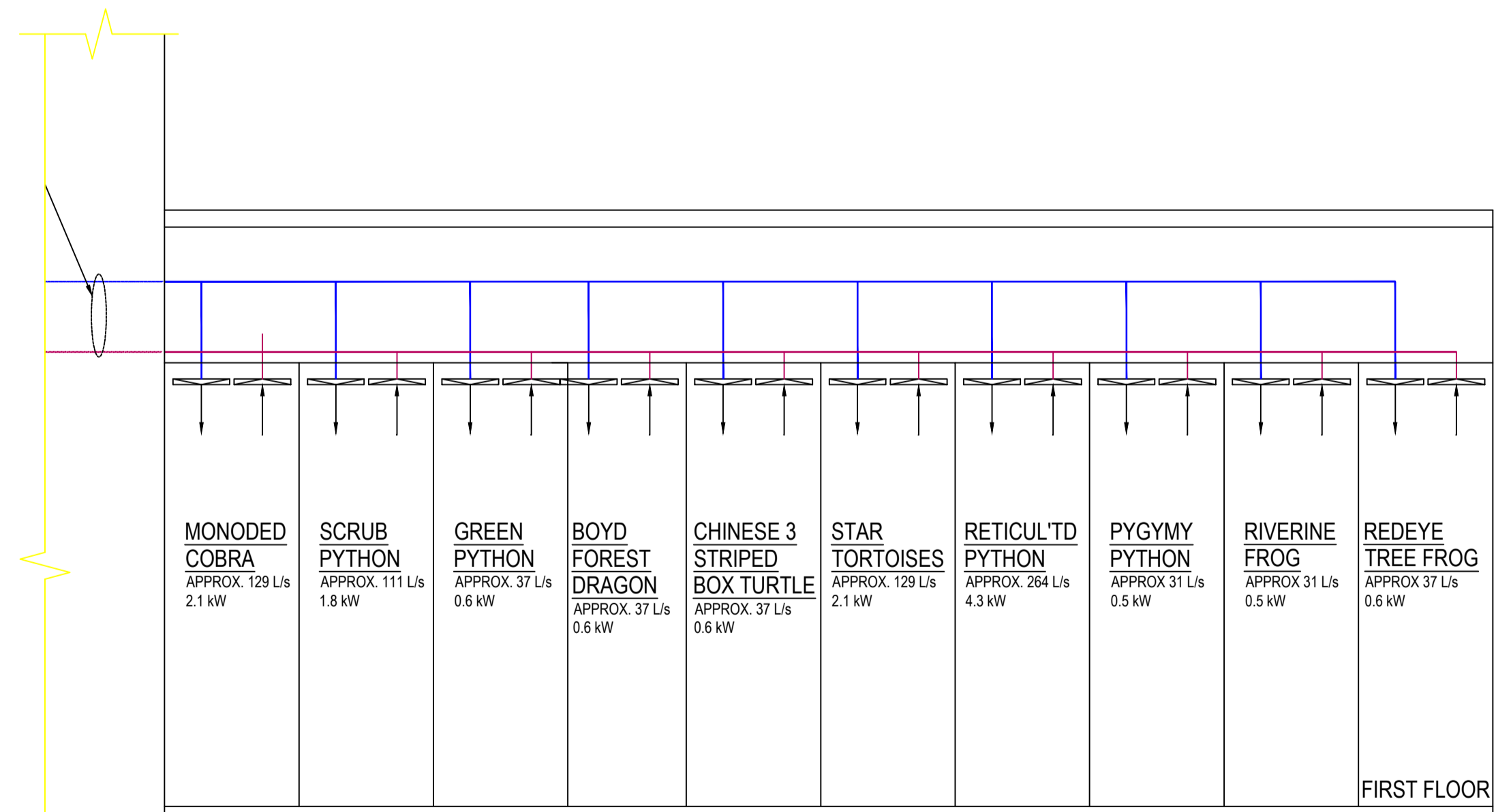
FF HVAC SCHEMATIC
