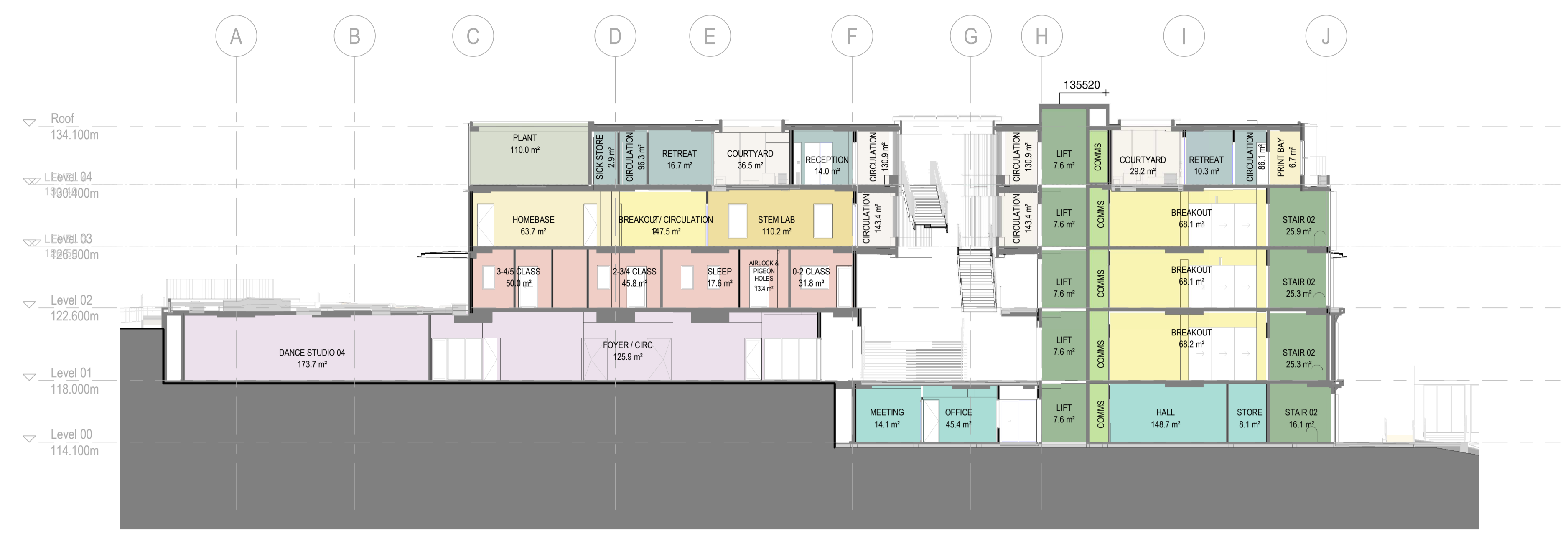
1 EAST / WEST SECTION 3 SSDA 1 : 200
