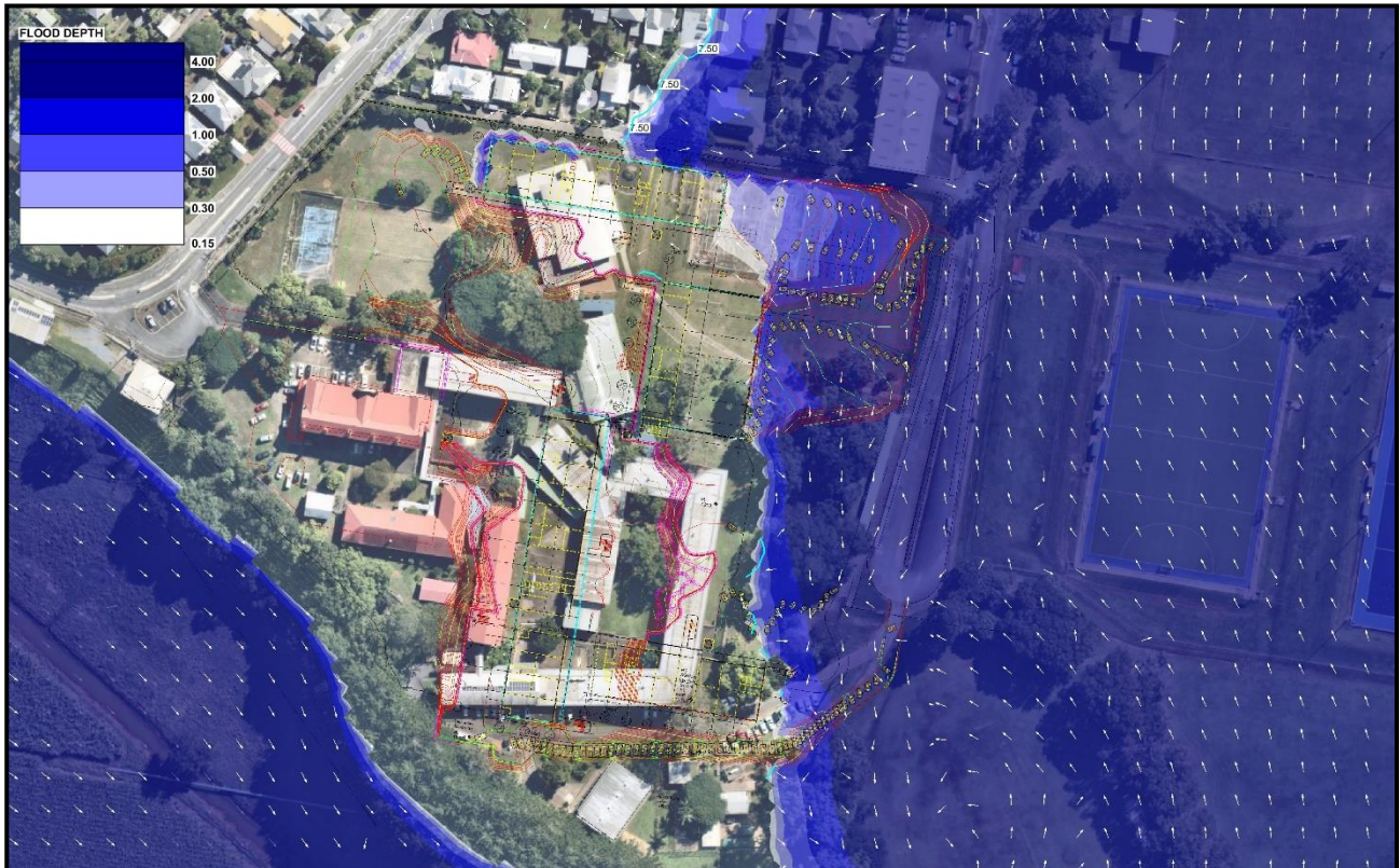
Figure 14 – 0.2% AEP Post Development Flood Levels and Depths
