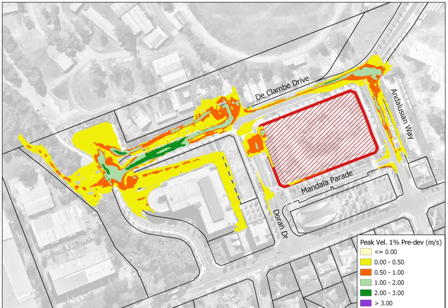
Figure 4.8 – Existing Scenario 1% AEP Flood Velocity
