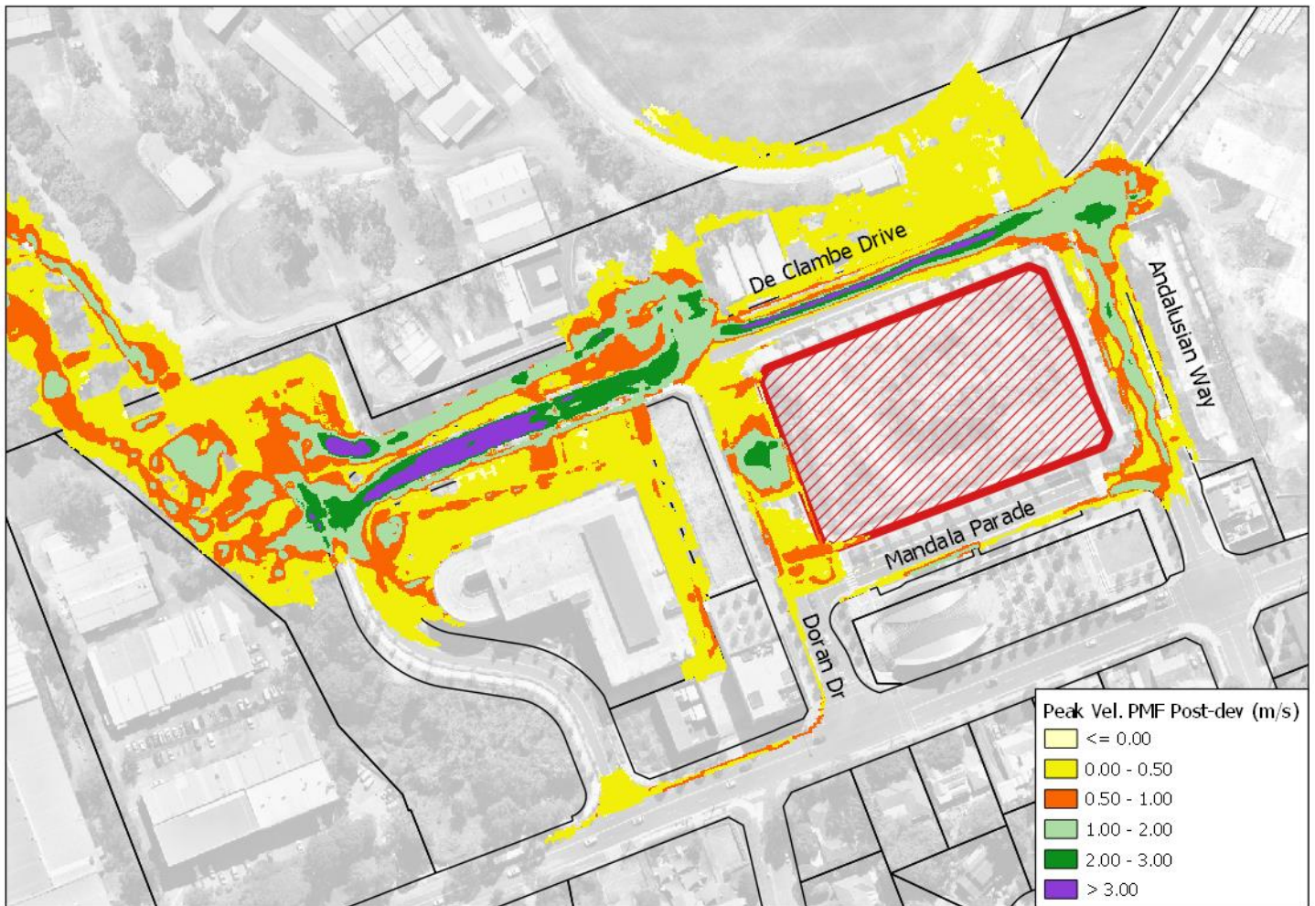
Figure 4.25 – Developed Scenario PMF Flood Velocity
