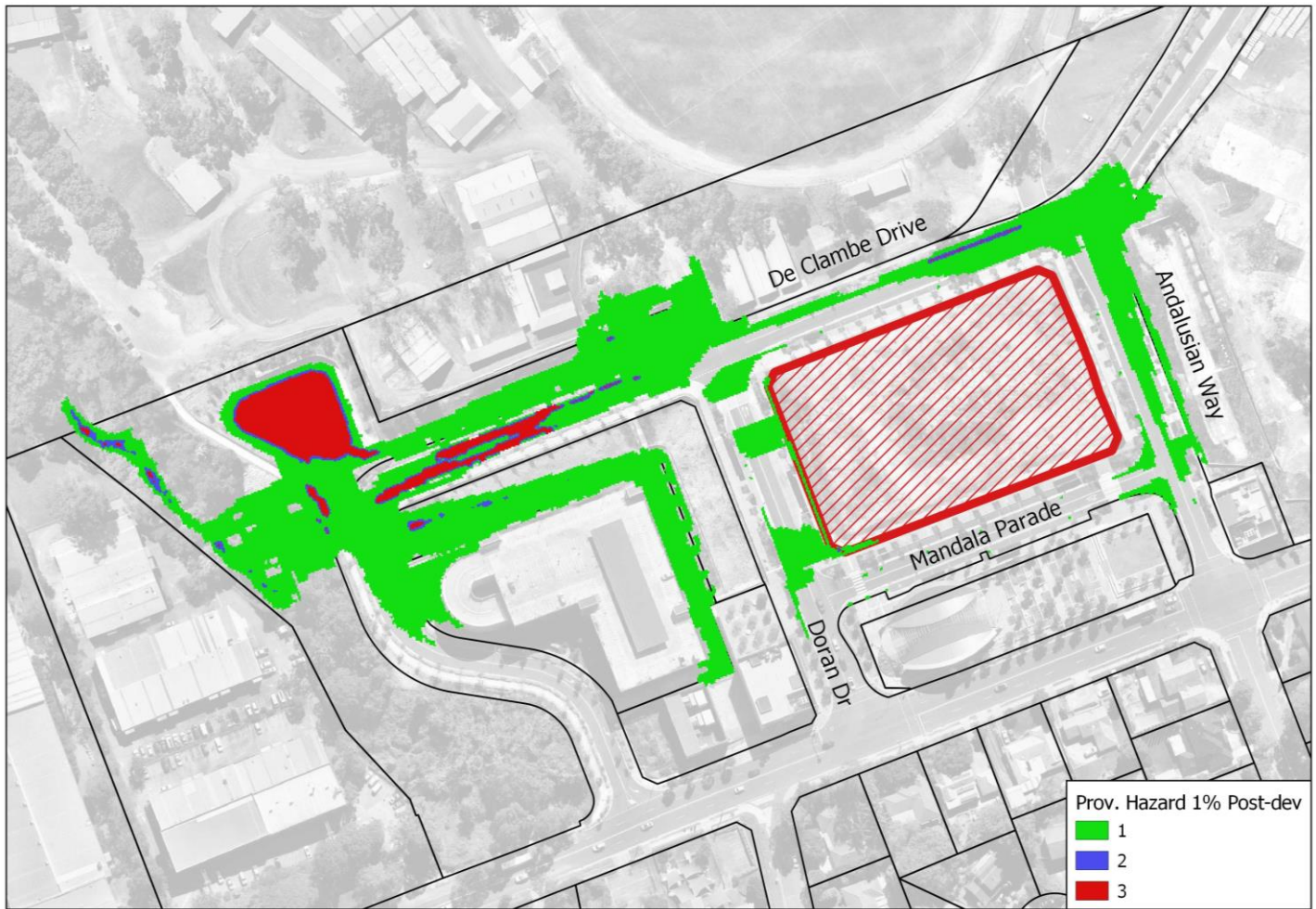
Figure 4.22 – Developed Scenario 1% AEP Flood Hazard (1 = Low 2 = Medium 3 = High)
