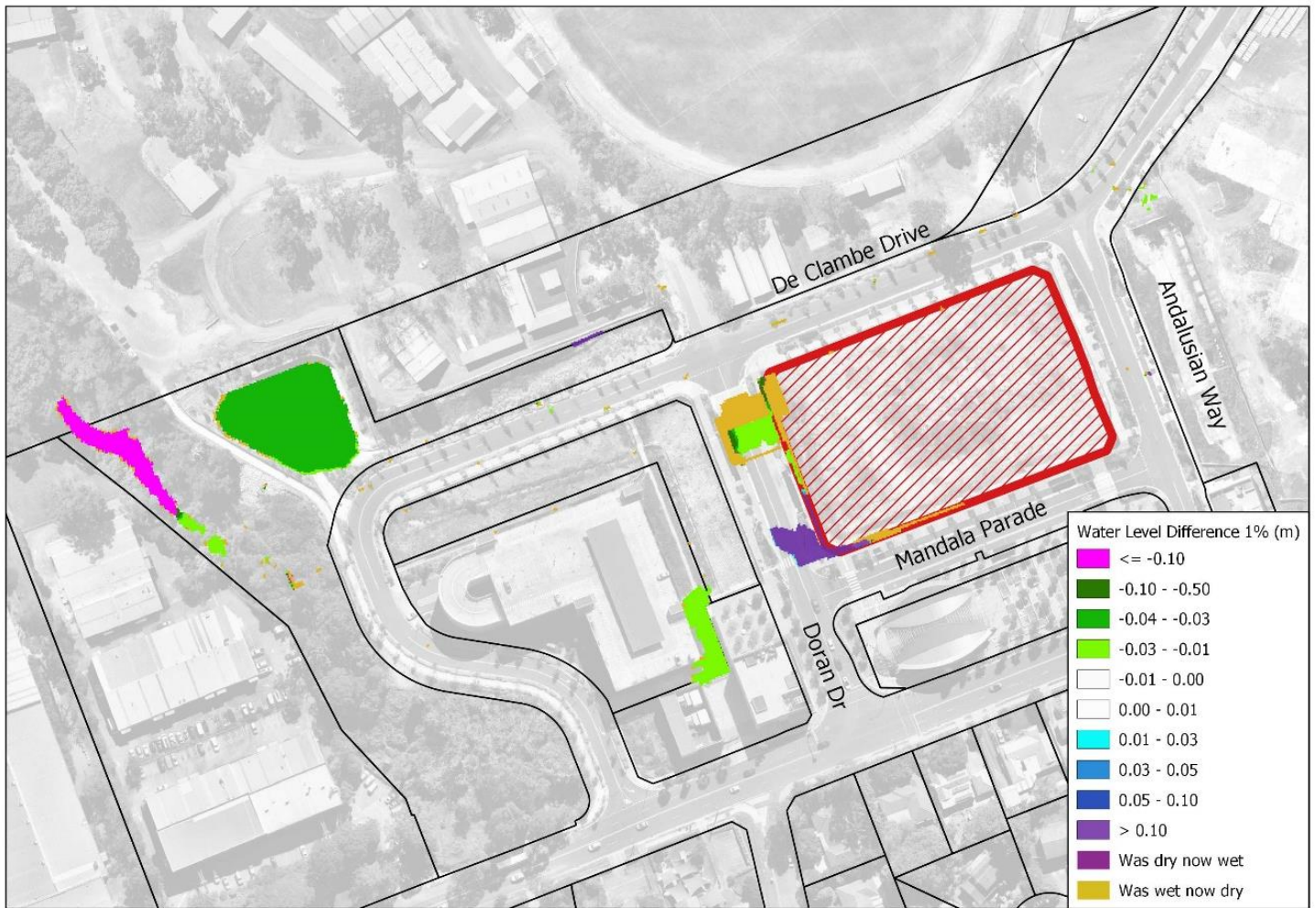
Figure 4.30 – Flood Level Difference – 1% AEP
