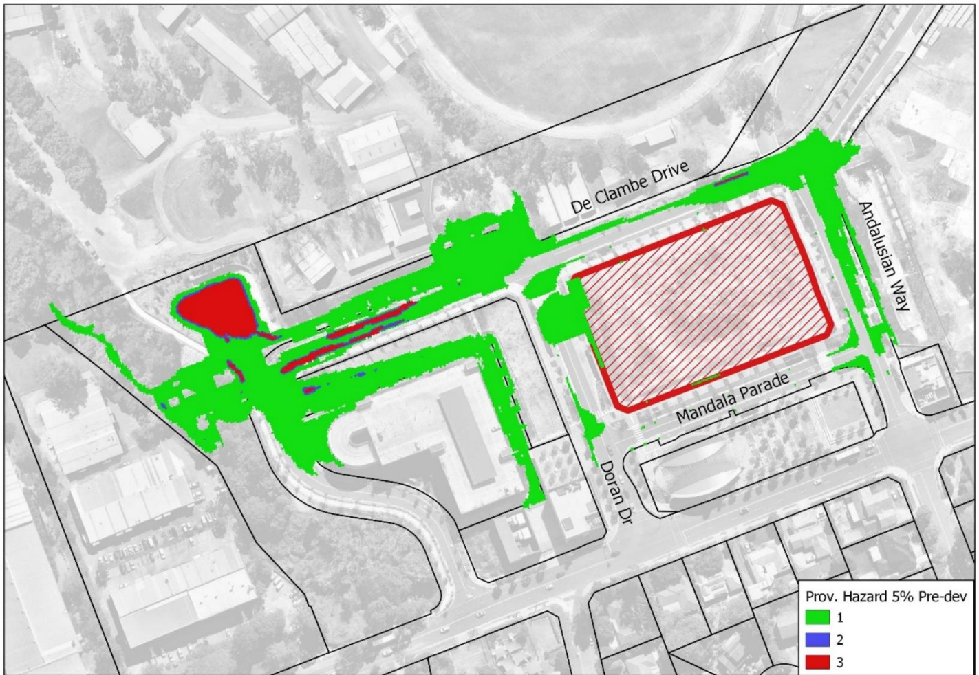
Figure 4.5 – Existing Scenario 5% AEP Flood Hazard (1 = Low 2 = Medium 3 = High)
