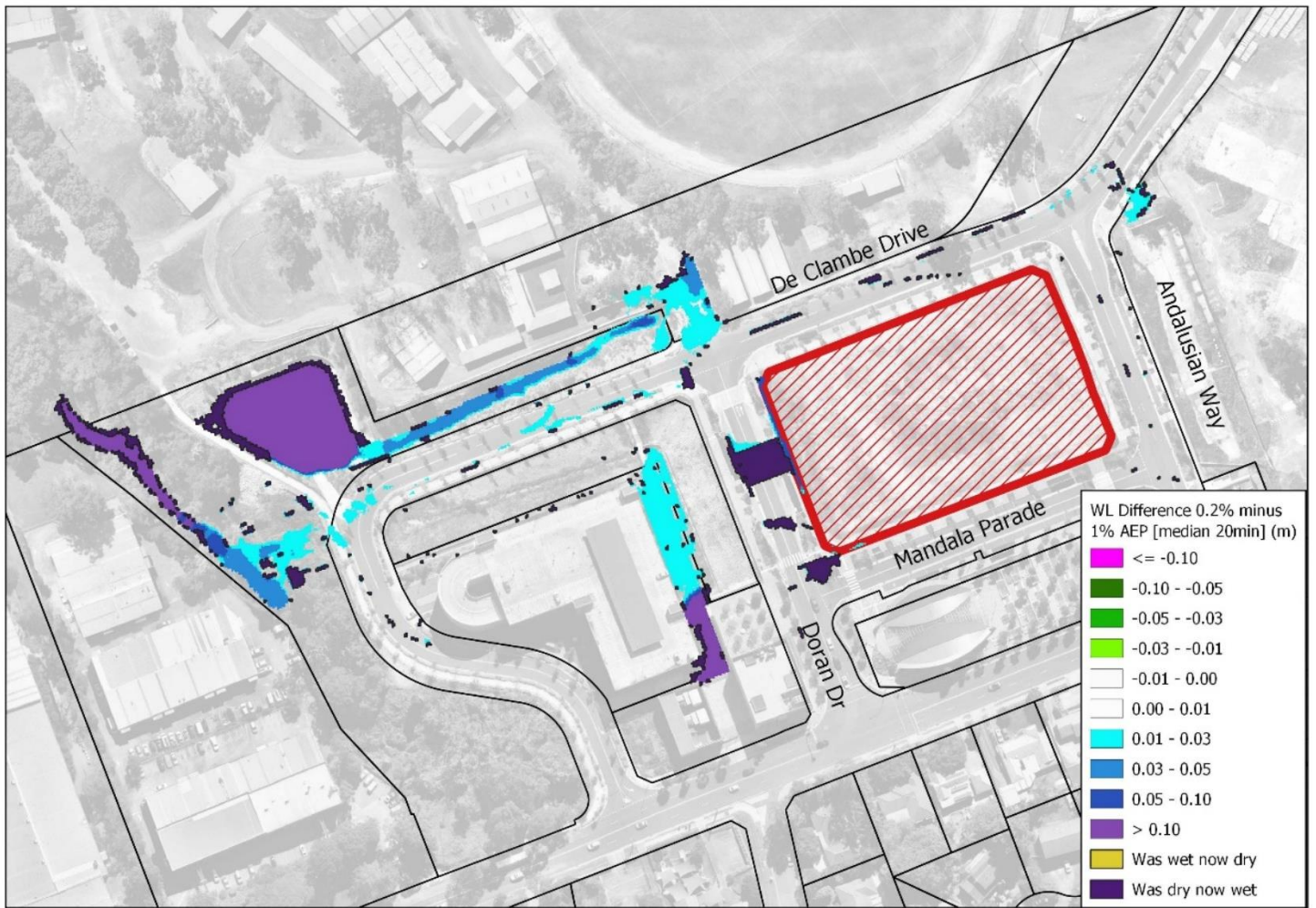
Figure 5.12 – Flood Level Difference – 0.2% AEP
