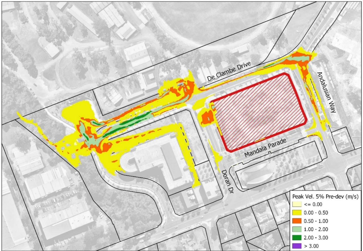
Figure 4.4 – Existing Scenario 5% AEP Flood Velocity
