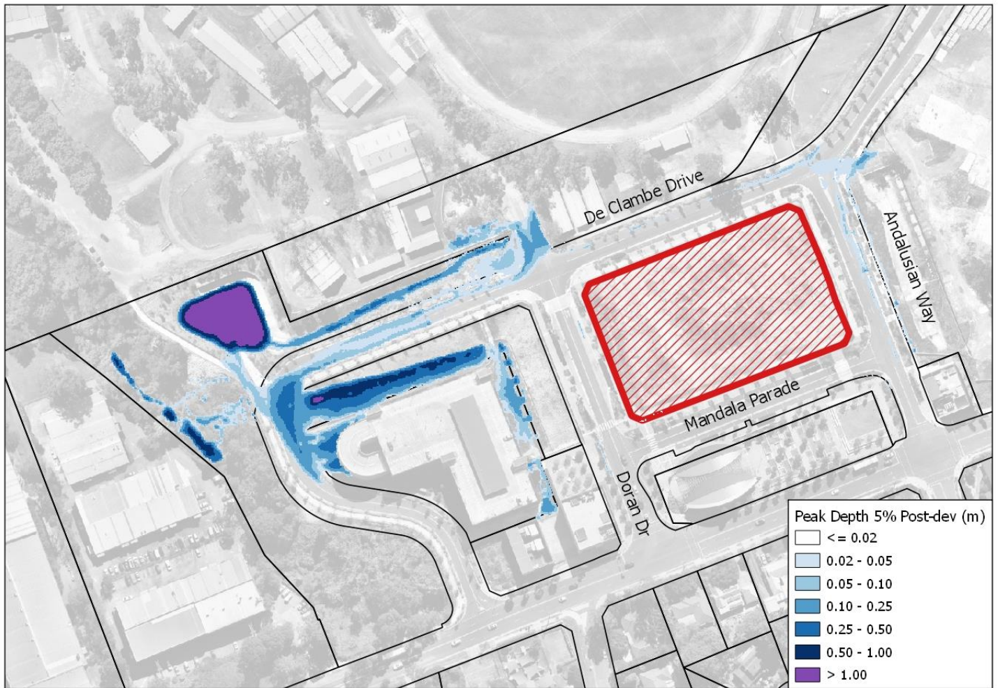
Figure 4.16 – Developed Scenario 5% AEP Flood Depth
