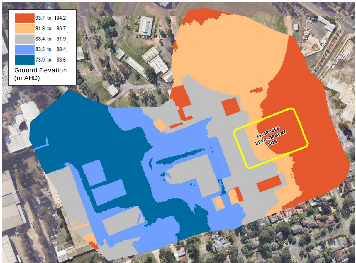
Figure 3.2 – TUFLOW Model Grid
