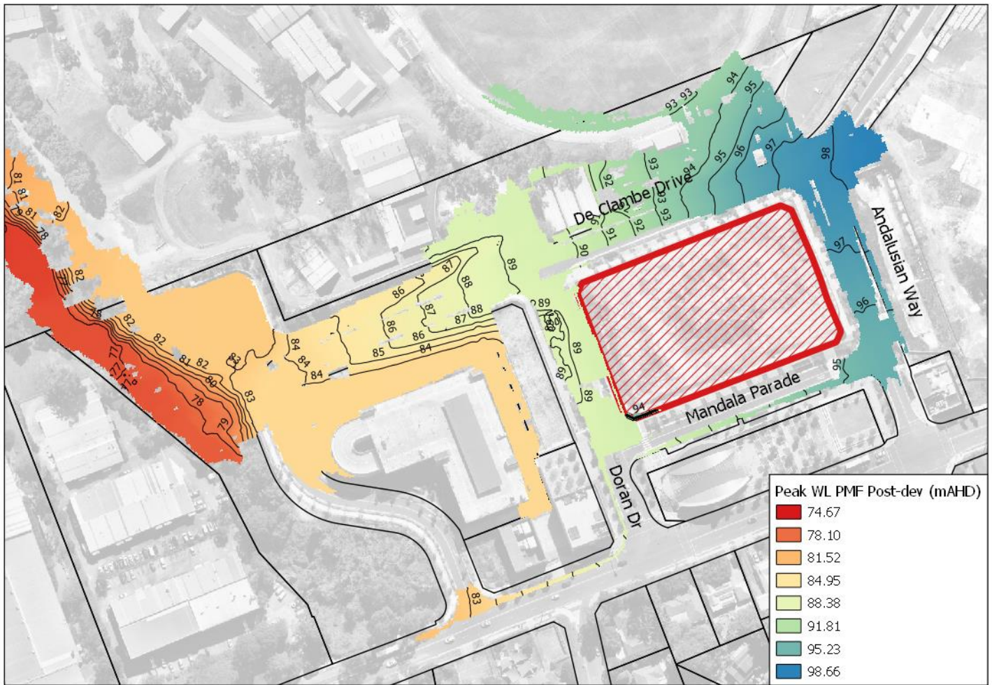
Figure 4.23 – Developed Scenario PMF Flood Level
