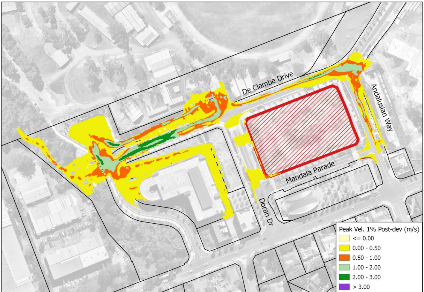
Figure 4.21 – Developed Scenario 1% AEP Flood Velocity
