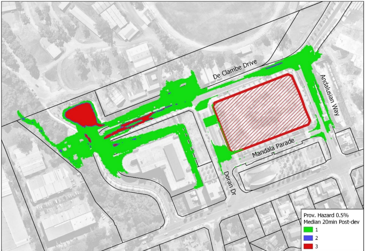
Figure 5.4 – Developed Scenario 0.5% AEP Flood Hazard
