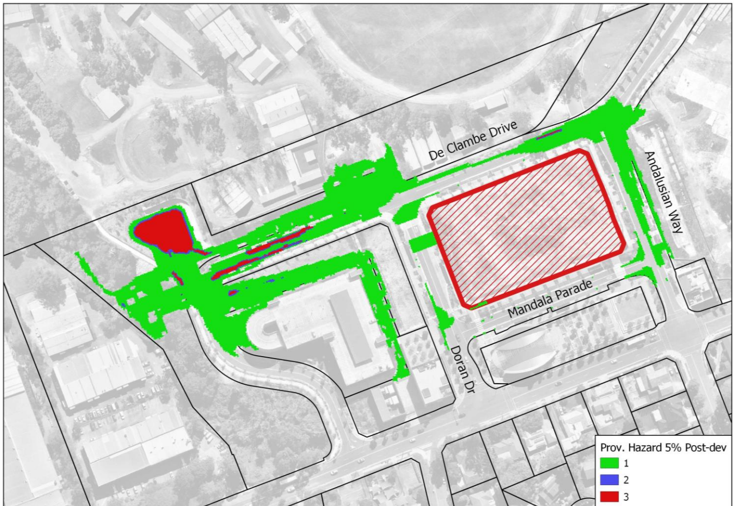
Figure 4.18 – Developed Scenario 5% AEP Flood Hazard (1 = Low 2 = Medium 3 = High)
