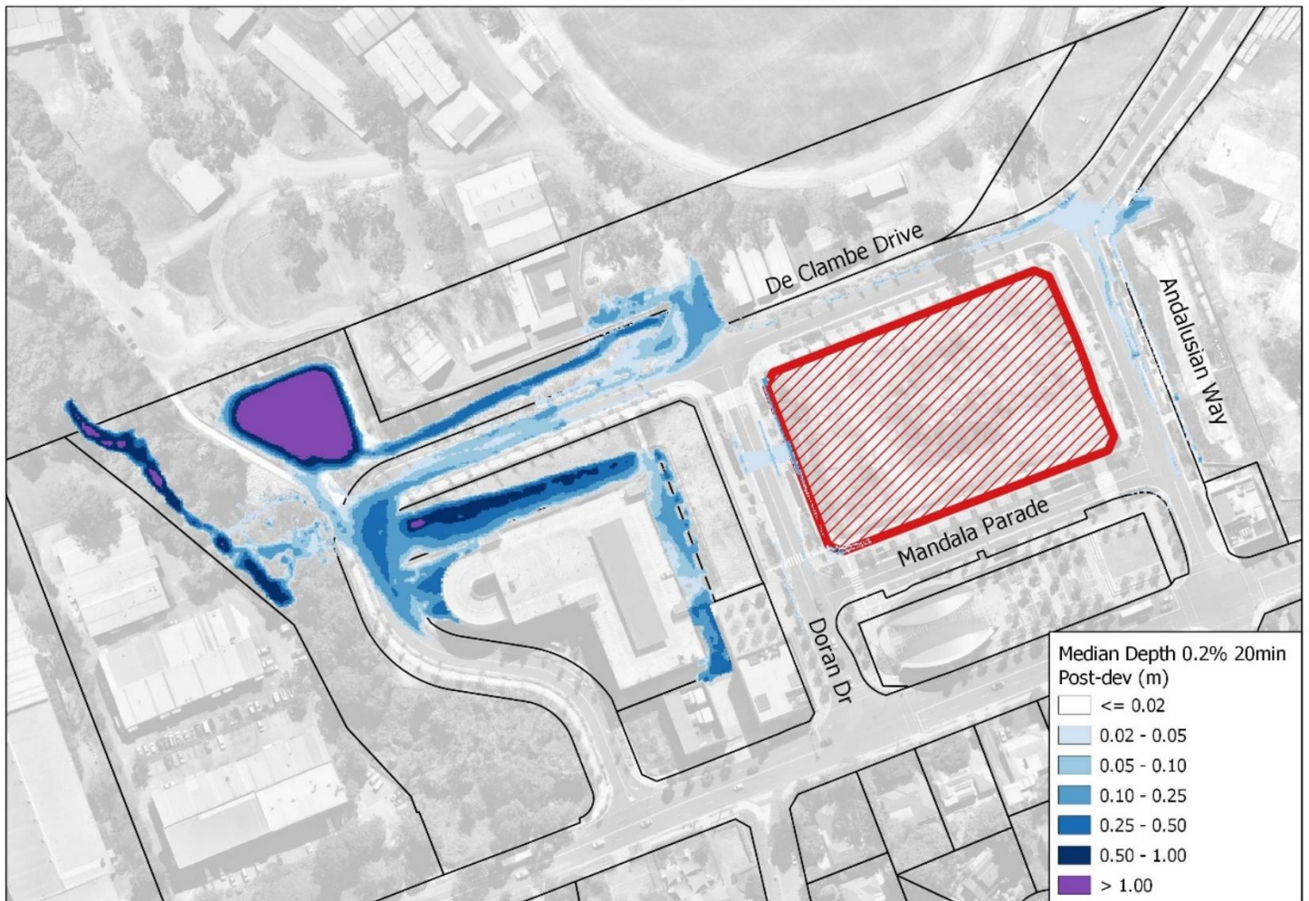
Figure 5.6 – Developed Scenario 0.2% AEP Flood Depth
