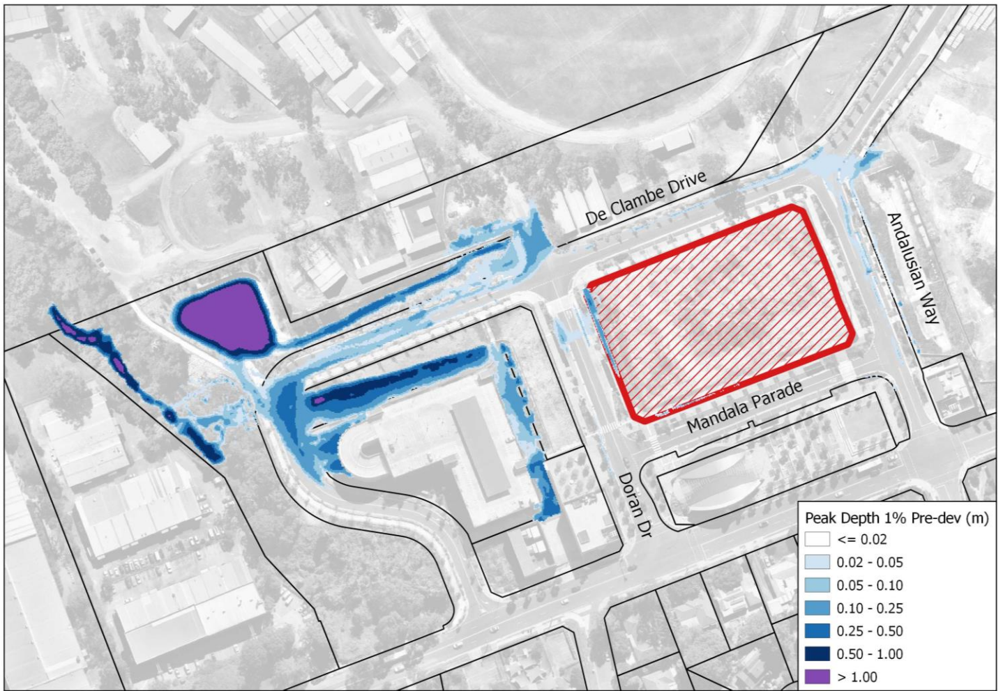
Figure 4.7 – Existing Scenario 1% AEP Flood Depth
