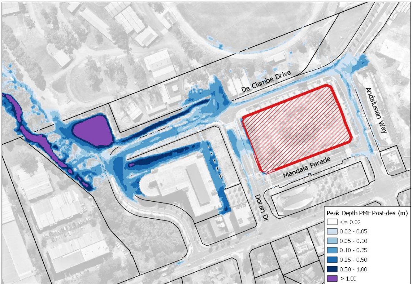
Figure 4.24 – Developed Scenario PMF Flood Depth
