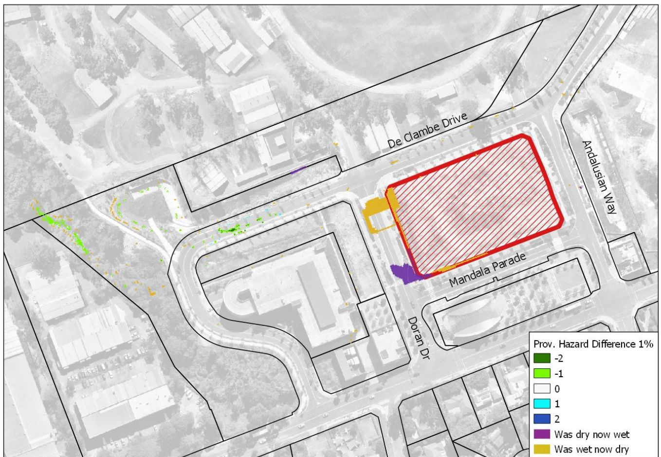
Figure 4.32 – Flood Hazard Difference – 1% AEP
