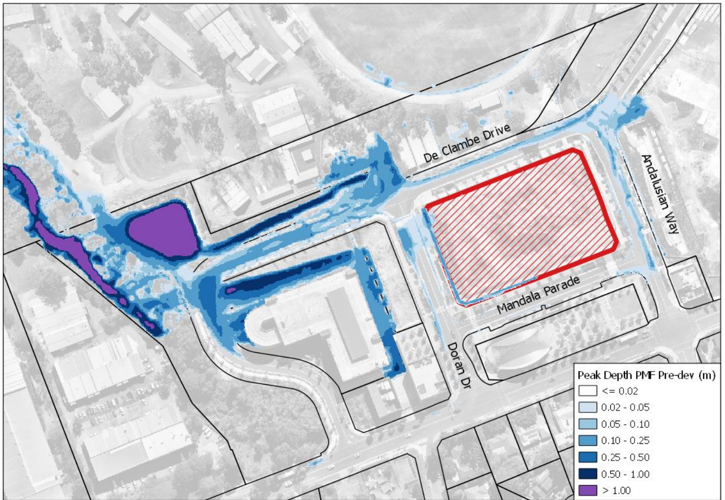
Figure 4.11 – Existing Scenario PMF Flood Depth
