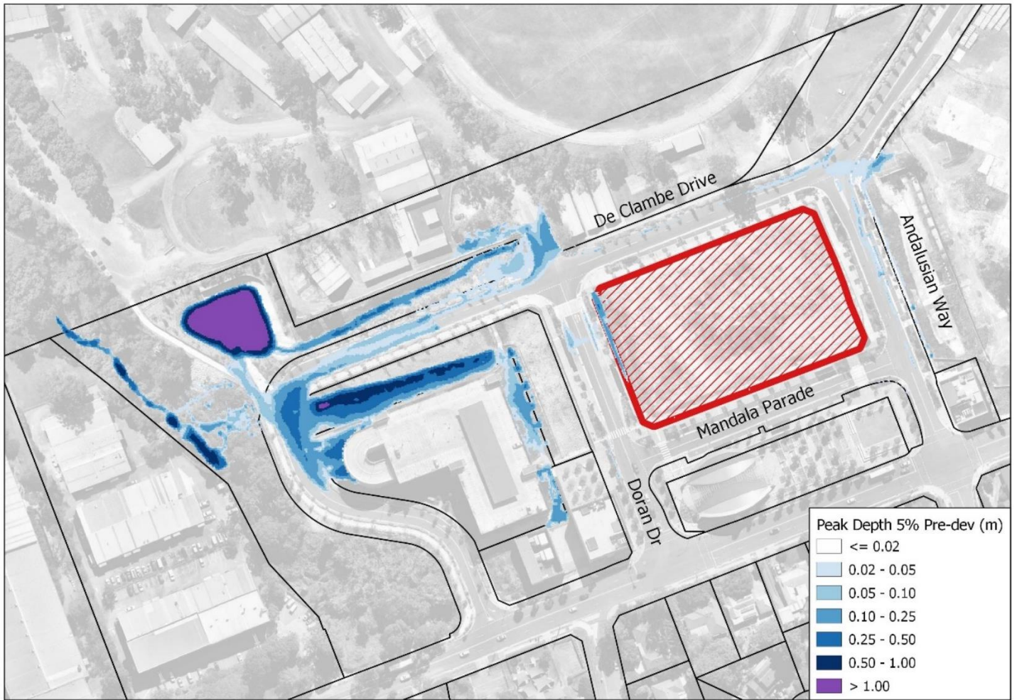
Figure 4.3 – Existing Scenario 5% AEP Flood Depth
