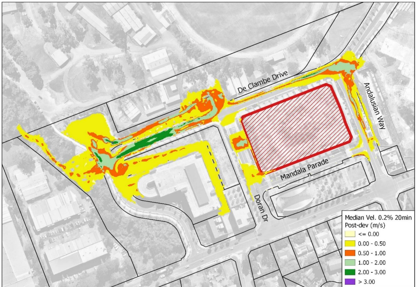
Figure 5.7 – Developed Scenario 0.2% AEP Flood Velocity
