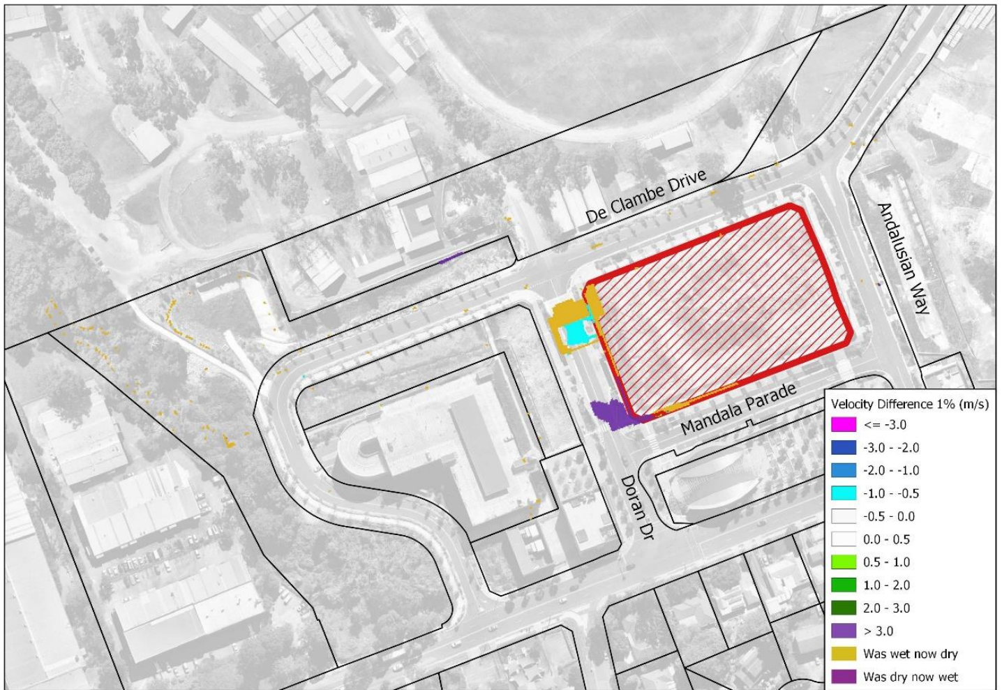
Figure 4.31 – Flood Velocity Difference – 1% AEP
