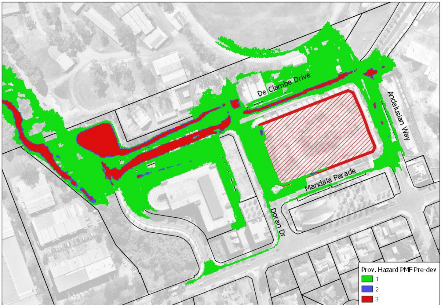
Figure 4.13 – Existing Scenario PMF Flood Hazard (1 = Low 2 = Medium 3 = High)
