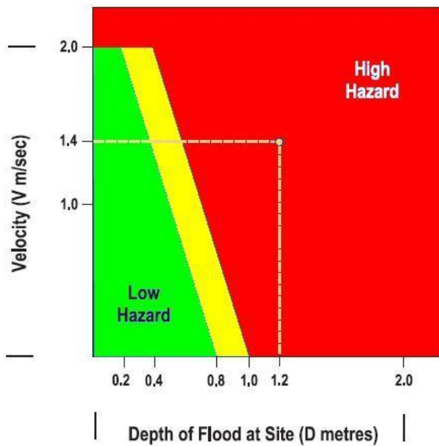
Figure 4.1 – Provisional Hydraulic Hazard Categories (Figure L2 from NSW Floodplain development manual (2005))
