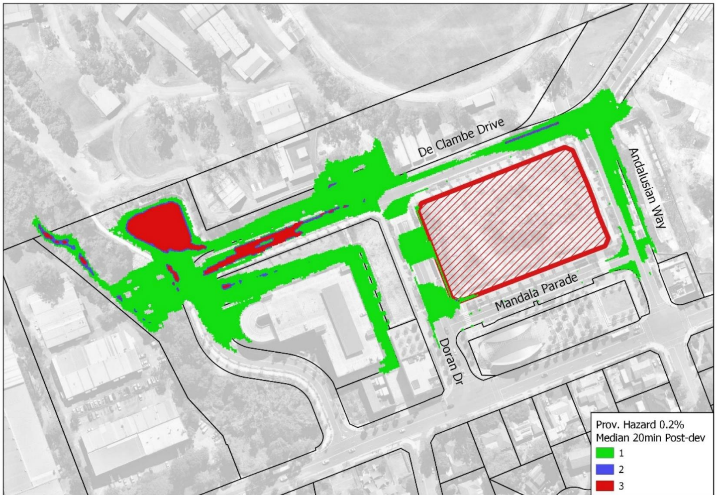
Figure 5.8 – Developed Scenario 0.5% AEP Flood Hazard
