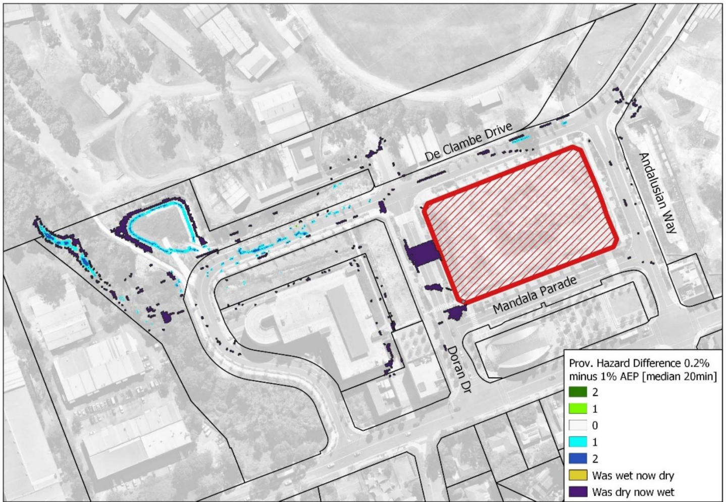
Figure 5.14 – Flood Hazard Difference – 0.2% AEP
