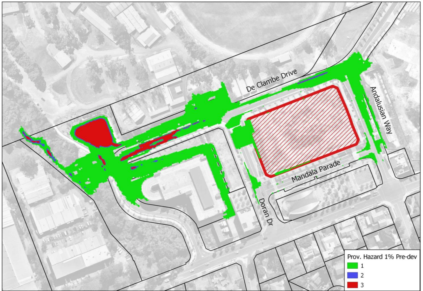
Figure 4.9 – Existing Scenario 1% AEP Flood Hazard Mapping (1 = Low 2 = Medium 3 = High)
