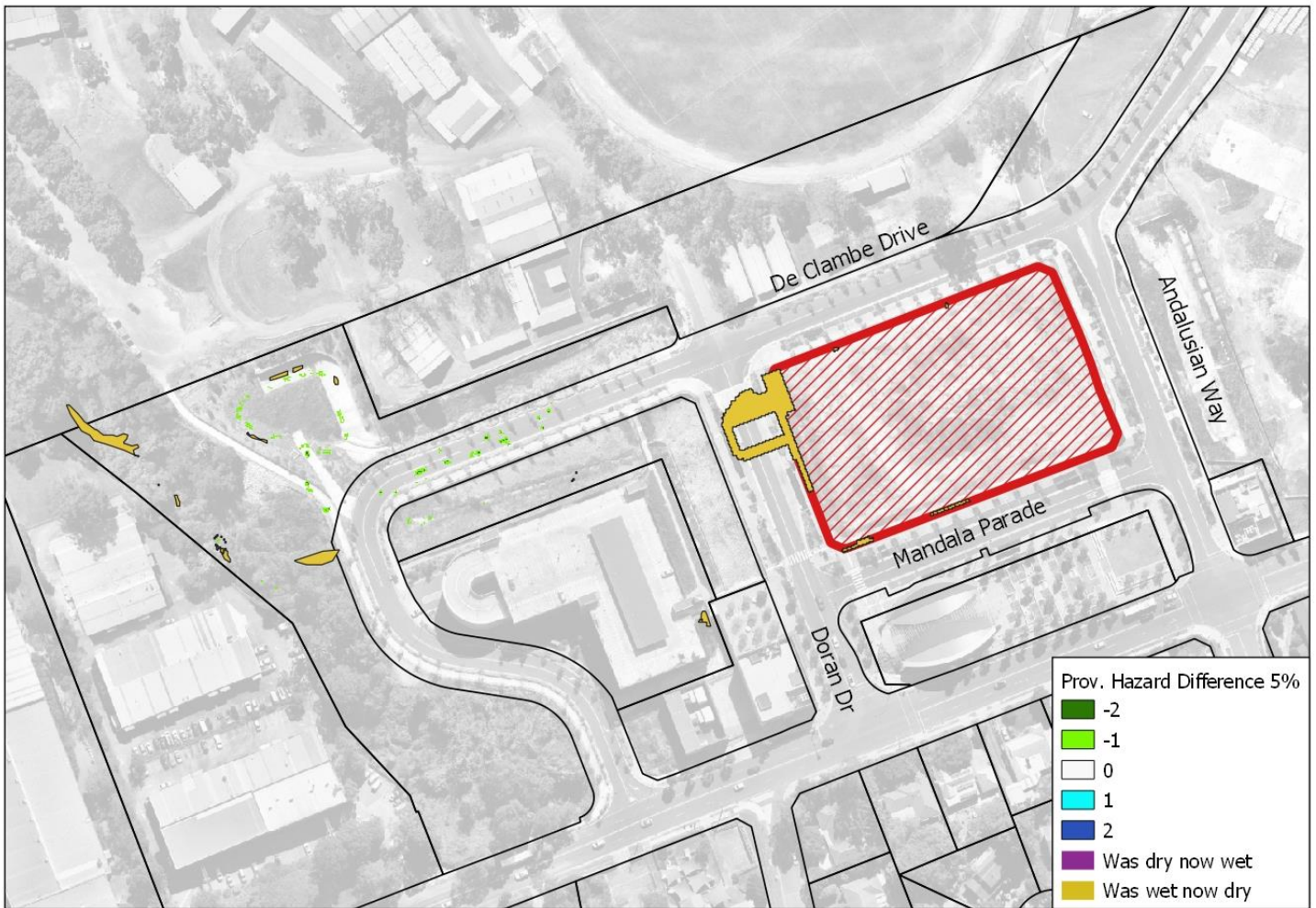
Figure 4.29 – Flood Hazard Difference – 5% AEP
