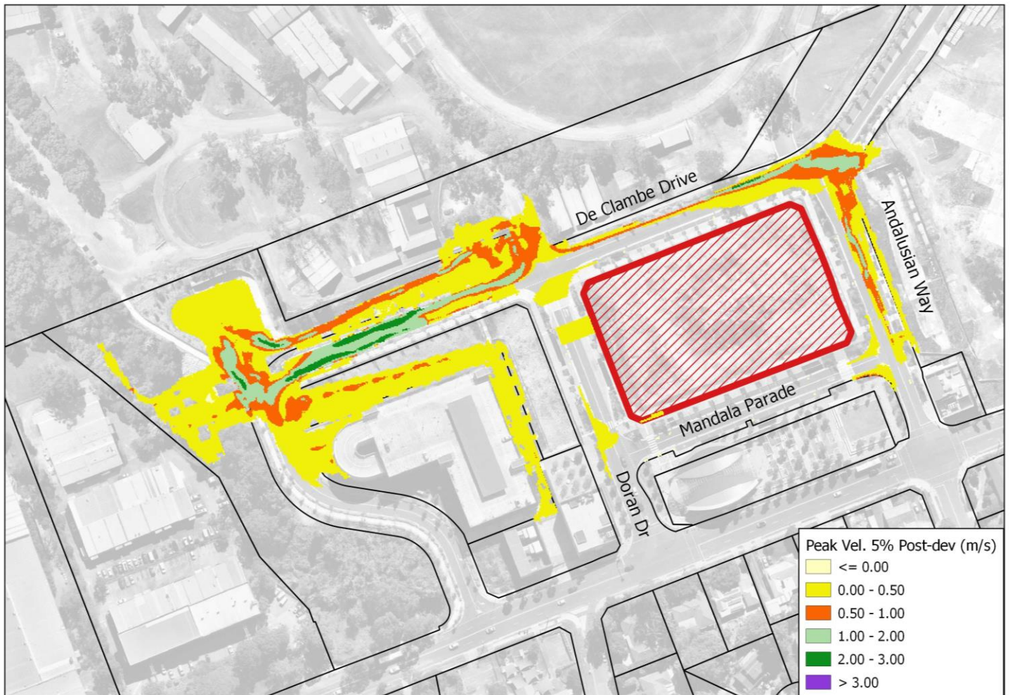
Figure 4.17 – Developed Scenario 5% AEP Flood Velocity
