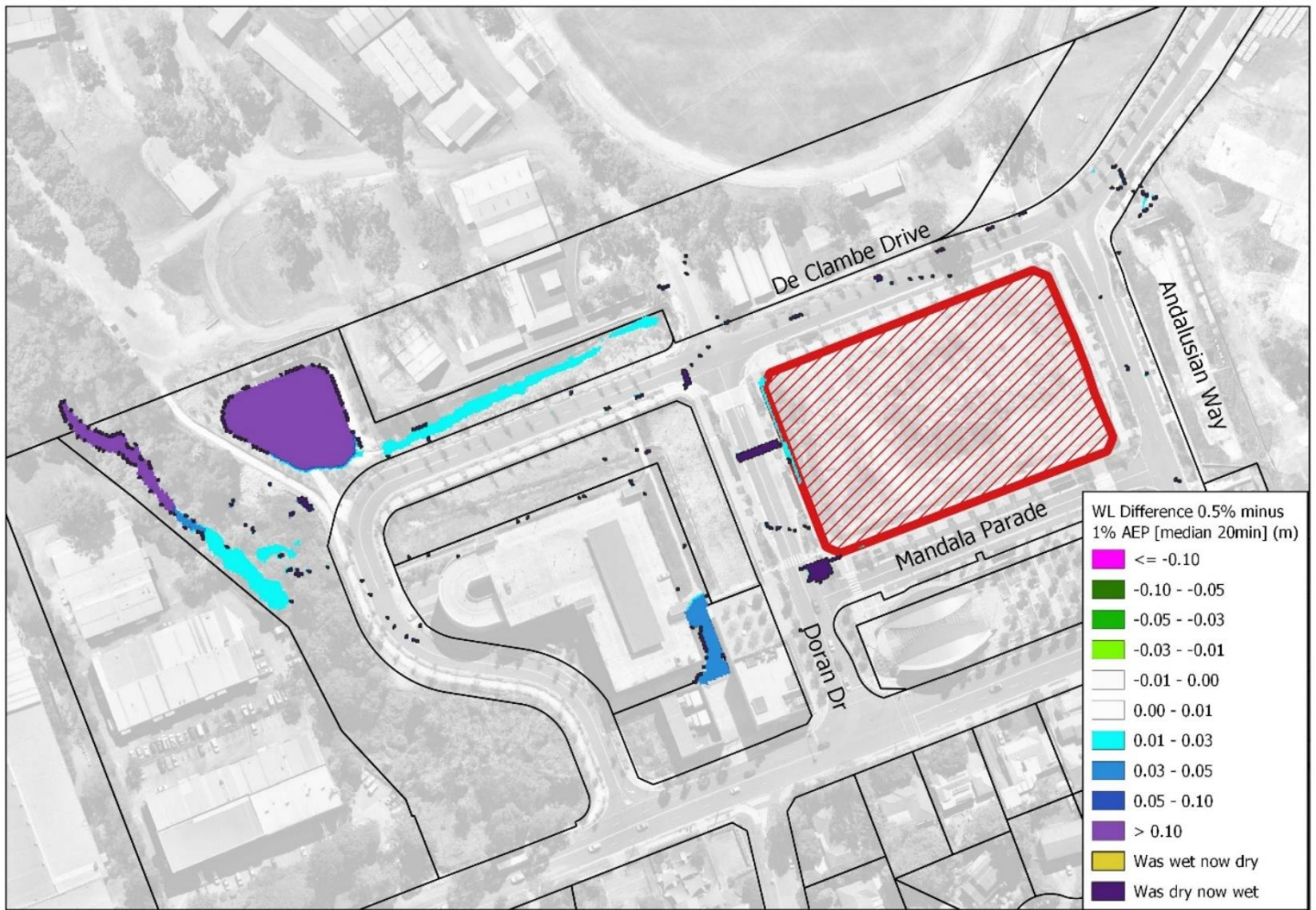
Figure 5.9 – Flood Level Difference – 0.5% AEP
