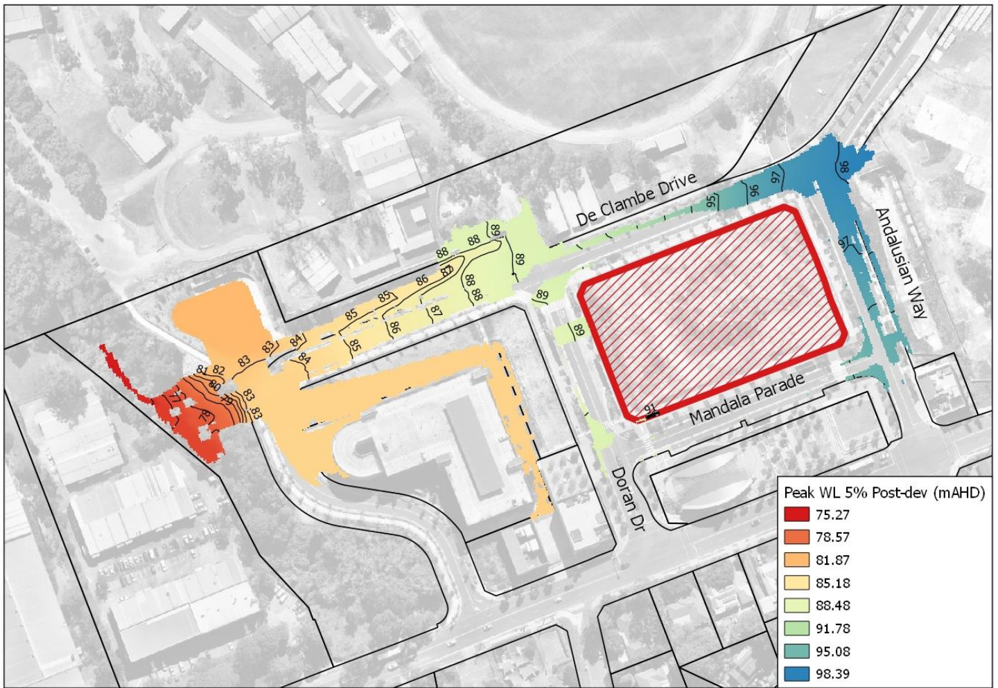
Figure 4.15 – Developed Scenario 5% AEP Flood Extent
