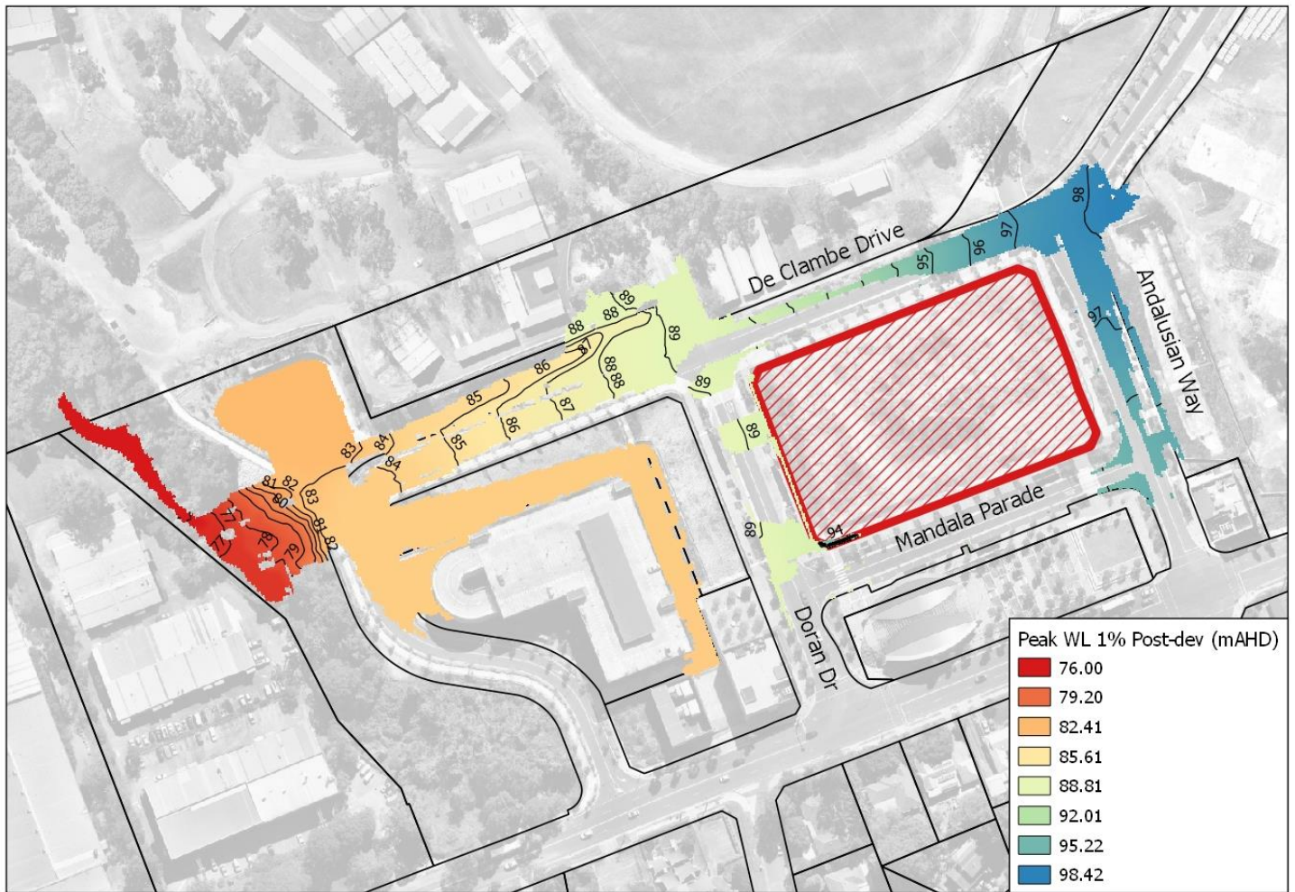
Figure 4.19 – Developed Scenario 1% AEP Flood Extent
