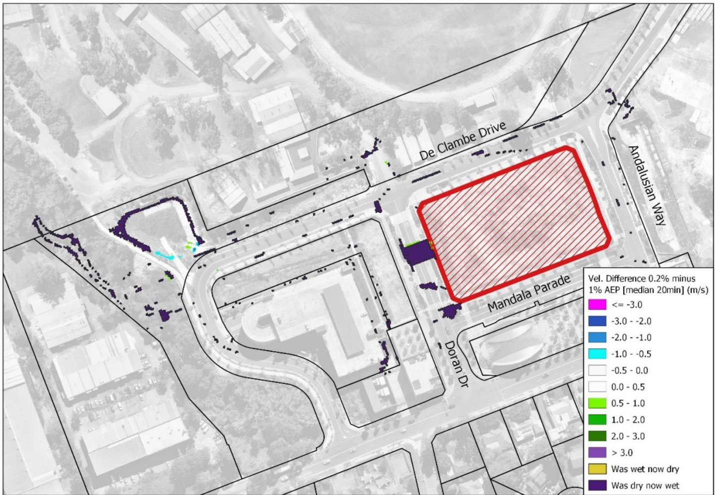
Figure 5.13 – Flood Velocity Difference – 0.2% AEP
