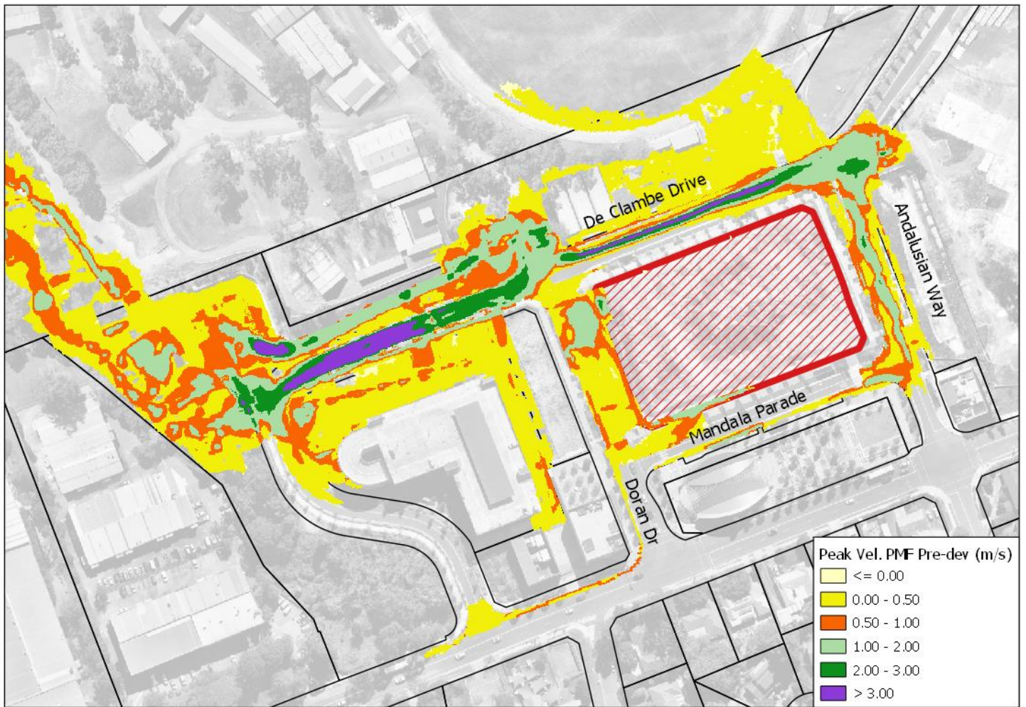
Figure 4.12 – Existing Scenario PMF Flood Velocity
