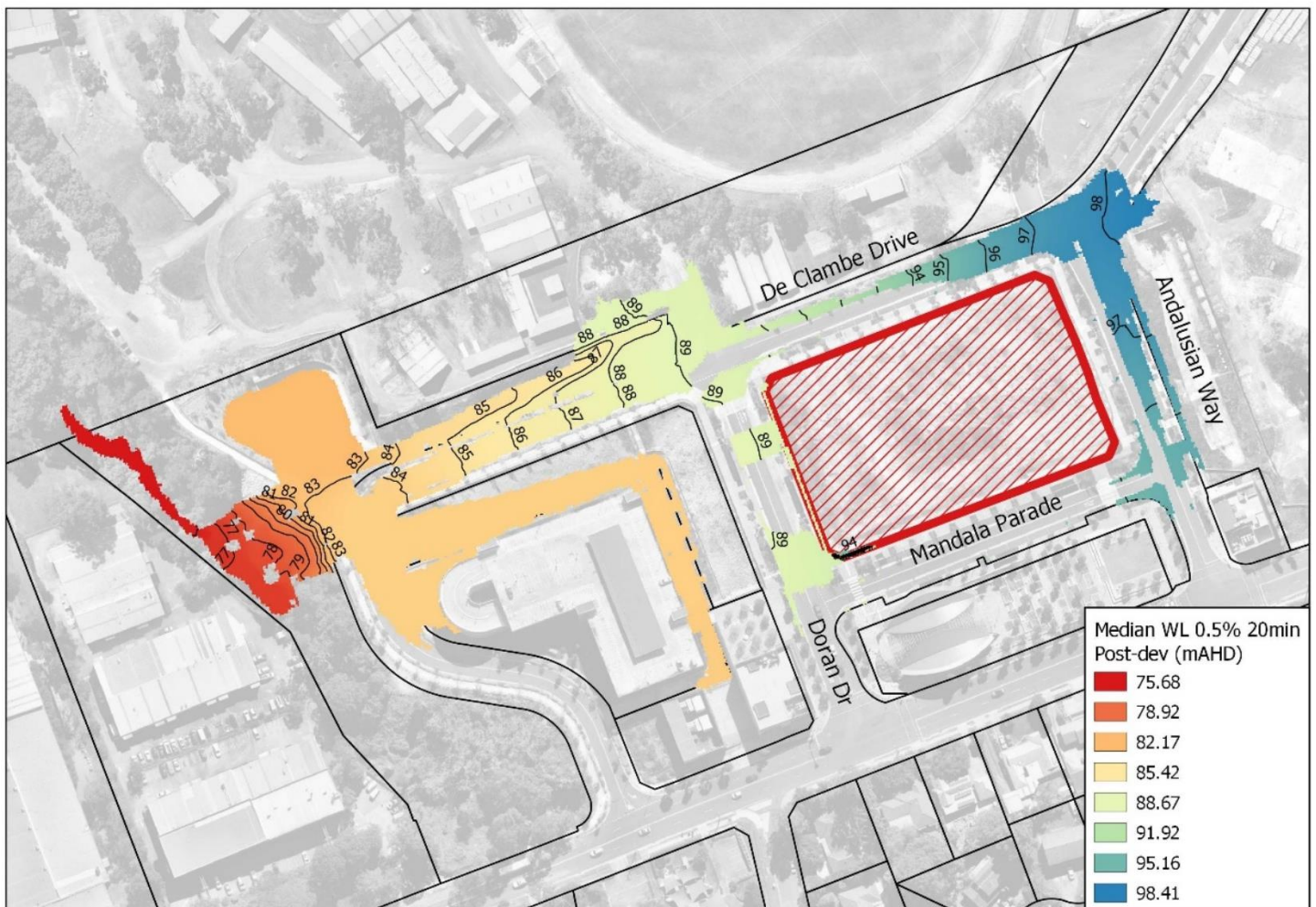
Figure 5.1 – Developed Scenario 0.5% AEP Flood Level
