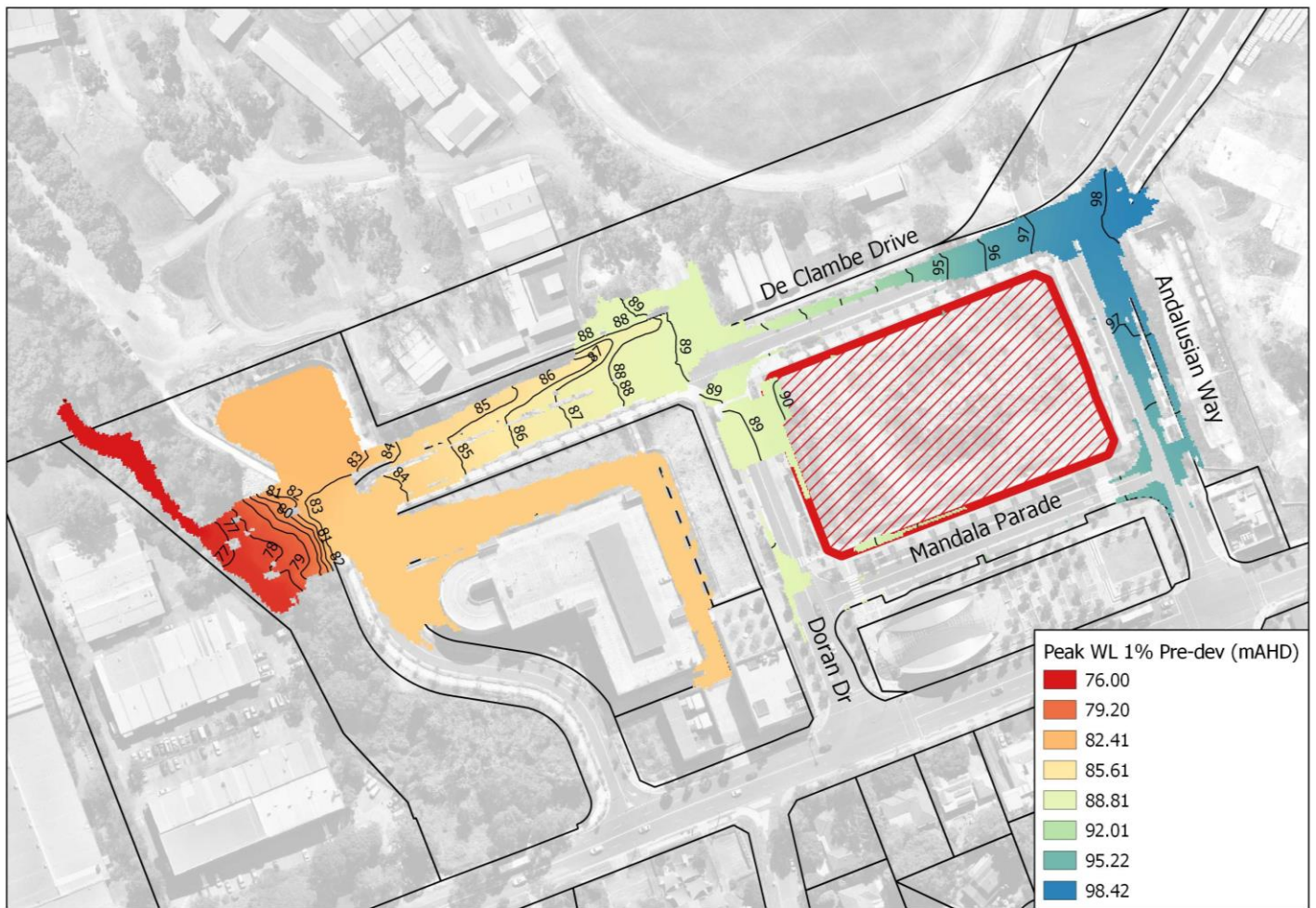
Figure 4.6 – Existing Scenario 1% AEP Flood Level
