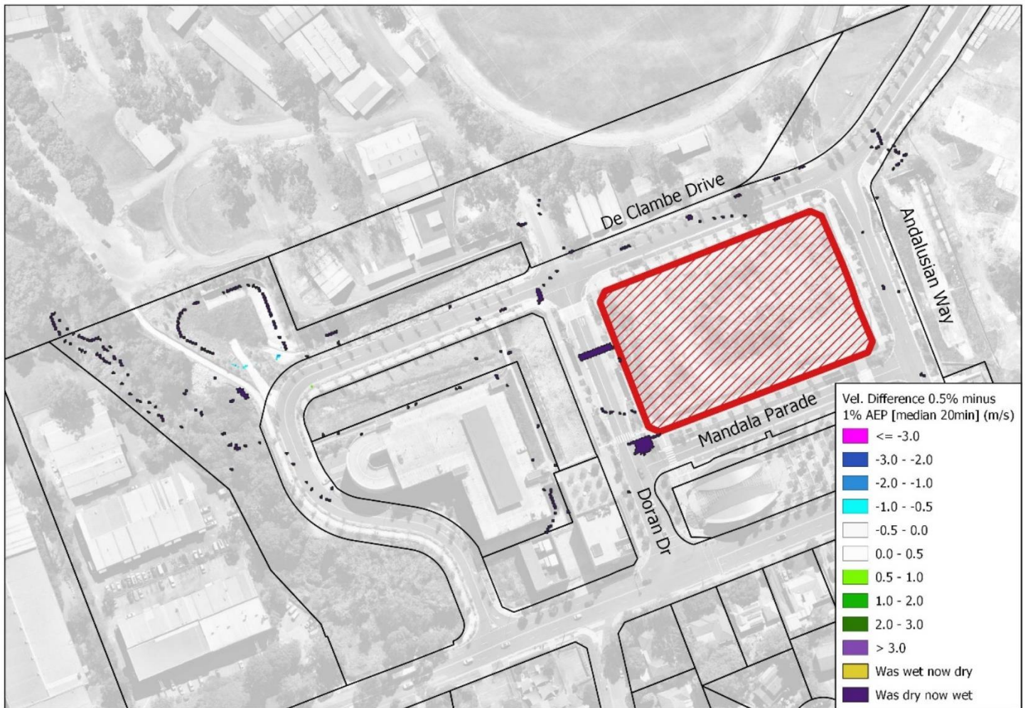
Figure 5.10 – Flood Velocity Difference – 0.5% AEP
