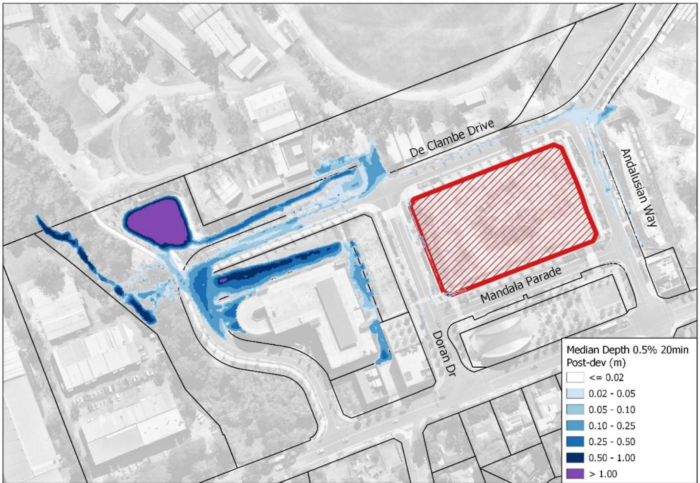
Figure 5.2 – Developed Scenario 0.5% AEP Flood Depth
