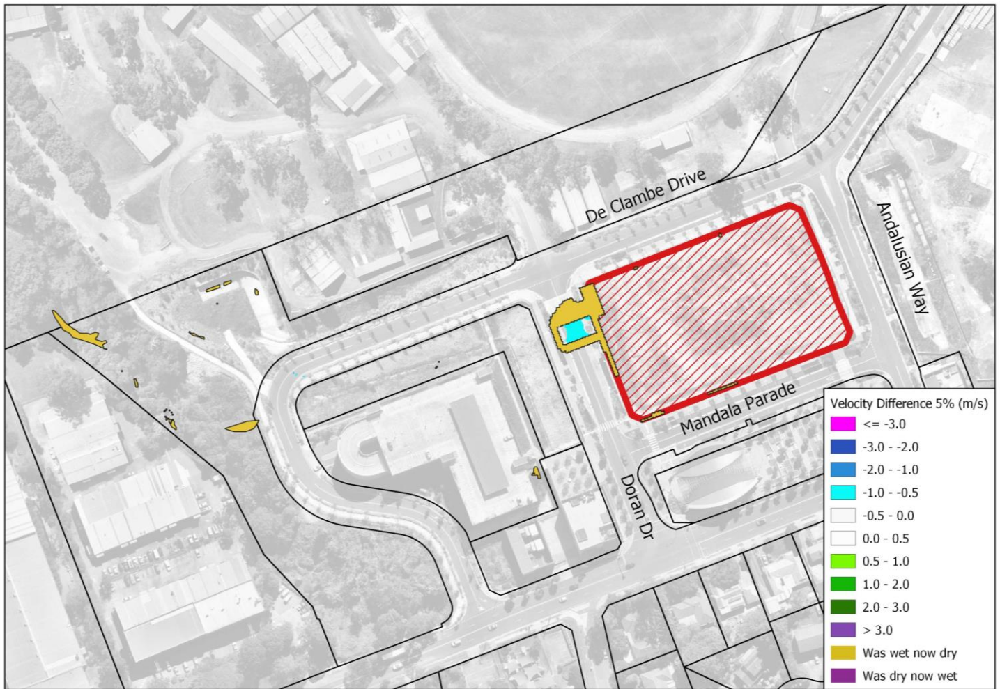
Figure 4.28 – Flood Velocity Difference – 5% AEP
