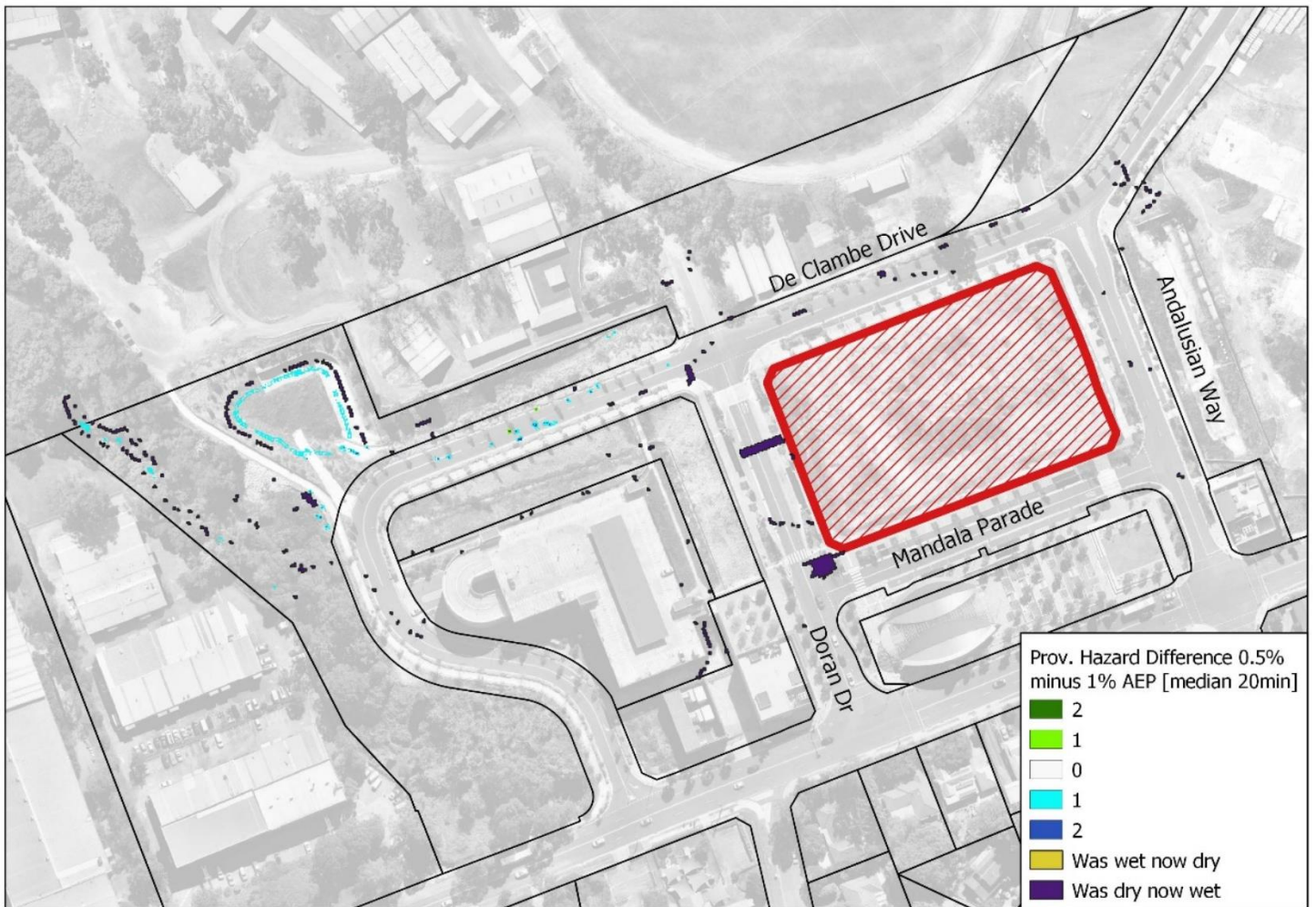
Figure 5.11 – Flood Hazard Difference – 0.5% AEP
