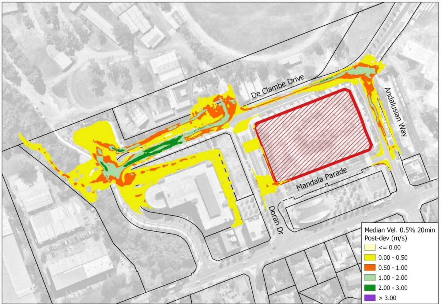
Figure 5.3 – Developed Scenario 0.5% AEP Flood Velocity
