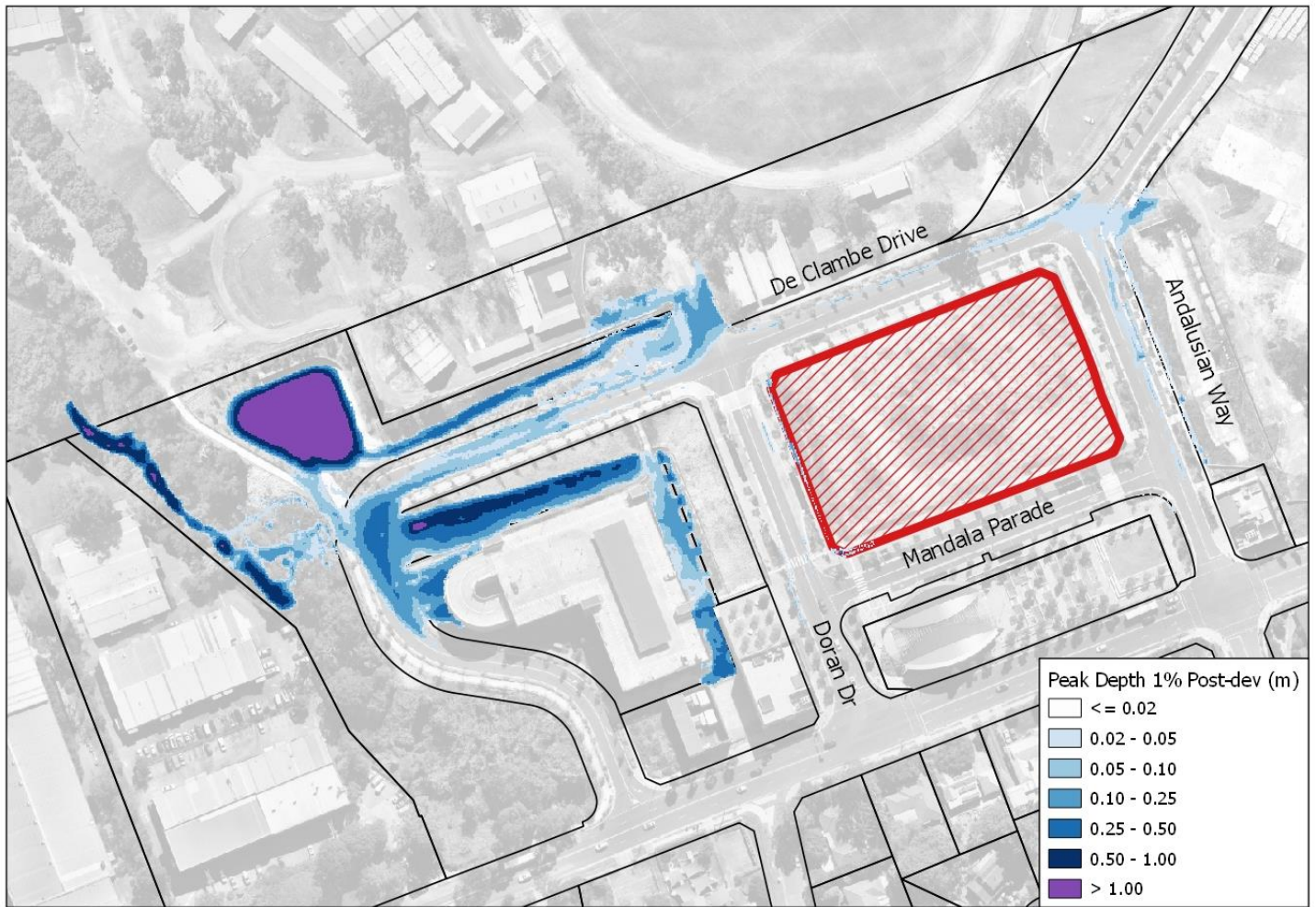
Figure 4.20 – Developed Scenario 1% AEP Flood Depth
