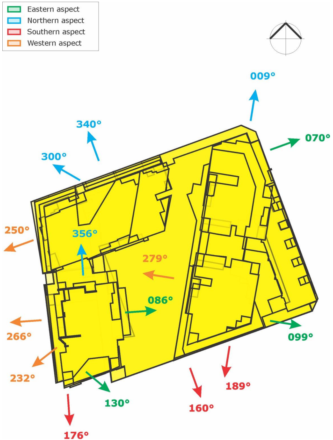
Figure 1: Critical Glazed Aspects of the Development (typical plan shown)
