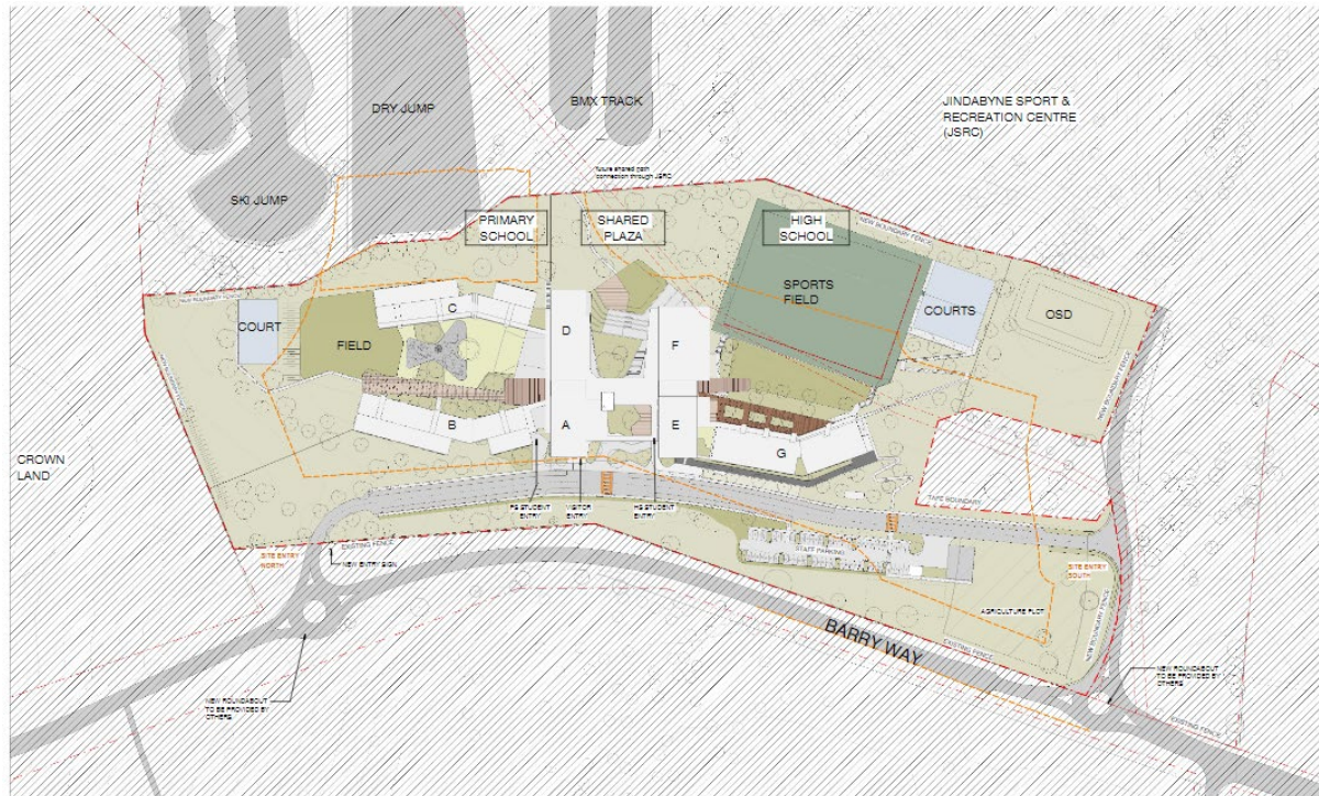
Figure 3-3 Site Layout
