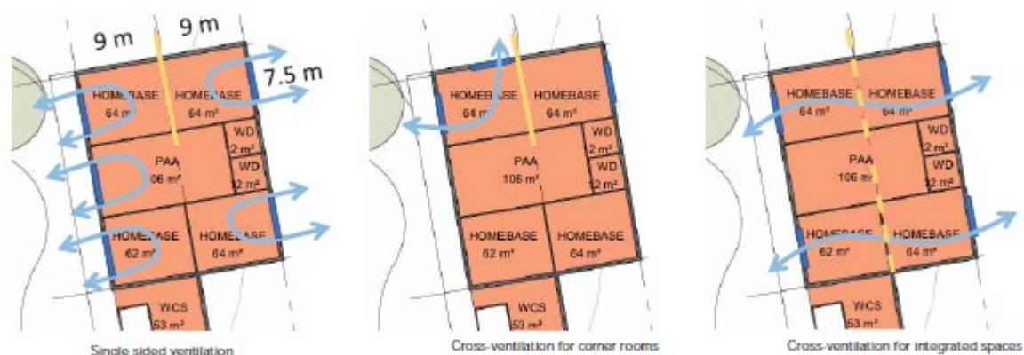
Figure 7-3 Ventilation diagram
