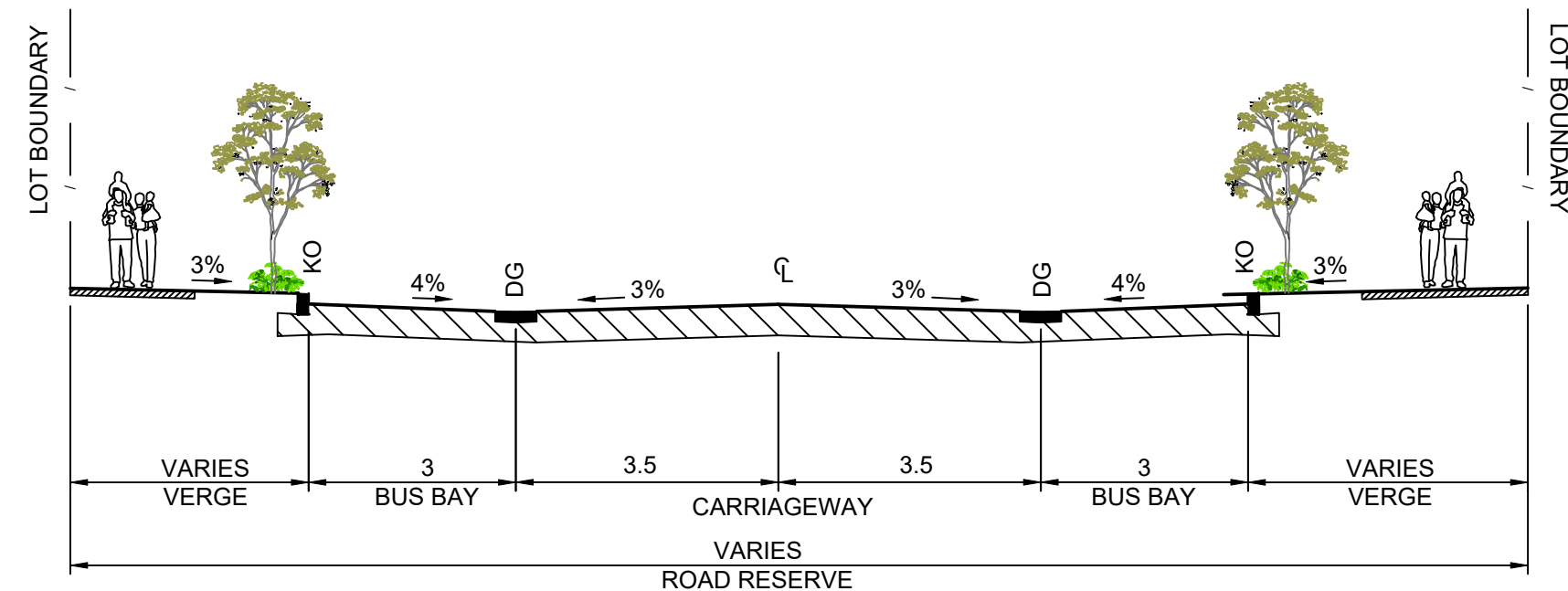
STURT STREET - BUS BAYS - BETWEEN SHORTLAND STREET & MEWS STREET EXIT 1:100
