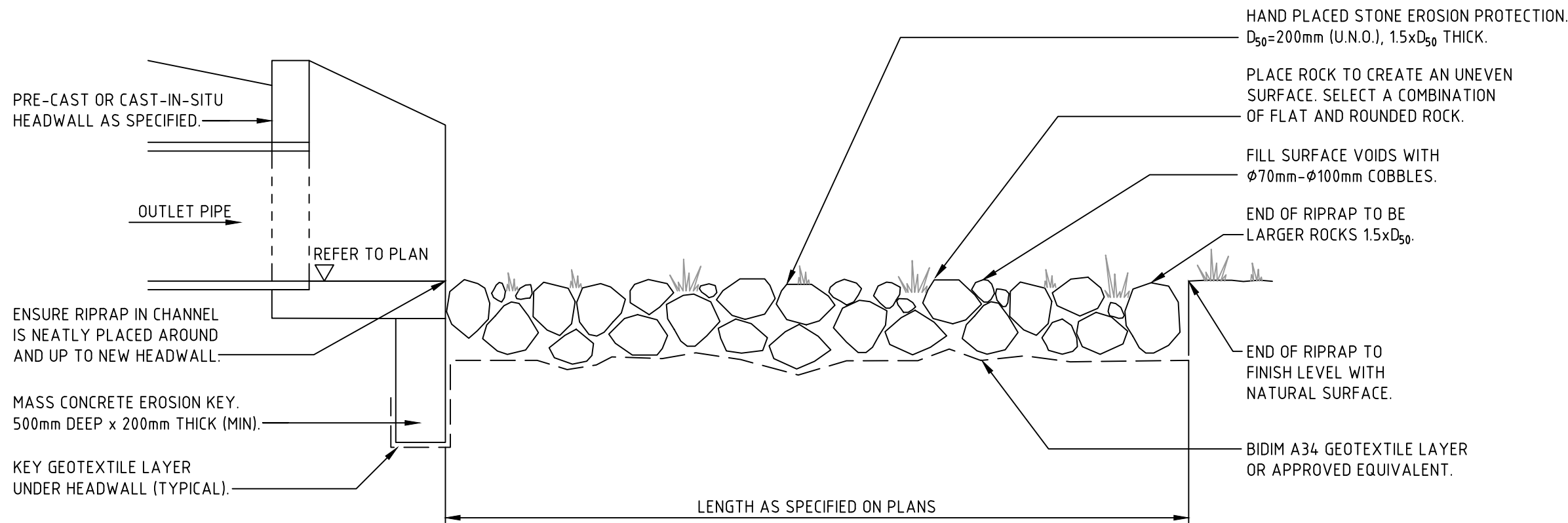
OUTLET HEADWALL RIPRAP SECTION
