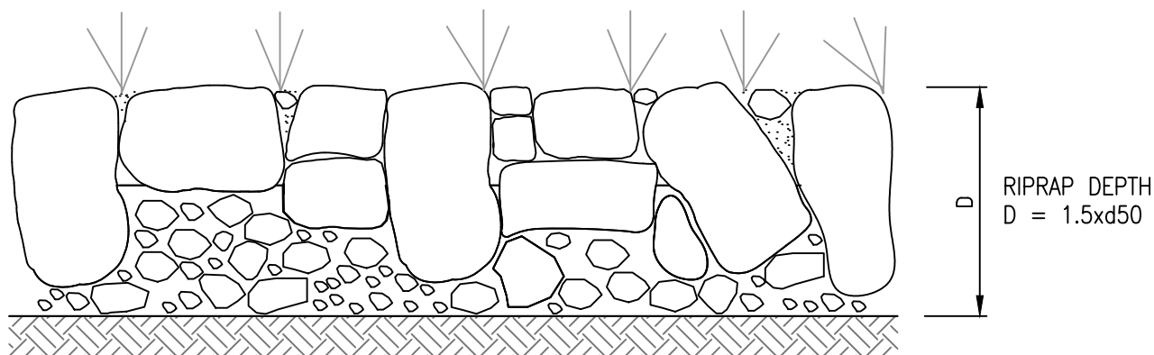
RIPRAP DETAIL
