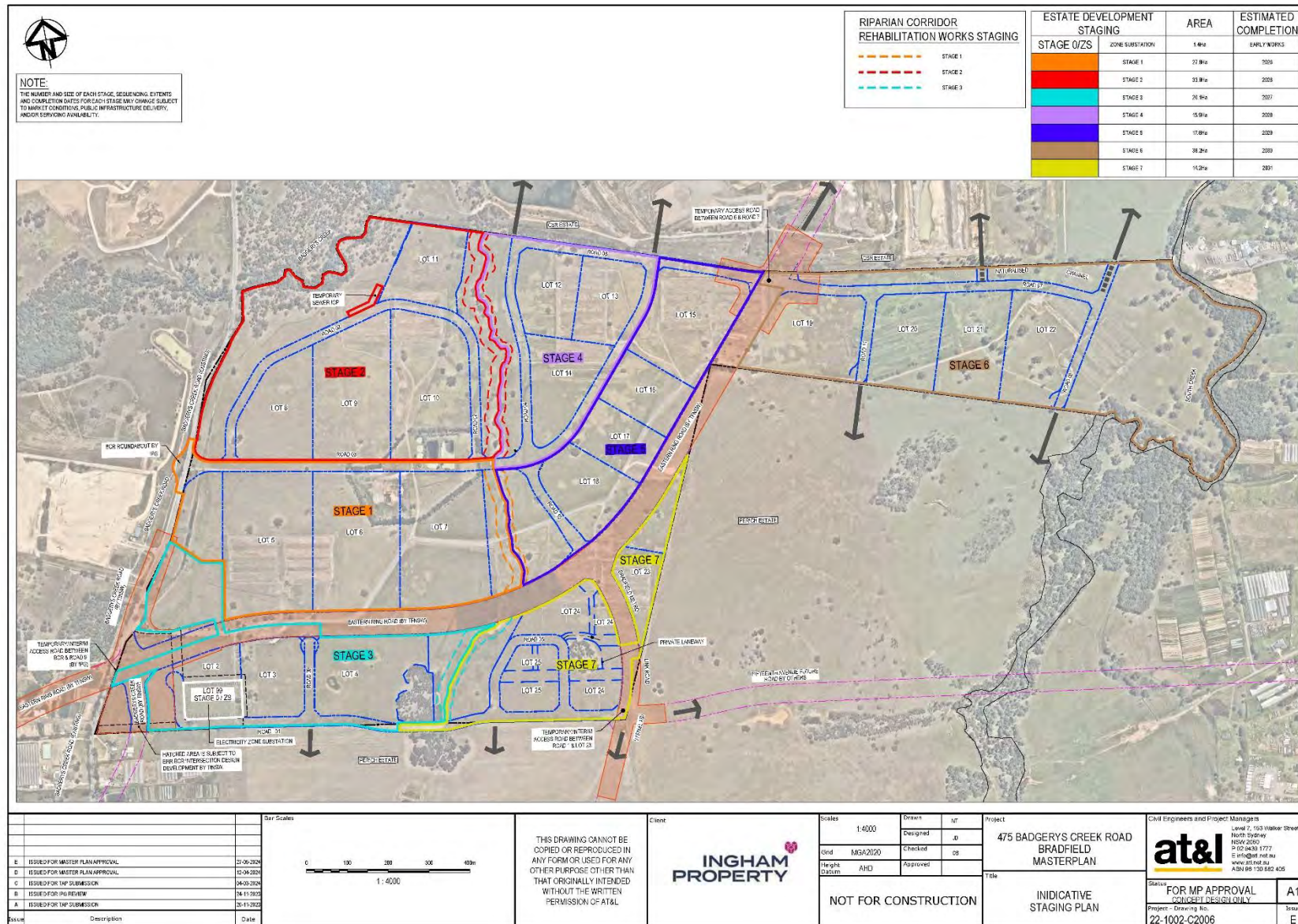
Figure 3: Stages Civil Works Plan for Complying Development (Site Image, 2025)
