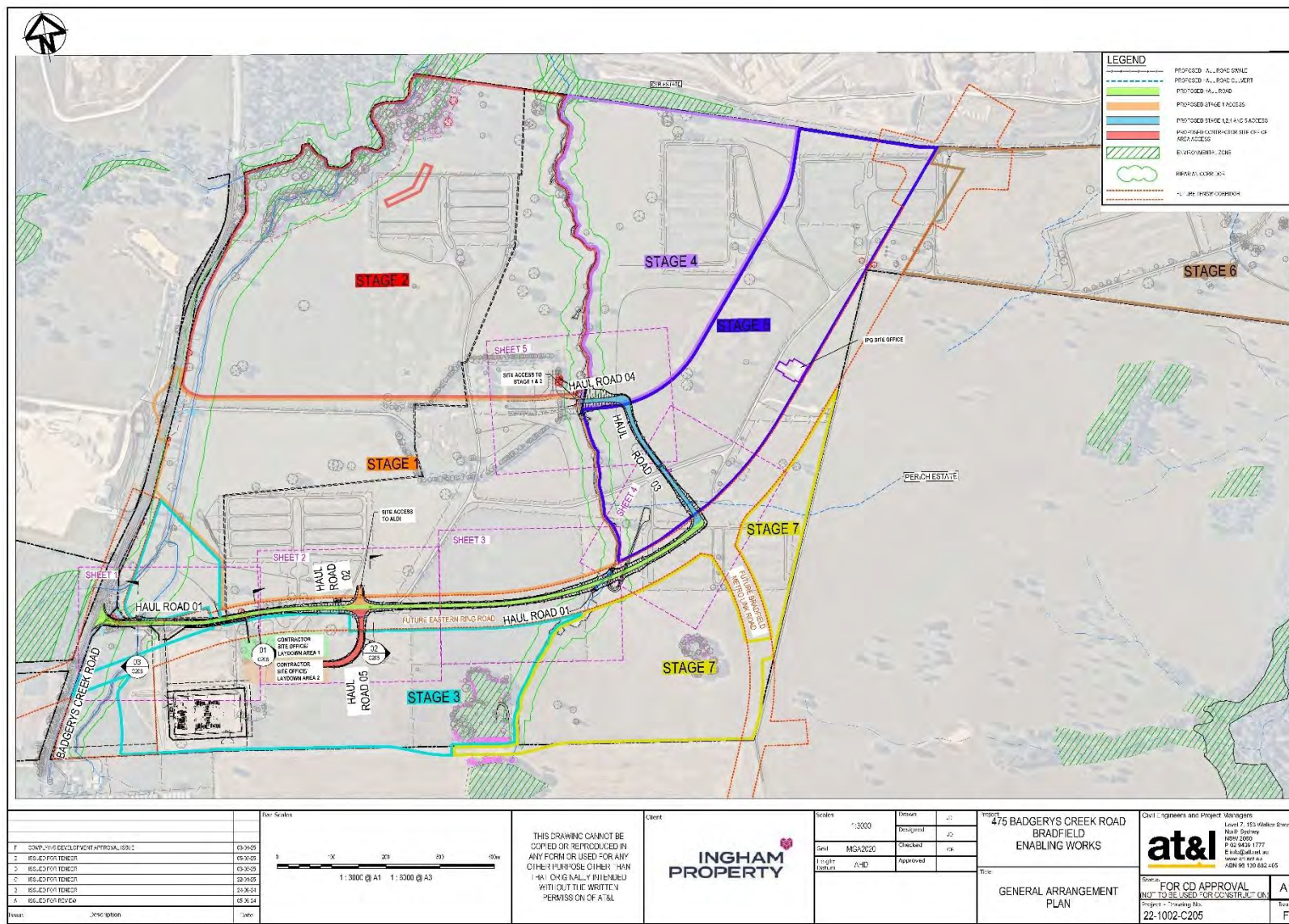
Figure 8: CDC 3 Temporary Haul Road for Stages 1 and 2 Civil Works
