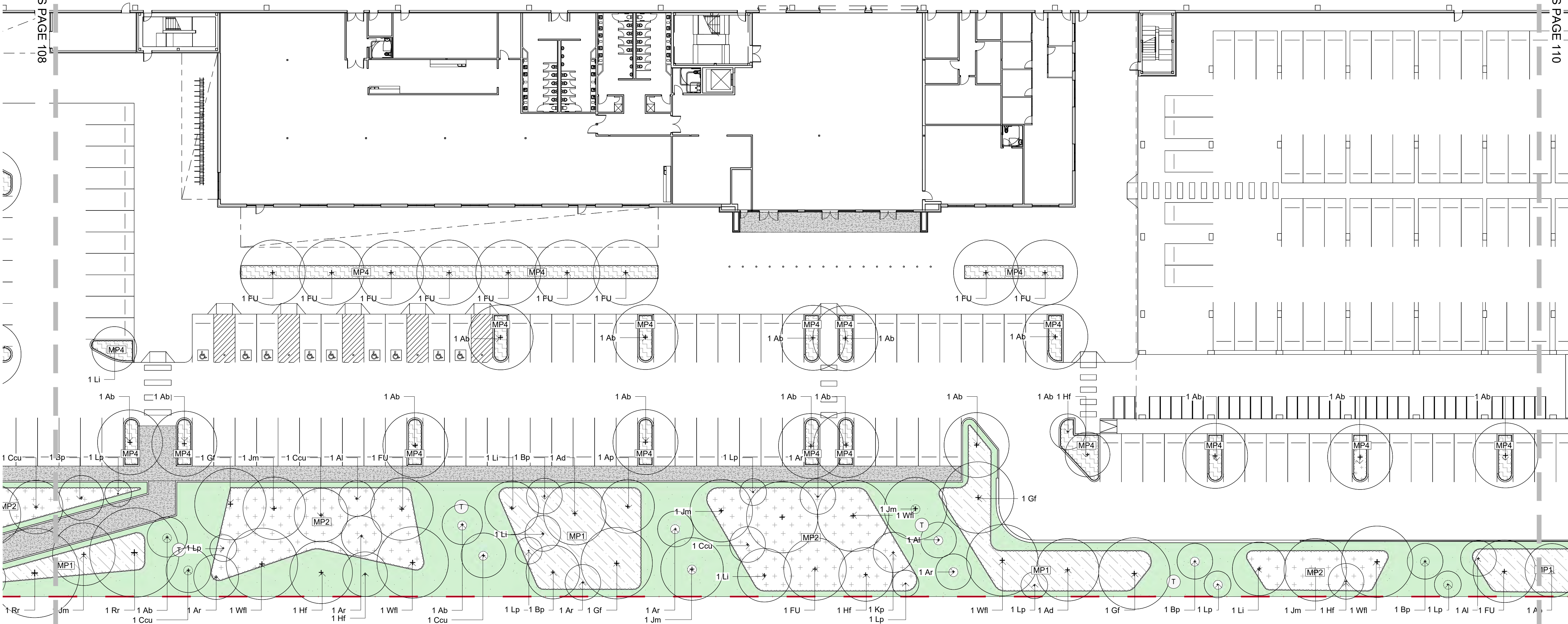
Key Plan
