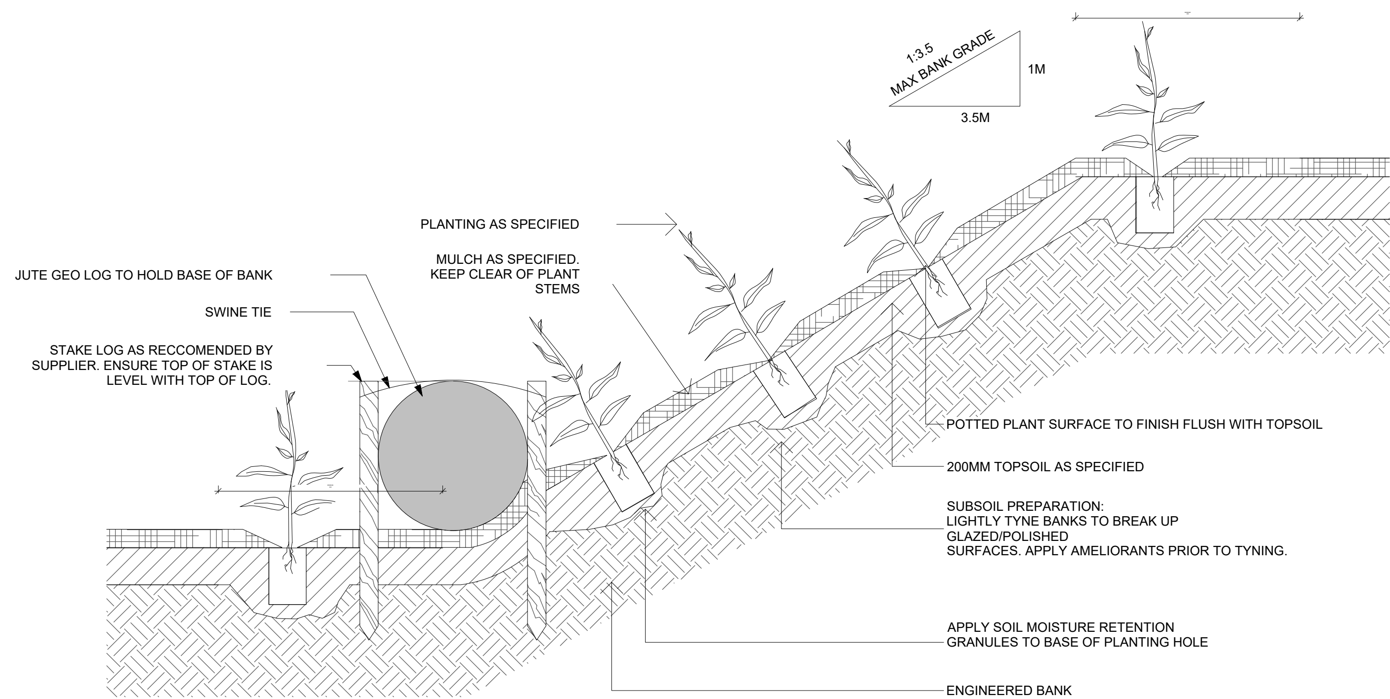
Typical Embankment Planting 1:10
