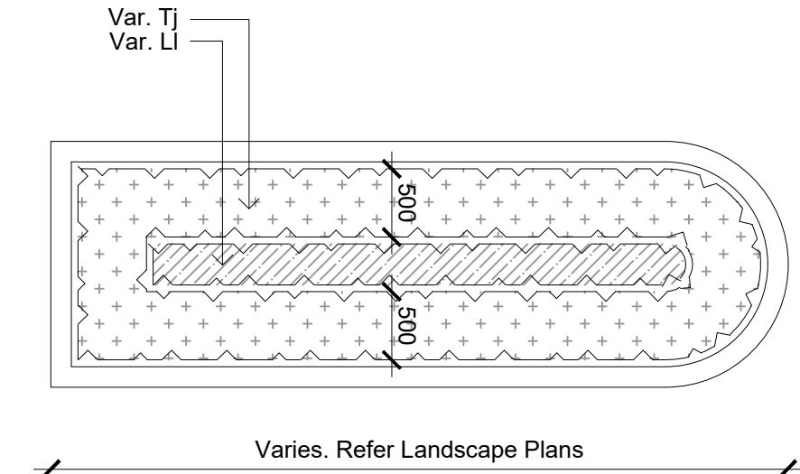
Planting Matrix 3 - Boundary Mix 1:50 Refer Landscape Plans & Schedule
