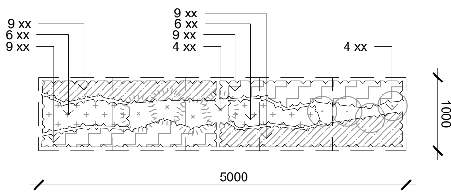
Planting Matrix 3 - Boundary Mix 1:50 Refer Landscape Plans & Schedule
