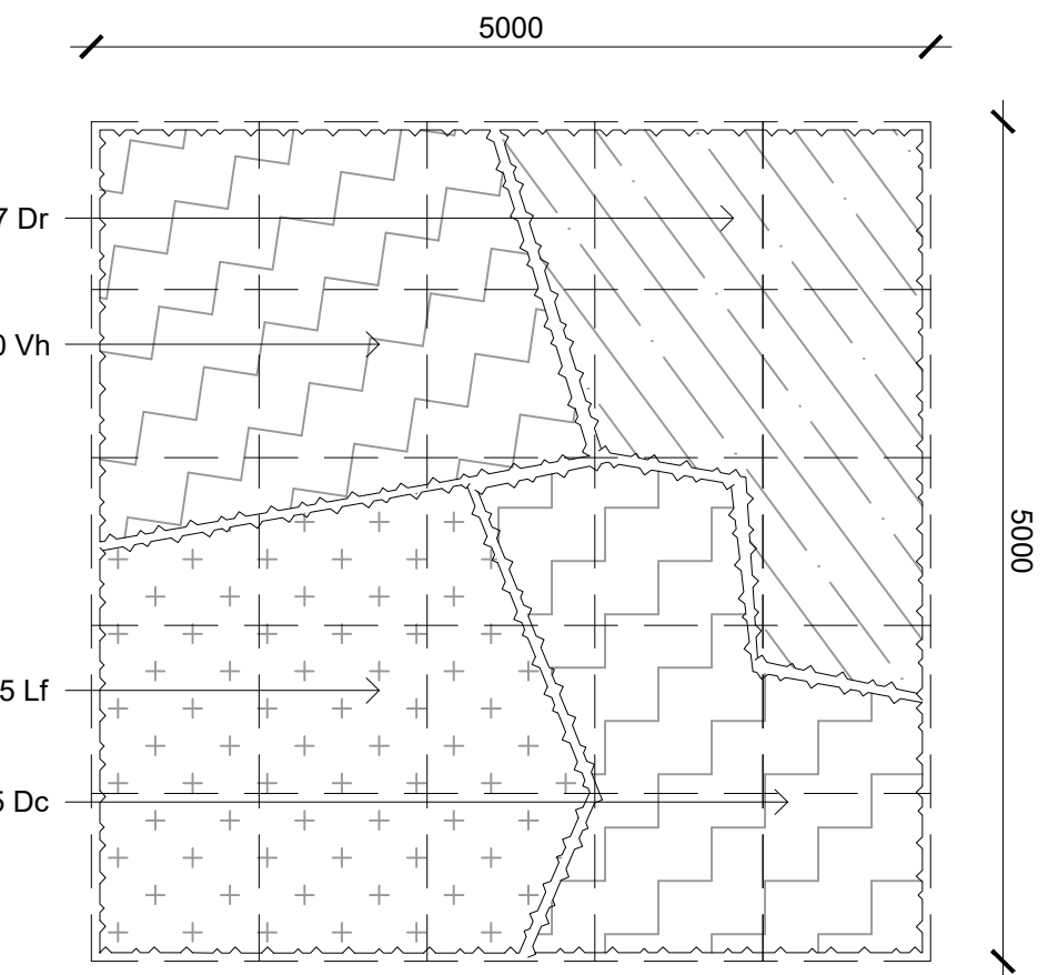
Planting Matrix 1 - Understory Mix A 1:50 Refer Landscape Plans & Schedule
