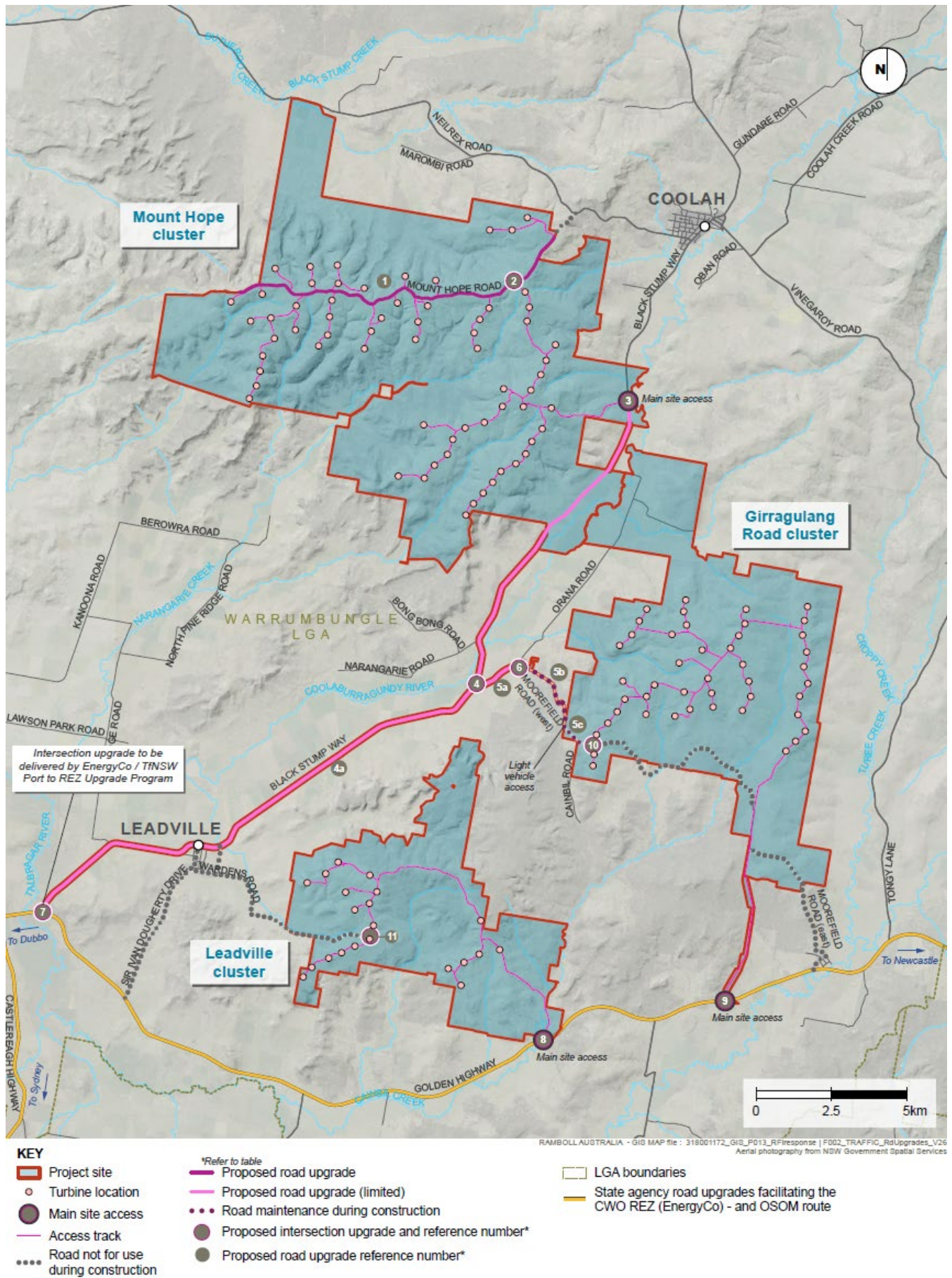
Figure 11 | Road and intersection upgrades
