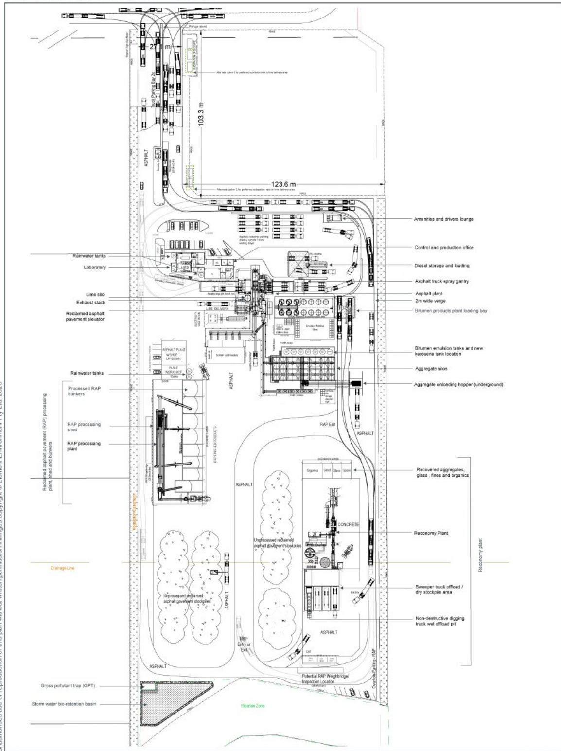
Figure 4. Layout of Lot 6 (from: Element Environment, 2020b).
