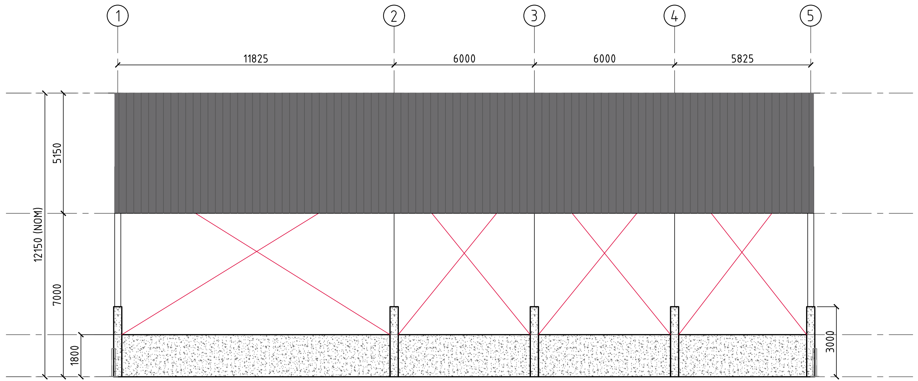
RECOVERED MATERIALS STORAGE BUNKER - SOUTHERN ELEVATION SCALE 1:100
