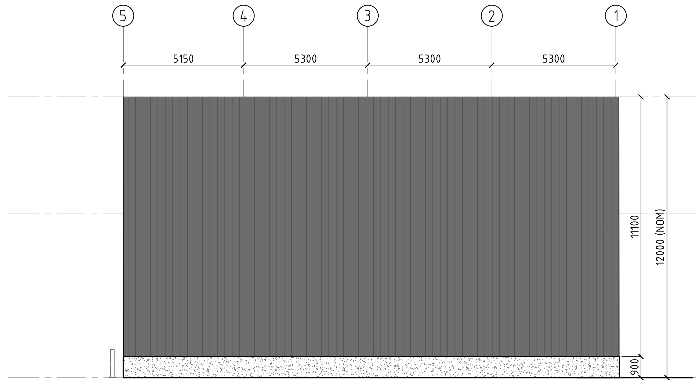
RECONOMY RECEIVAL PITS - NORTHERN ELEVATION SCALE 1:100
