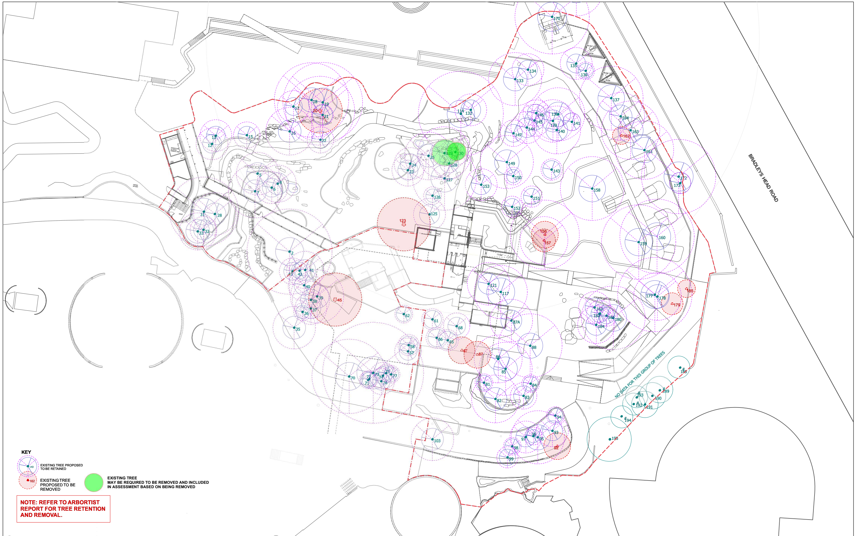
1 TREE PROTECTION AND REMOVAL PLAN 1:250
