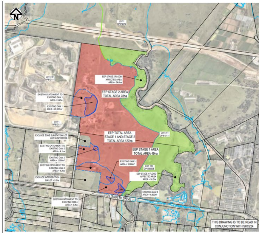
Figure 5A: Stage 1 Development, Phase 2 Stormwater Management Plan
