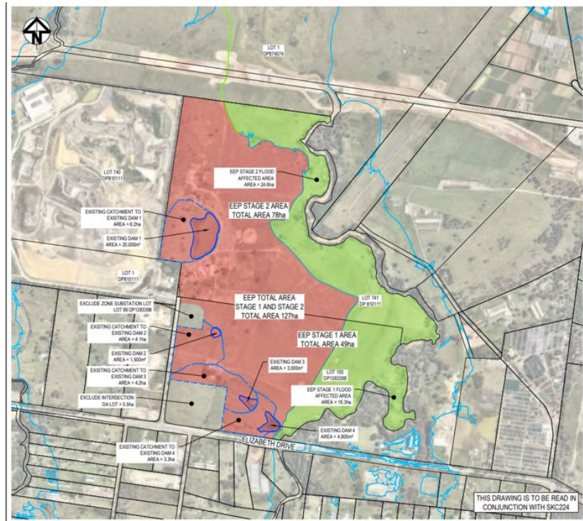
Figure 5: Stage 1 Development, Phase 1 Stormwater Management Plan
