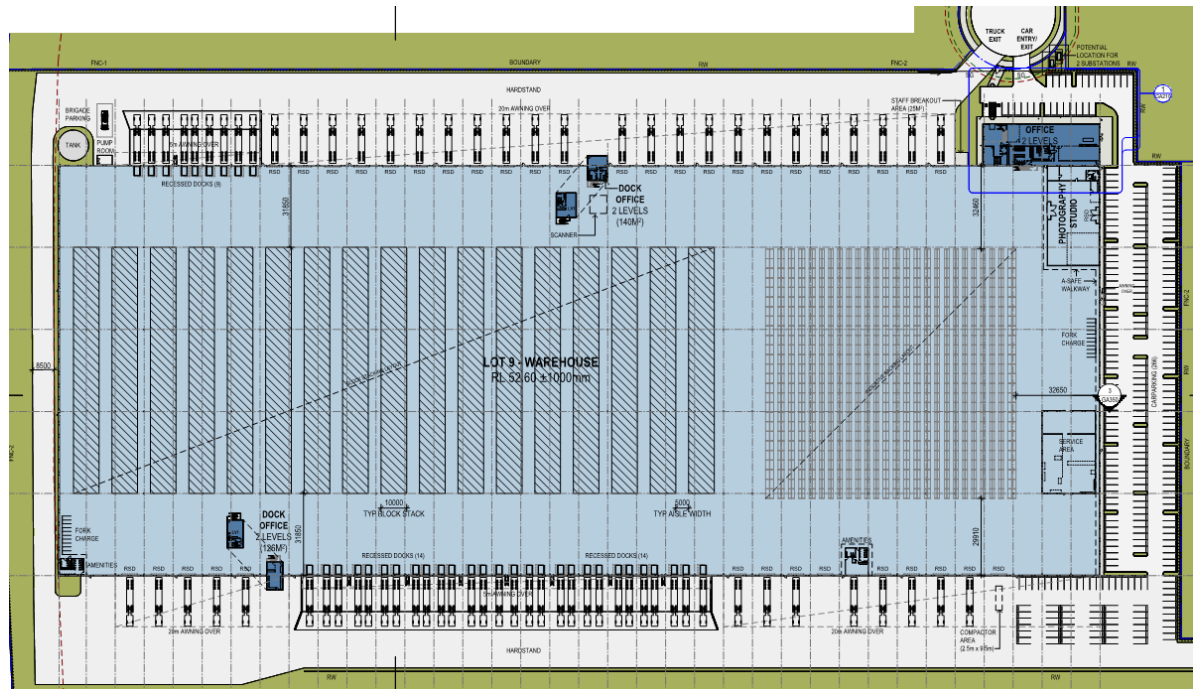
SBA Architects Drawing No. DA-910 Rev. K dated 25.05.2022
