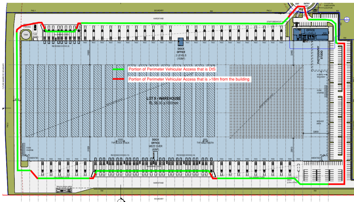
Figure 1 – Warehouse 9 Perimeter Vehicular Access per BCA C2.4.
