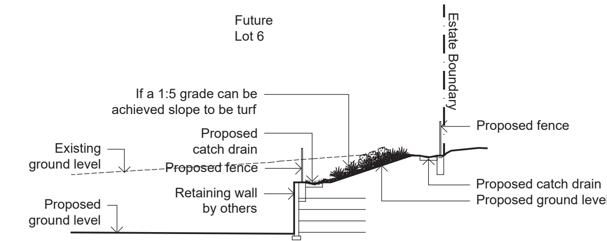
Section F 1:200
