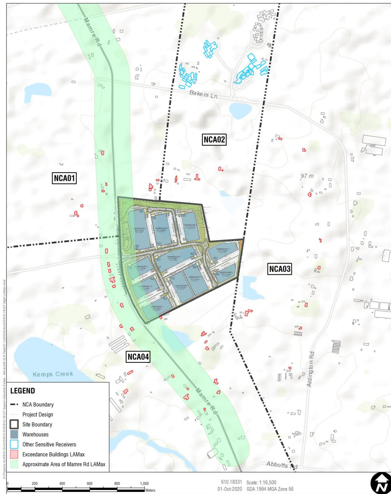
Figure 12 Predicted Exceedance of Sleep Disturbance Screening Noise Level – Noise-Enhancing Weather Conditions – Masterplan Site
