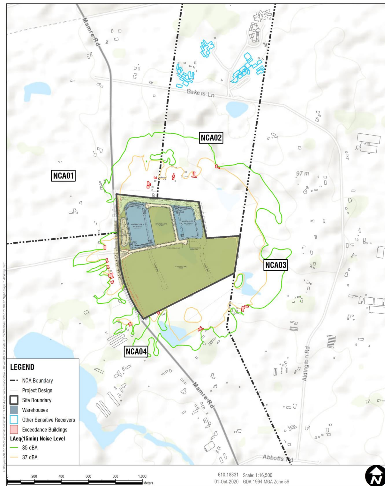
Figure 14 Predicted Noise Levels – Night – Noise-Enhancing Weather Conditions – Stage 1 Site
