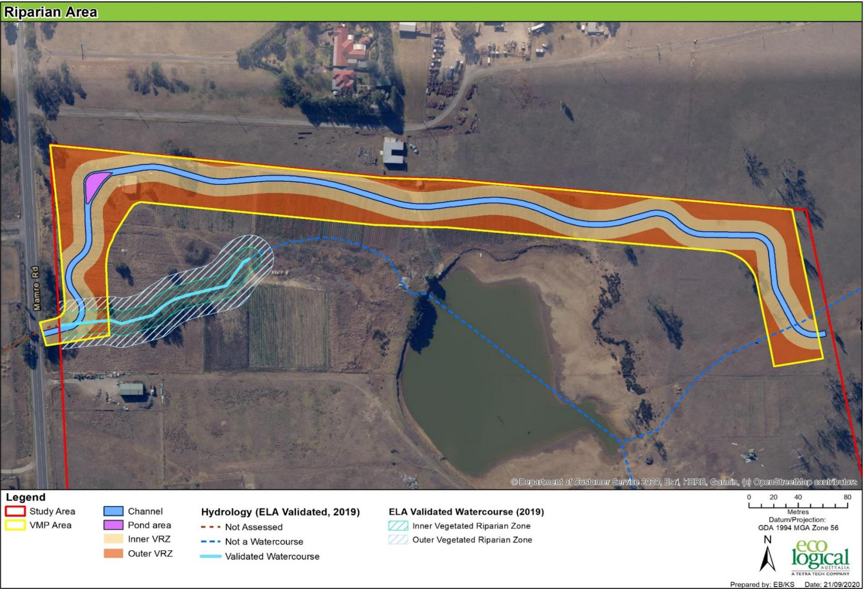
Figure 23: Proposed location of new vegetated channel
