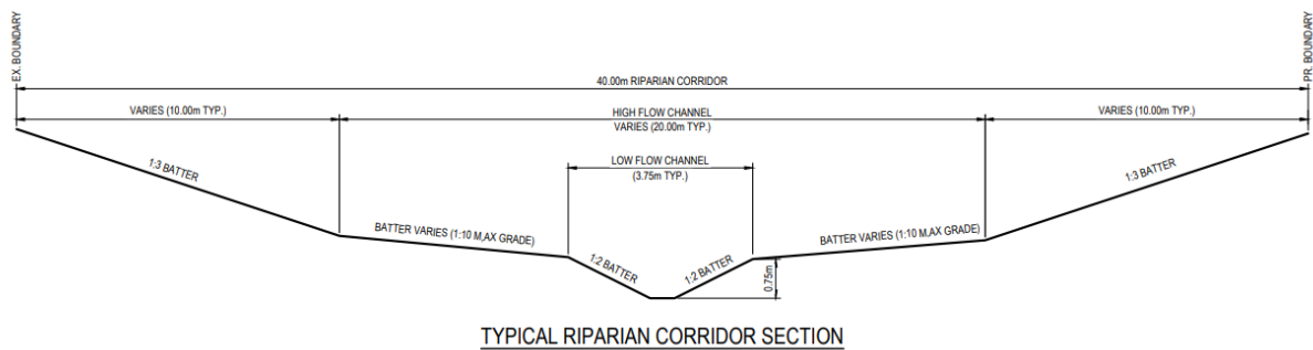
Figure 22: Typical riparian corridor cross section (AT&L, 15 October 2020)
