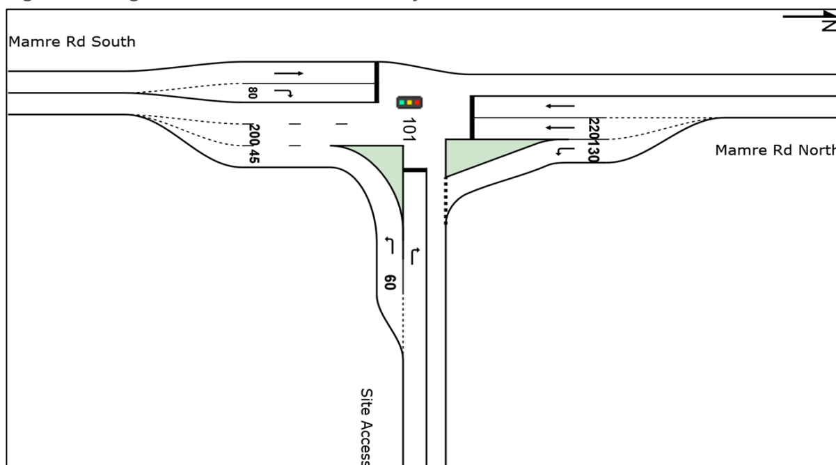
Figure 23: Stage 1 2026 SIDRA Intersection Layout
