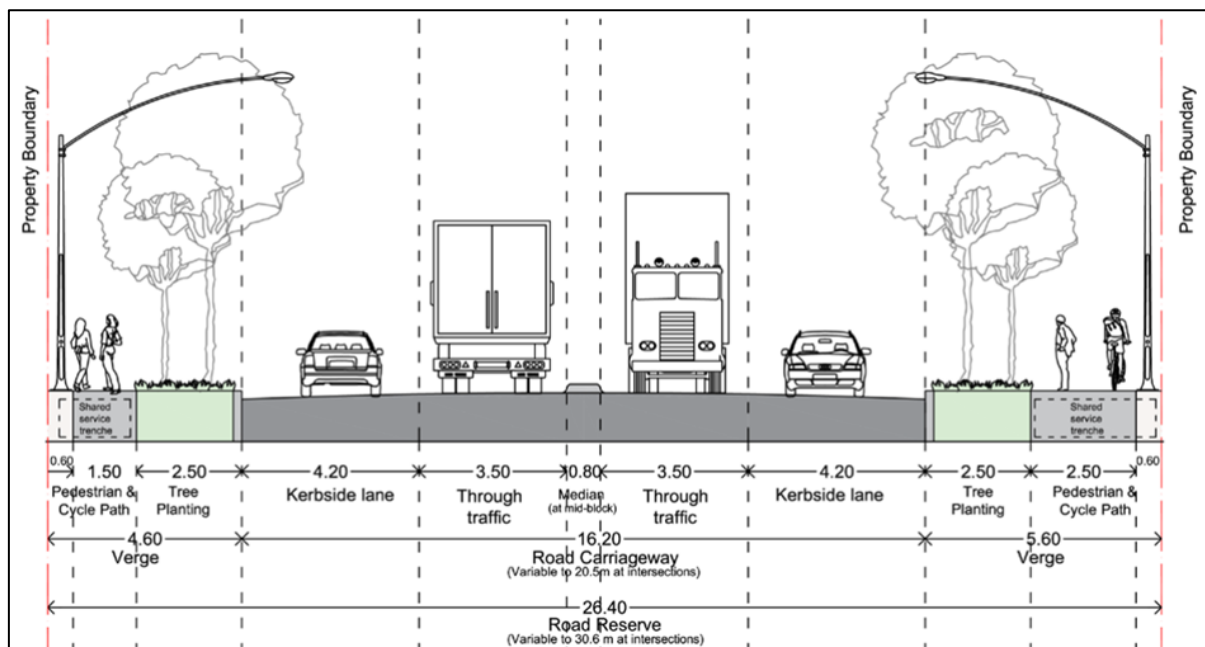
Figure 9: Draft DCP Typical Local Industrial Road
