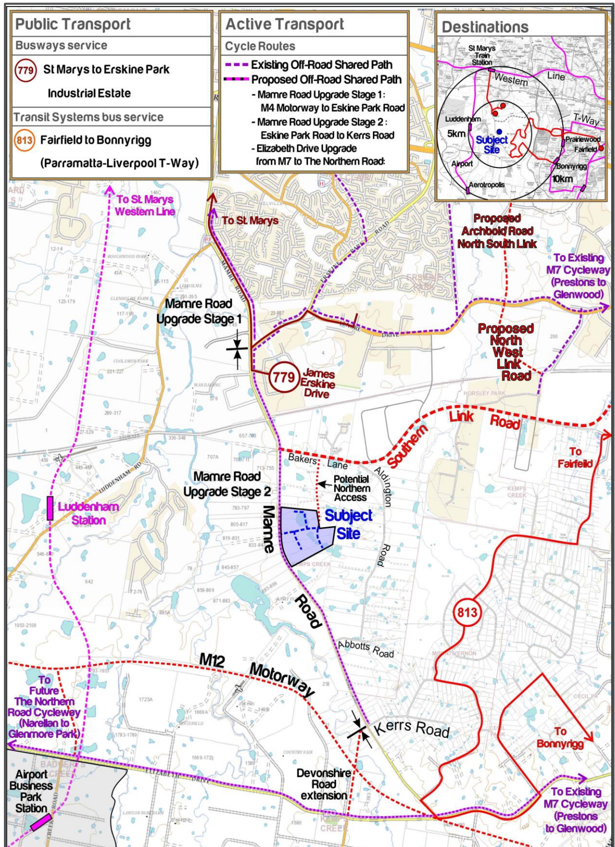
Figure 10: Public & Active Transport Network
