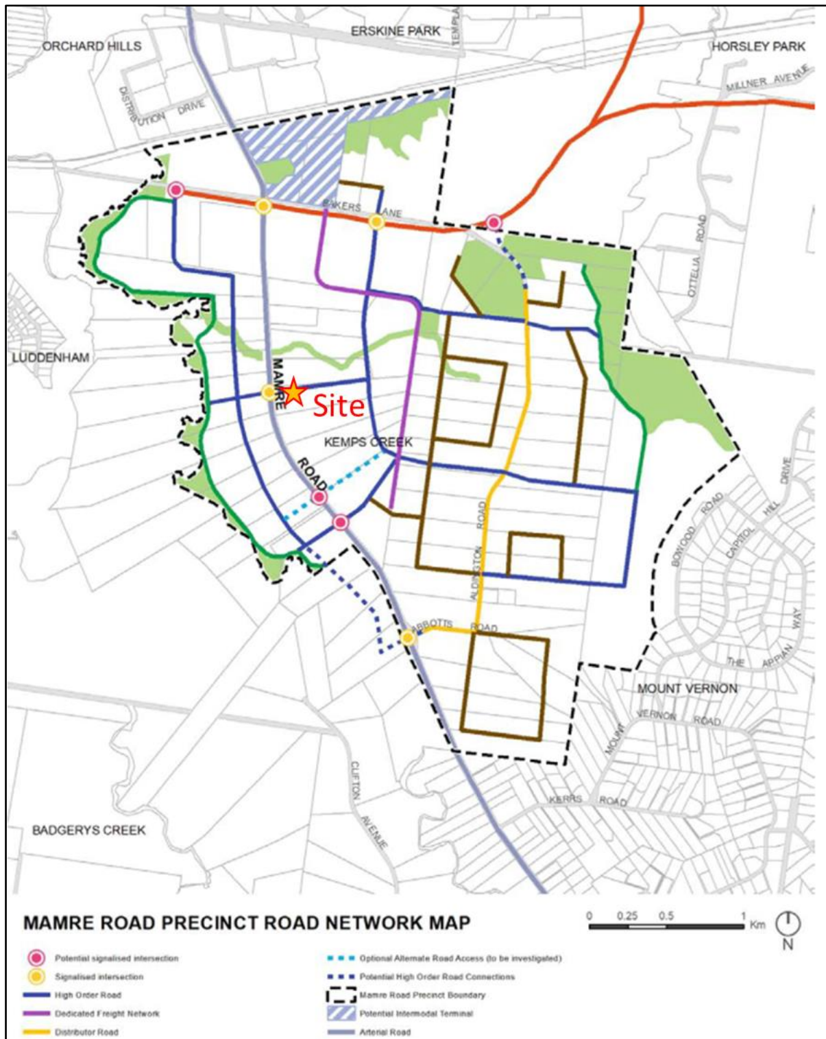
Figure 7: Draft DCP Proposed Precinct Roads
