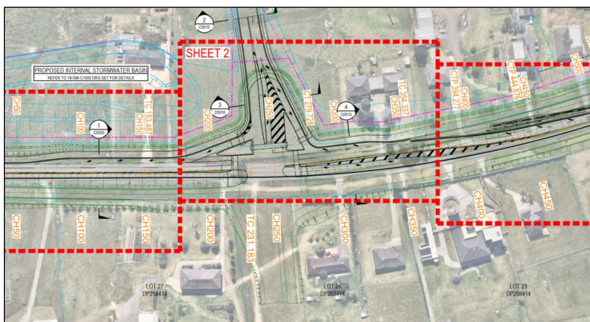
Figure 22: Stage 1 2026 Intersection Design
