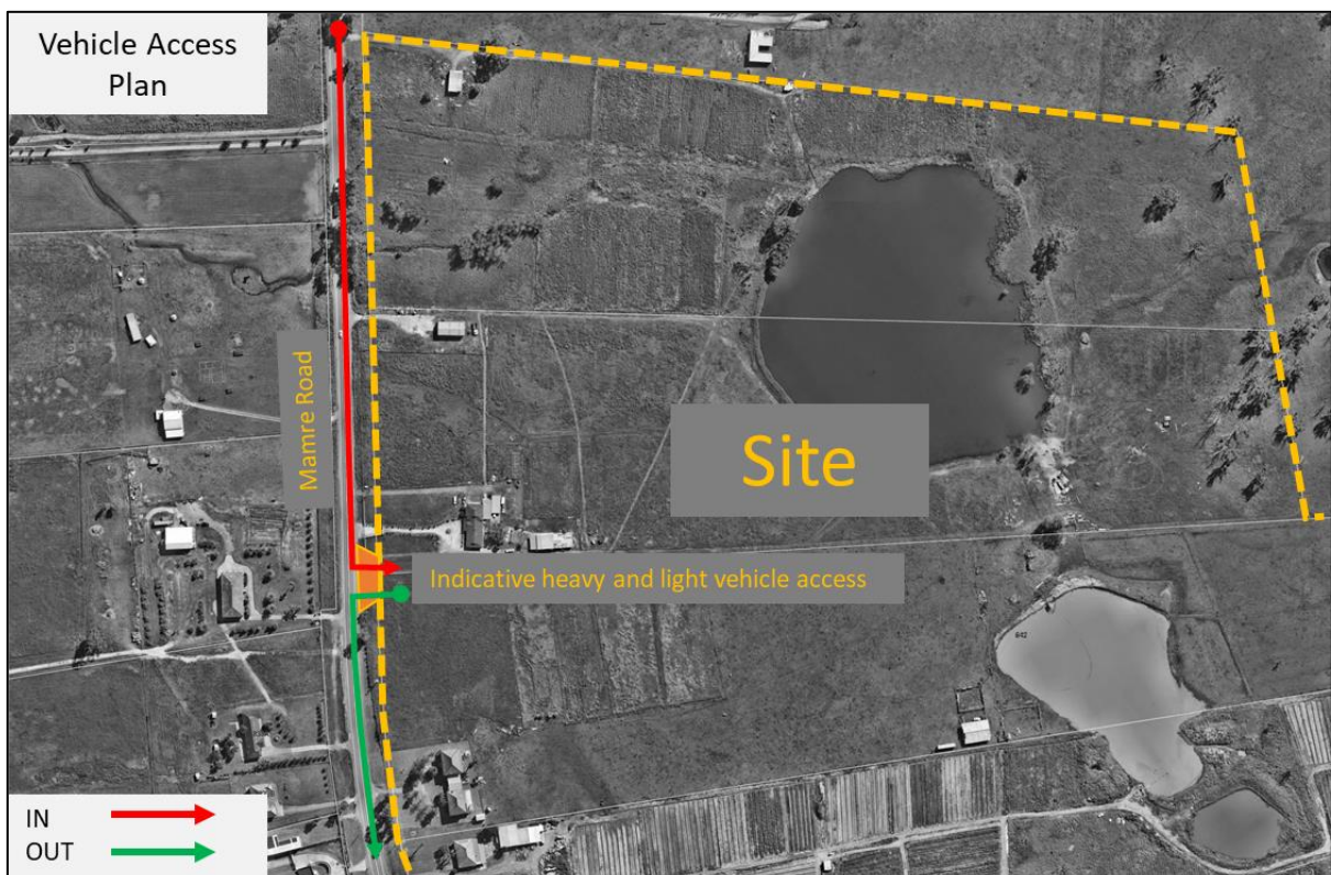
Figure 4: Indicative Vehicle Access Plan
