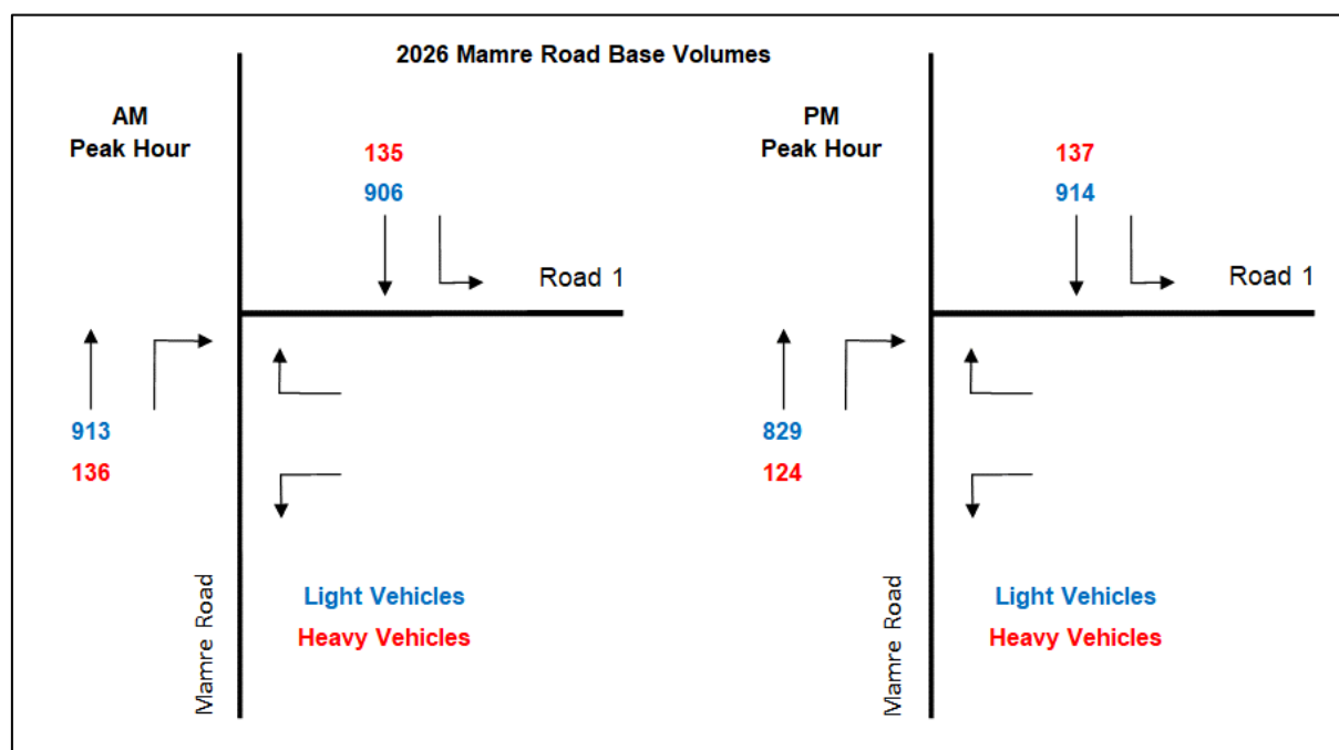
Figure 15: 2026 Mamre Road Base Flows
