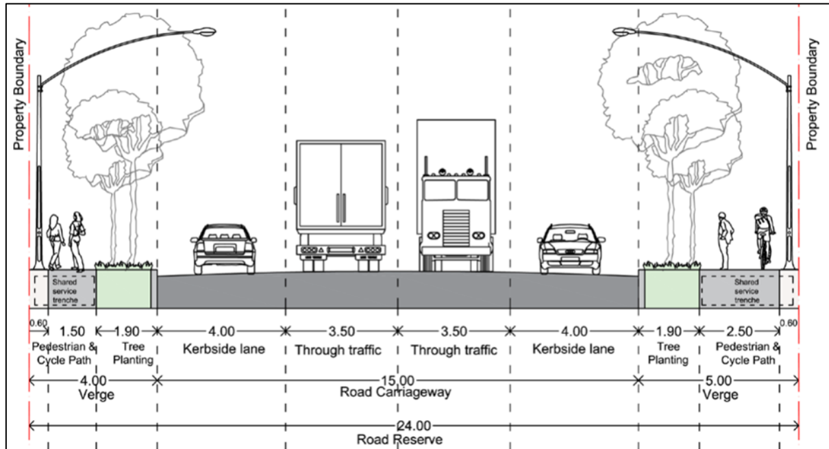
Figure 8: Draft DCP Typical Local Industrial Road
