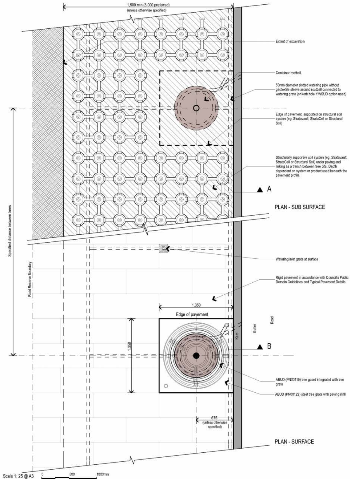
TYPE 10A - INDICATIVE TREE PLANTING WITH STRUCTURAL SUPPORT & CONTINUOUS TRENCH [PLANS]
