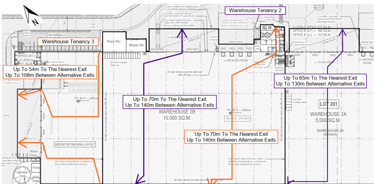
Figure 6-2: Indicative Maximum Non-Compliant Travel Distances within Warehouse Tenancies 2 and 3
