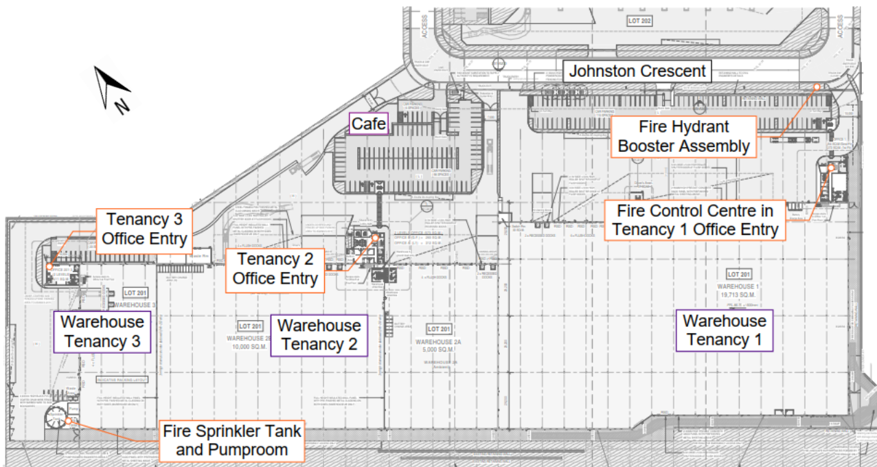
Figure 2-3: Site Plan & Building Description
