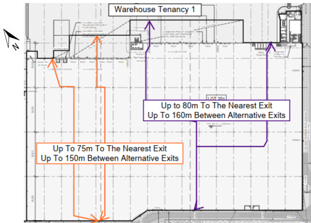
Figure 6-1: Indicative Maximum Non-Compliant Travel Distances within Warehouse Tenancy 1
