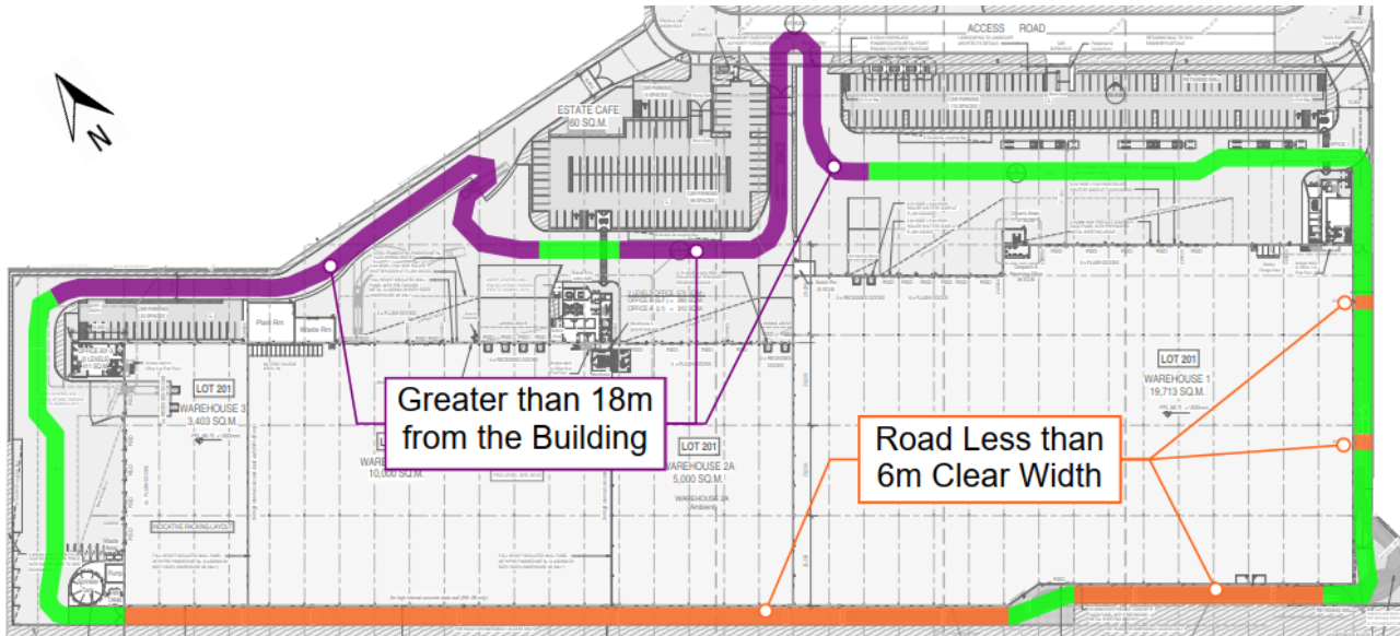
Figure 6-7: Vehicular Perimeter Path and Sections of Non-Conformance
