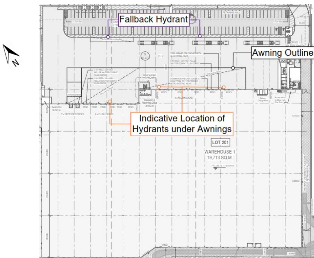
Figure 6-5: Indicative Hydrant Locations Beneath Awnings and the Additional Fallback Hydrants – Tenancy 1
