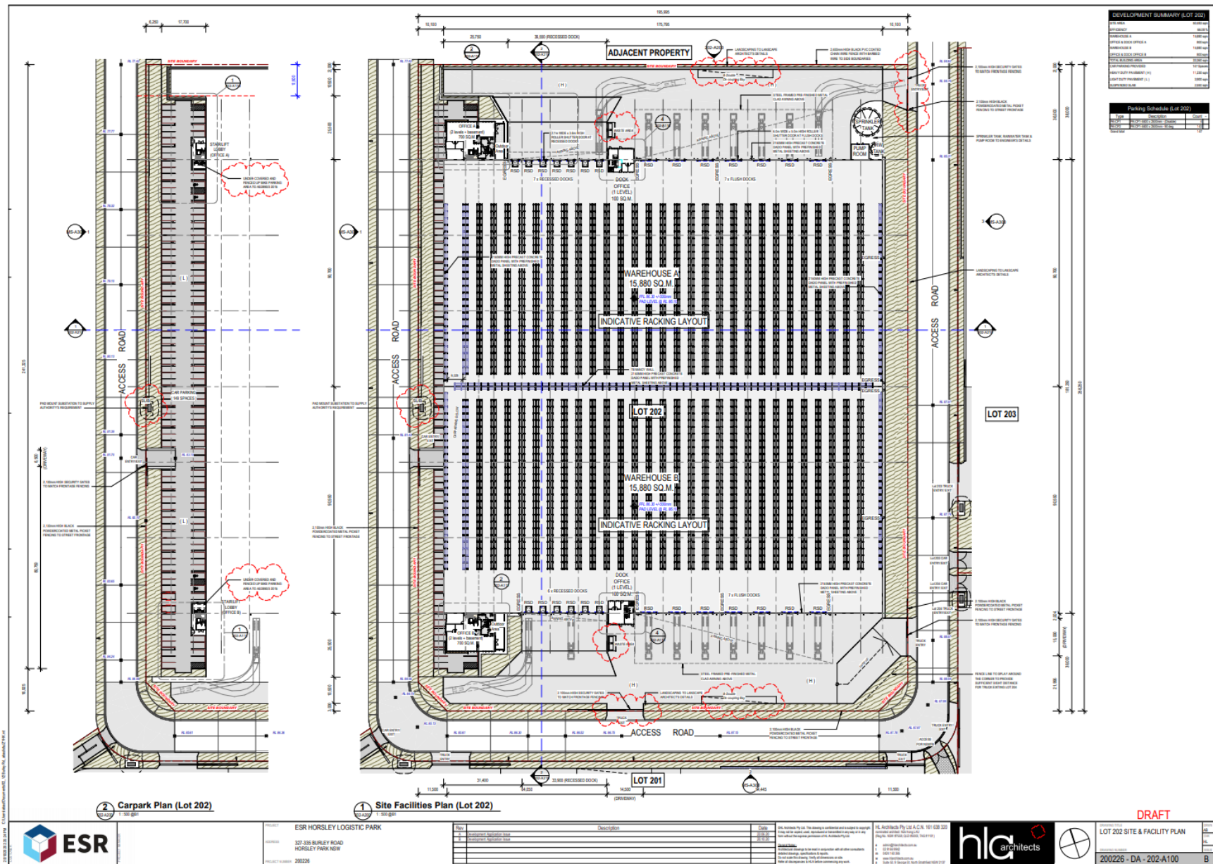
Figure 3: Lot 202 Plan
