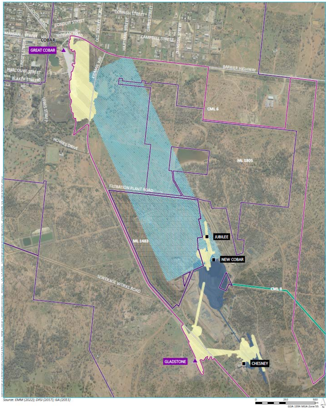
Underground development layout
