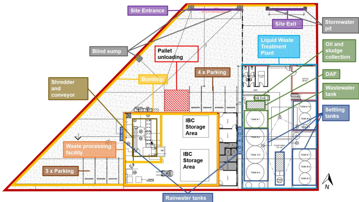
Figure 3 | Site Layout
