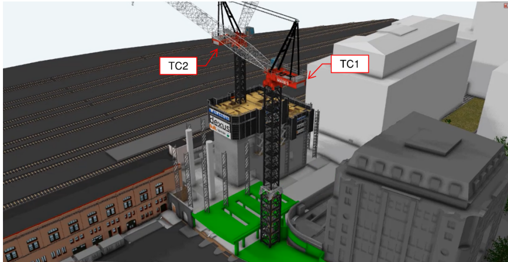
Figure 1-43: Atlassian Tower Crane Overview
