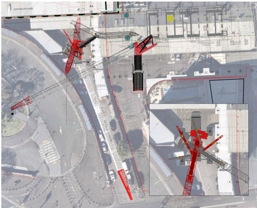
Figure 1-47: Mobile crane location mark-up
