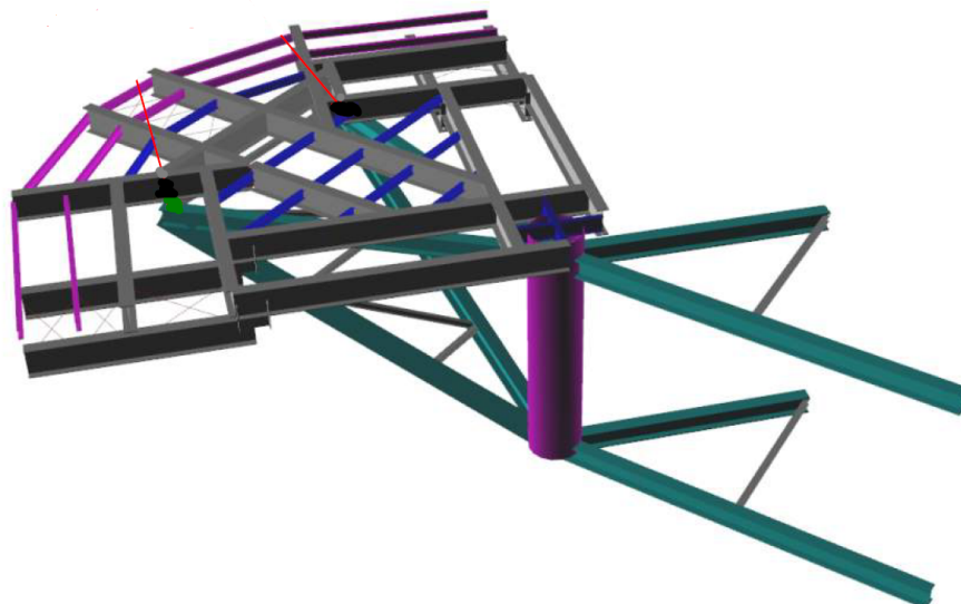
Figure 1-55b: North-East Oversail Temporary Engineering Concept
