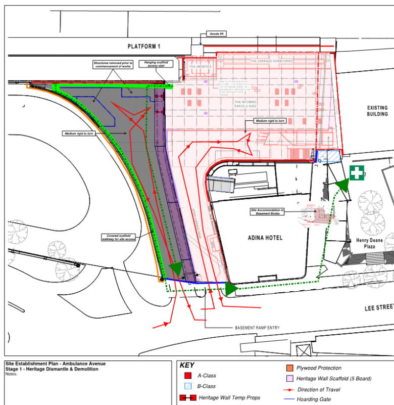
Figure 1-39a: Phase 1 – demolition & retention egress pathway
