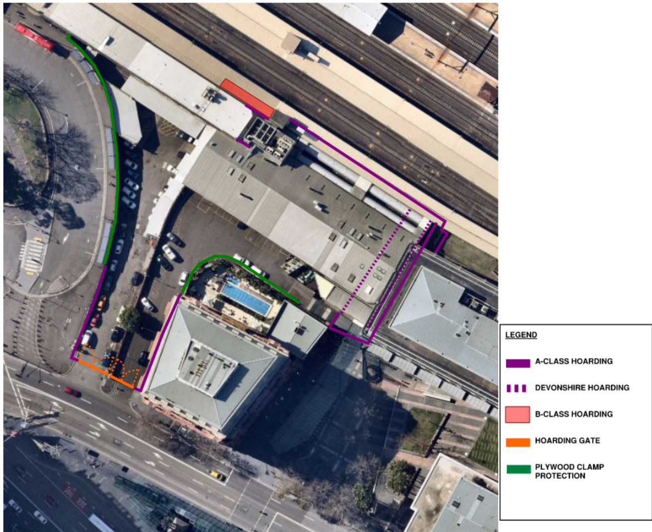
Figure 1-14: Overall Hoarding Layout Plan
