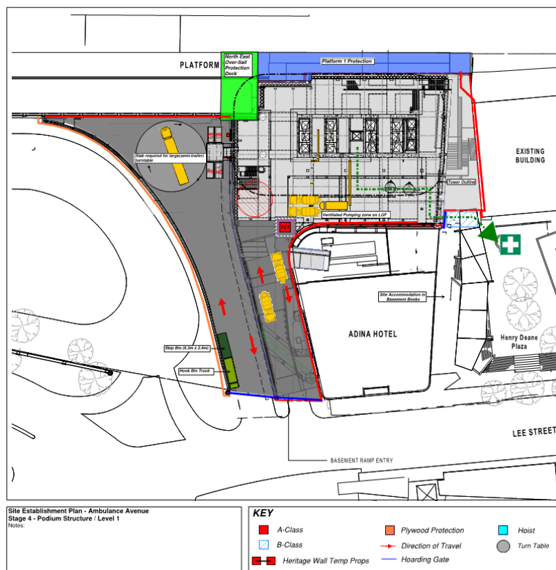
Figure 1.39c: Phase 3 – tower construction egress pathway
