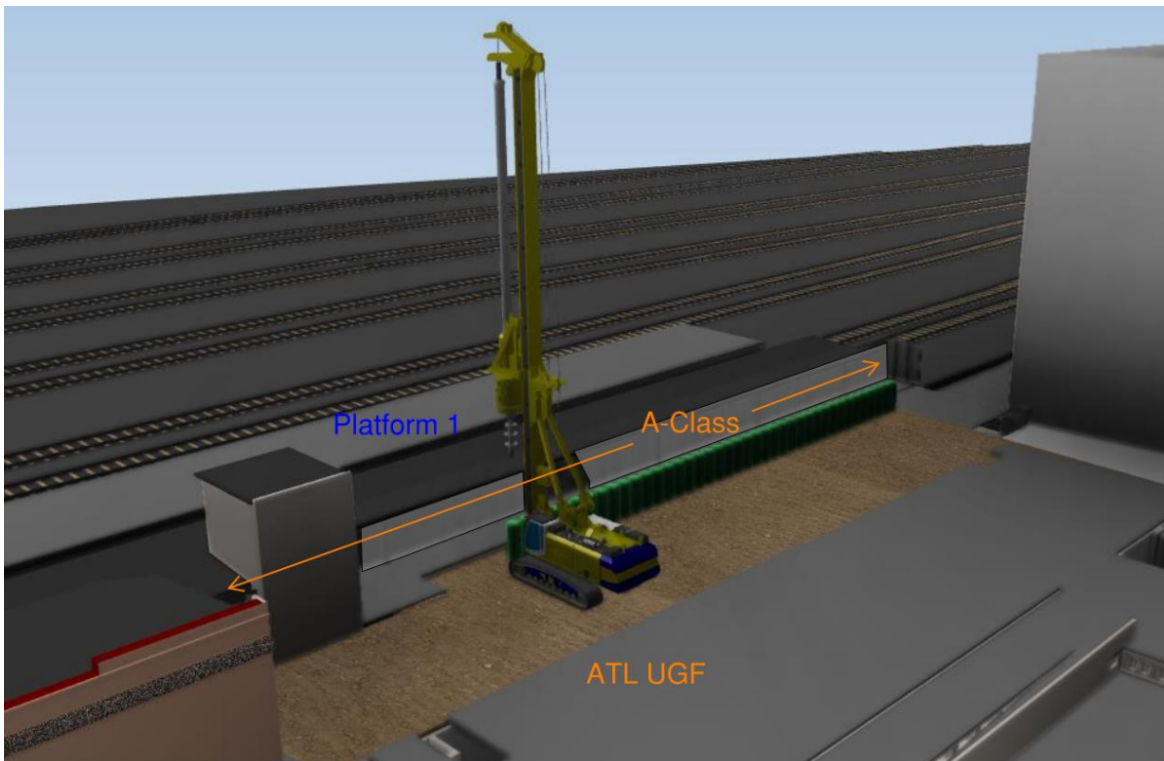
Figure 1-23: Example of A-Class hoarding in relation to piling works
