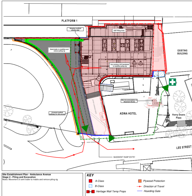
Figure 1-39b: Phase 2 – excavation and basement construction egress pathway
