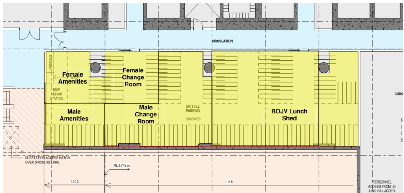
Figure 1-34: Site Accommodation – Basement 2 Bicycle Parking
