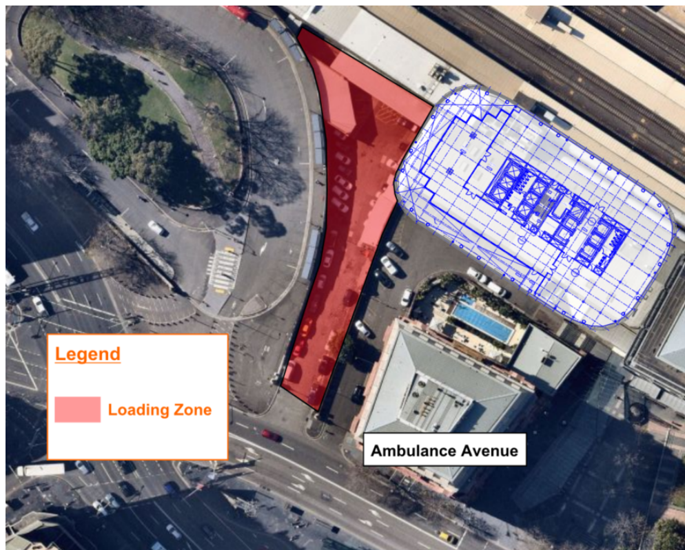
Figure 1-25b: Loading Zone Layout Plan – Ambulance Avenue
