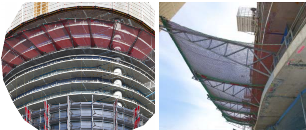
Figure 1-59b: Photographic Example of Perimeter Catch Fan Systems
