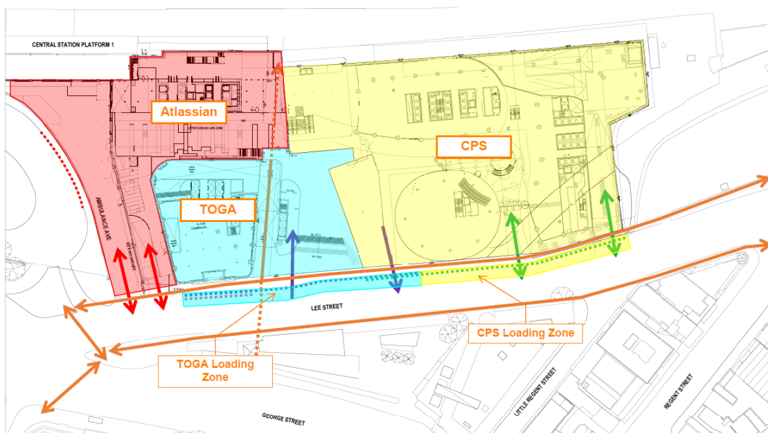
Figure 1-5: Western Gateway Precinct vehicle pathway overview
