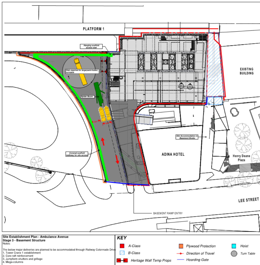
Figure 1-13: Site Establishment Plan
