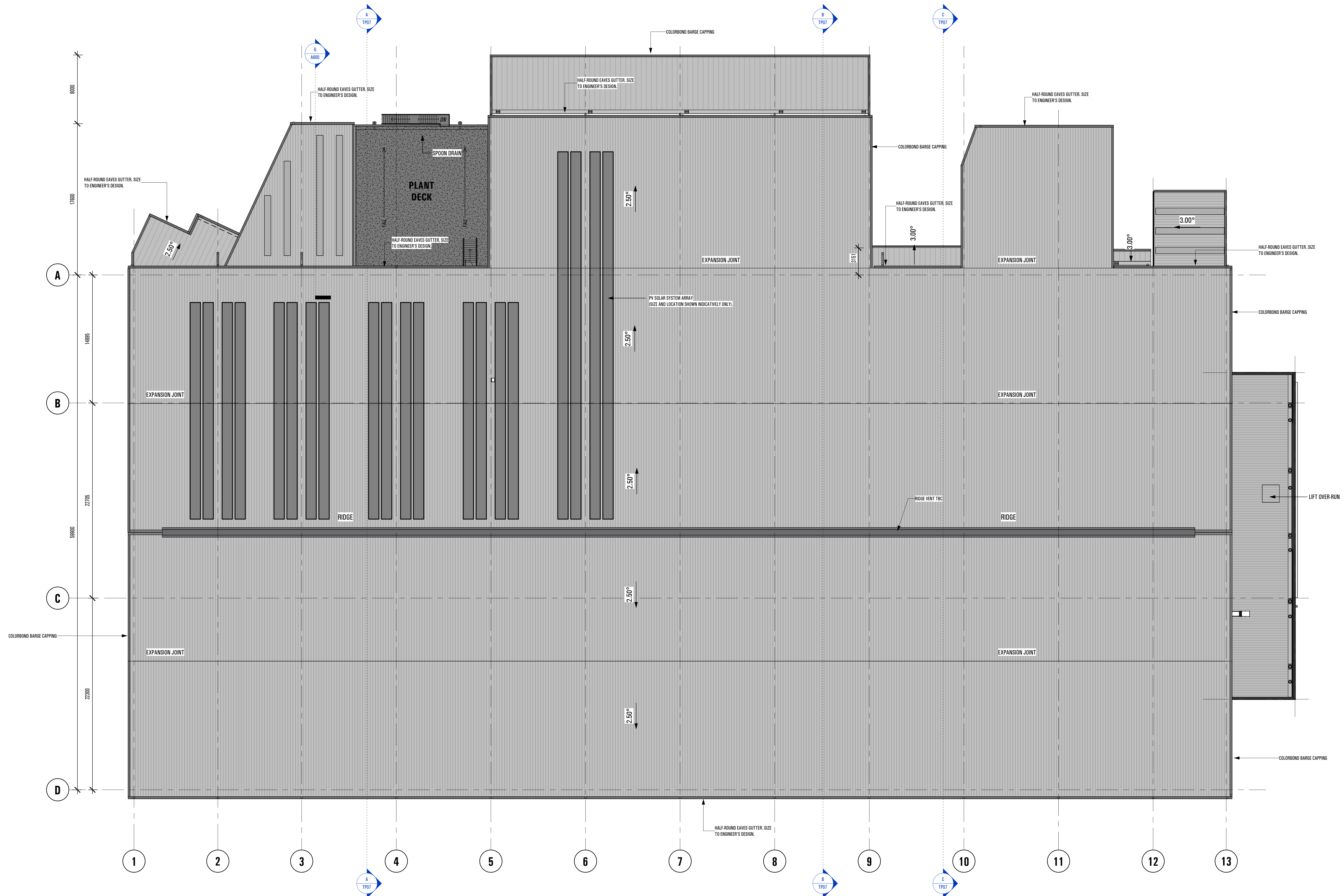
ROOF PLAN 1:200
