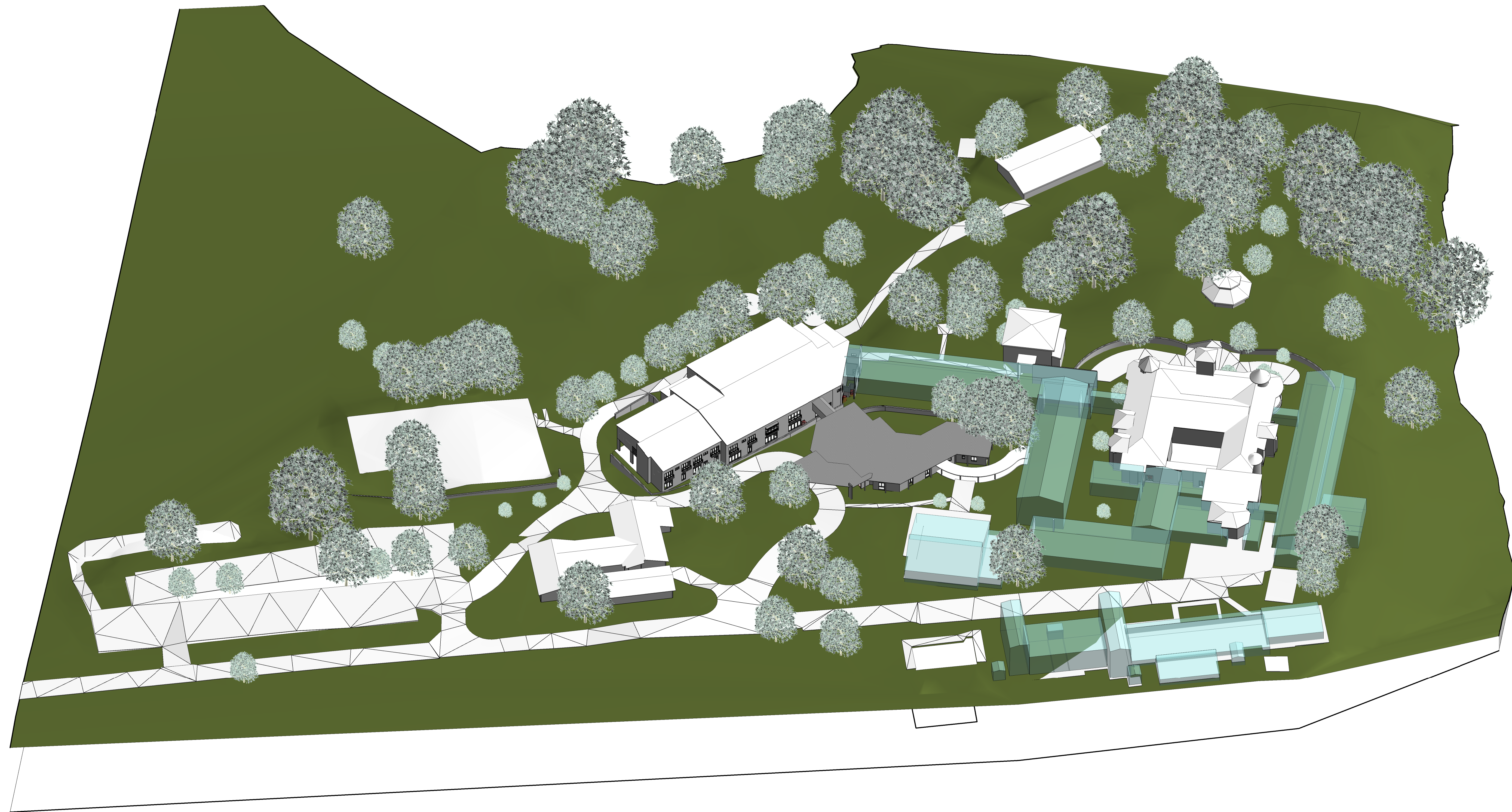
2 3D Site - Demolition Volumes 3D View SCALE
