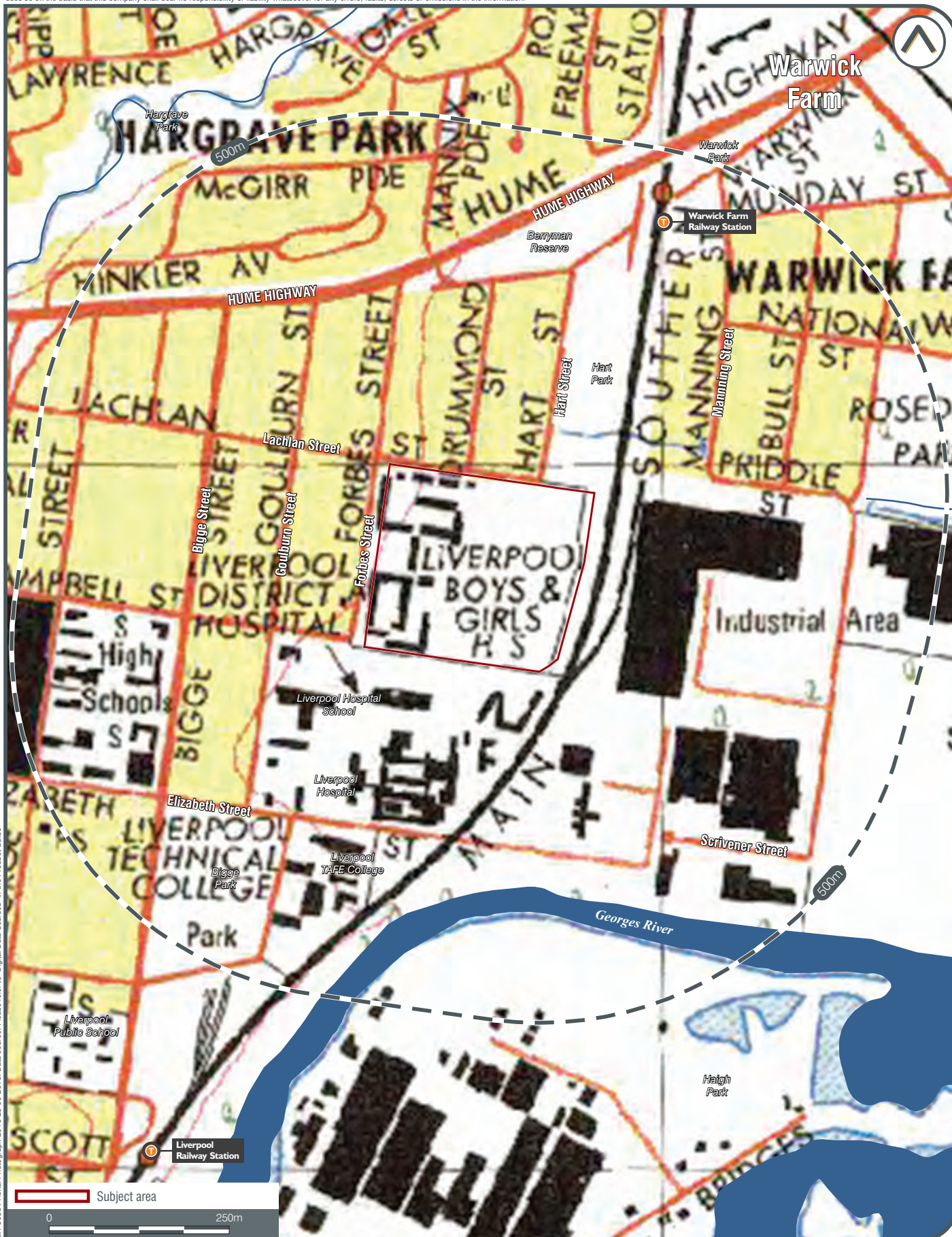
1969-1991 TOPOGRAPHIC MAP SERIES (LIVERPOOL 9030-2S)
