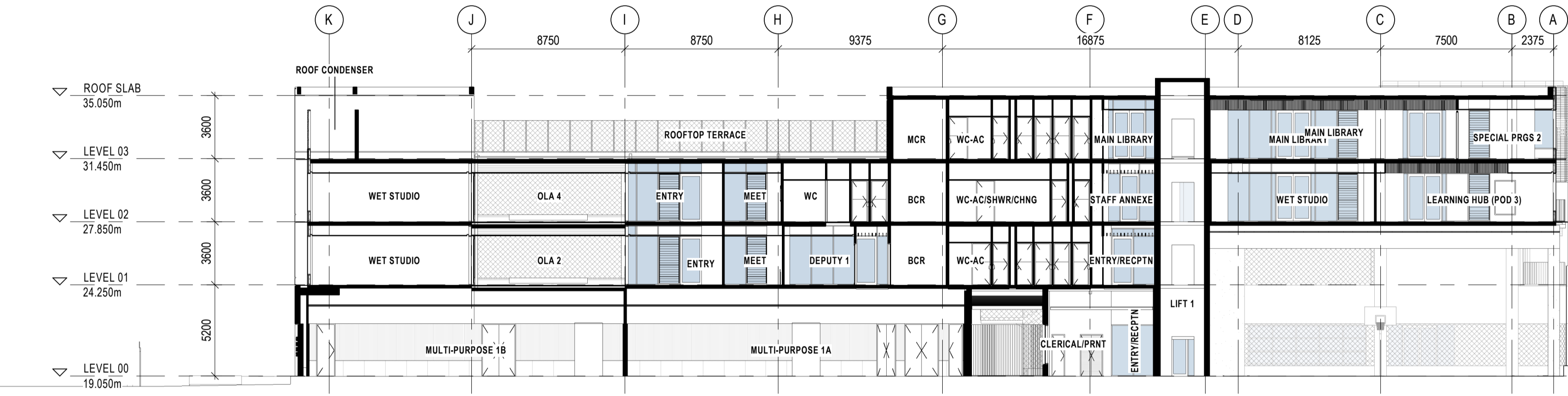
1 SECTION 01 1:200
