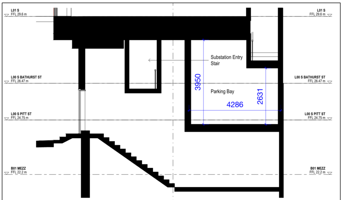
Figure 4-11: Cross section A elevation view between level B01 Mezz and level L01 S
