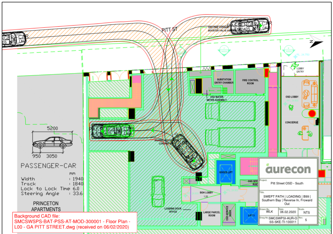
Figure 4-10: Vehicle swept path analysis for the B99 southern service bay – forward in and reverse out from bay
