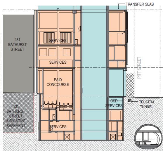
Figure 2-4: Pitt Street Station (East-West Section)
