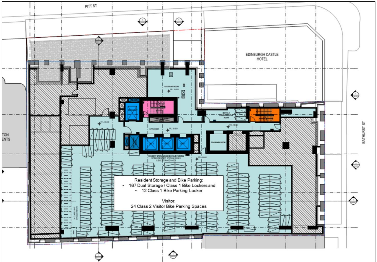
Figure 4-15: On-site bicycle parking provision on level 3 (drawing no: SMCSWSPS-BAT-OSS-AT-DWG-930341, Revision C)
