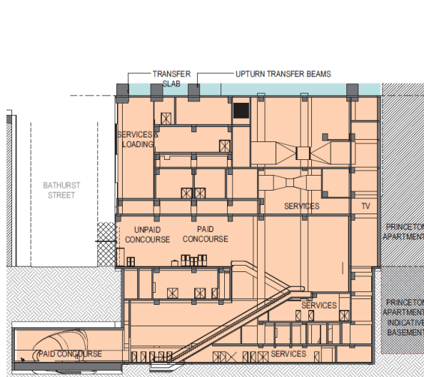
Figure 2-3: Pitt Street Station (North-South Section)
