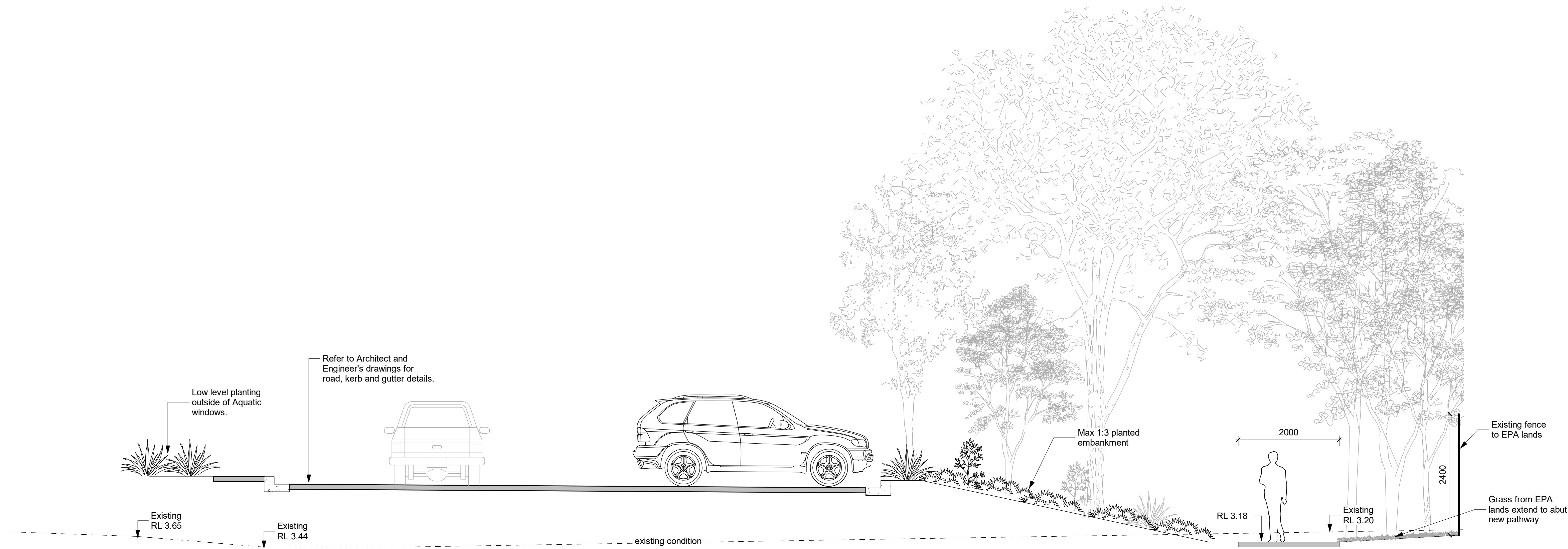
1 Proposed Building Western Interface 1 : 50
