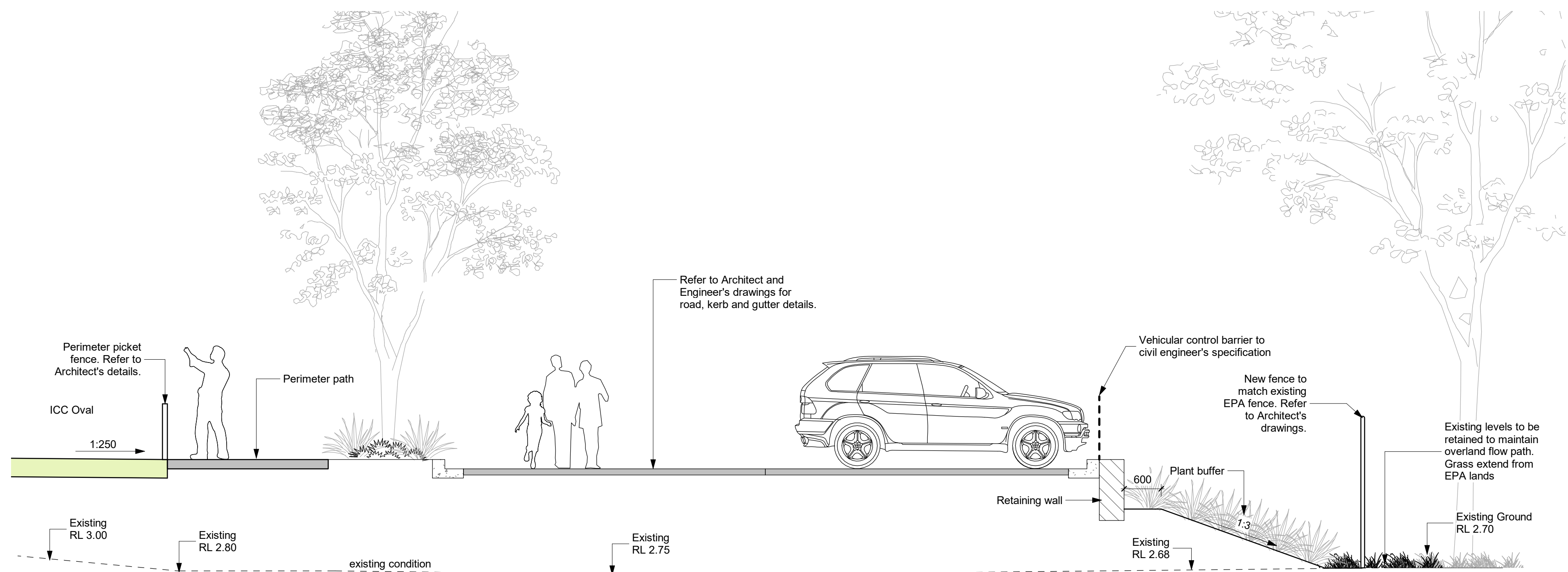
2 ICC Oval & New shared path 1 : 50
