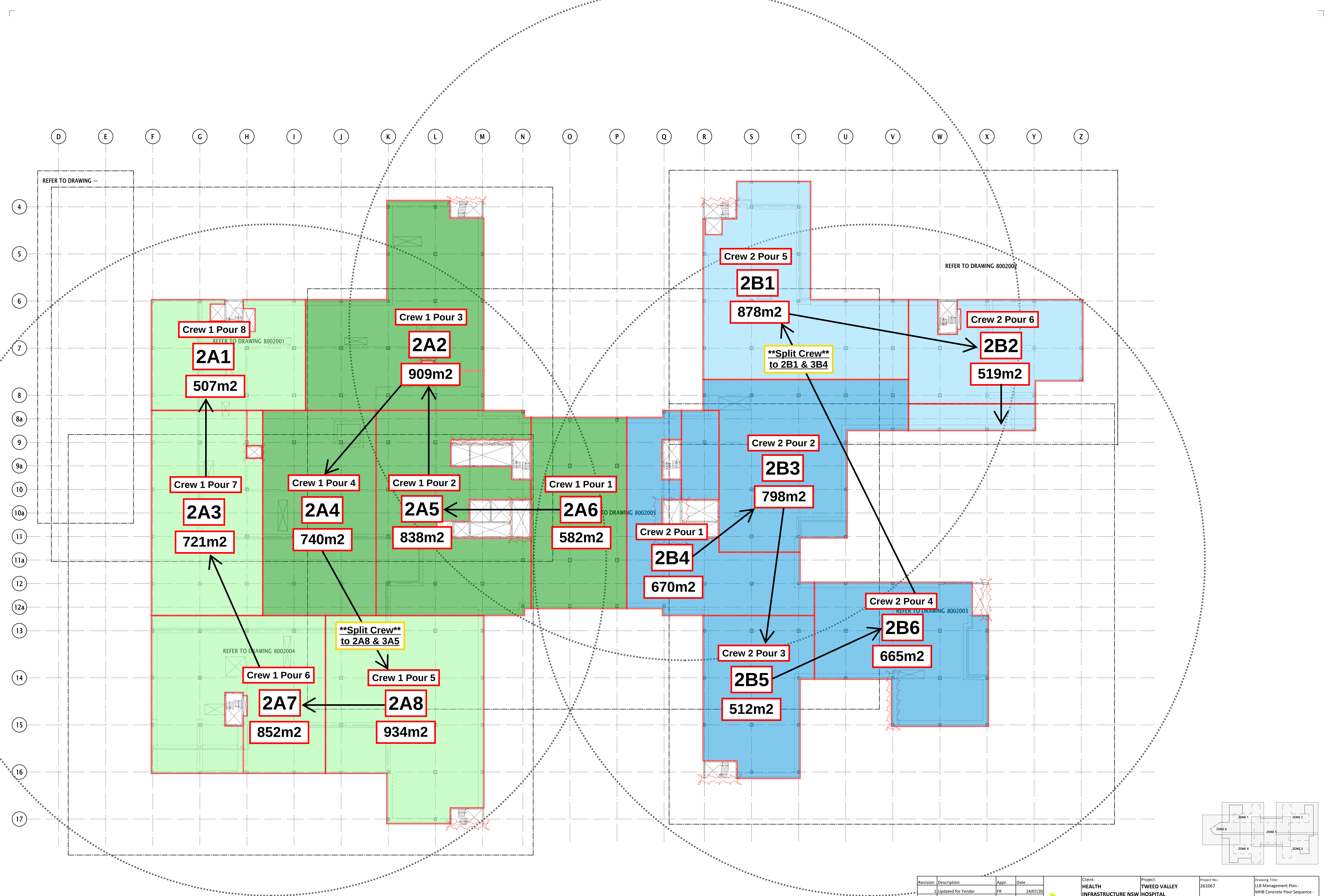
LEVEL 02 OVERALL GENERAL ARRANGEMENT PLAN SCALE 1:200
