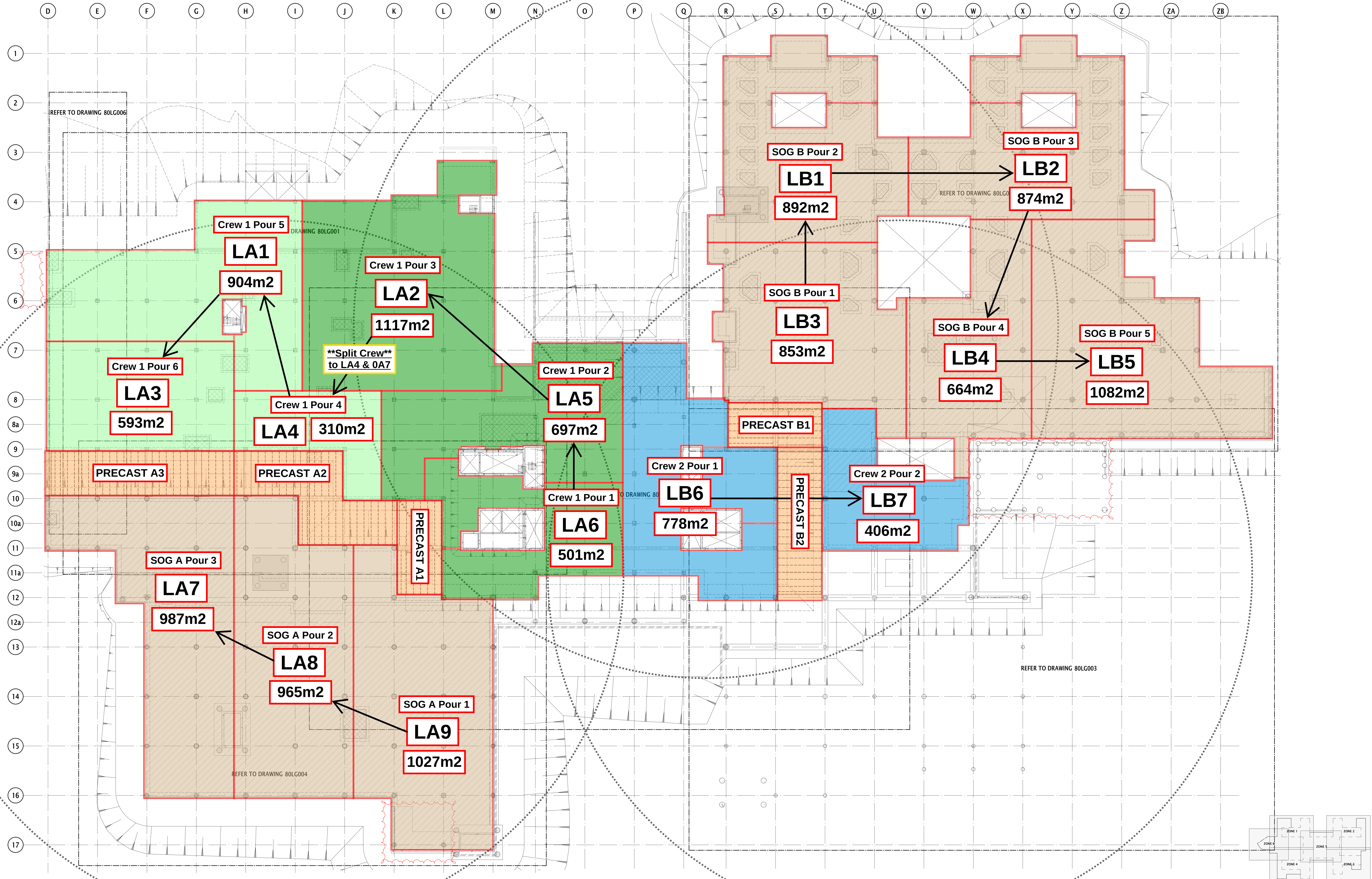
LOWER GROUND OVERALL GENERAL ARRANGEMENT PLAN SCALE 1:200
