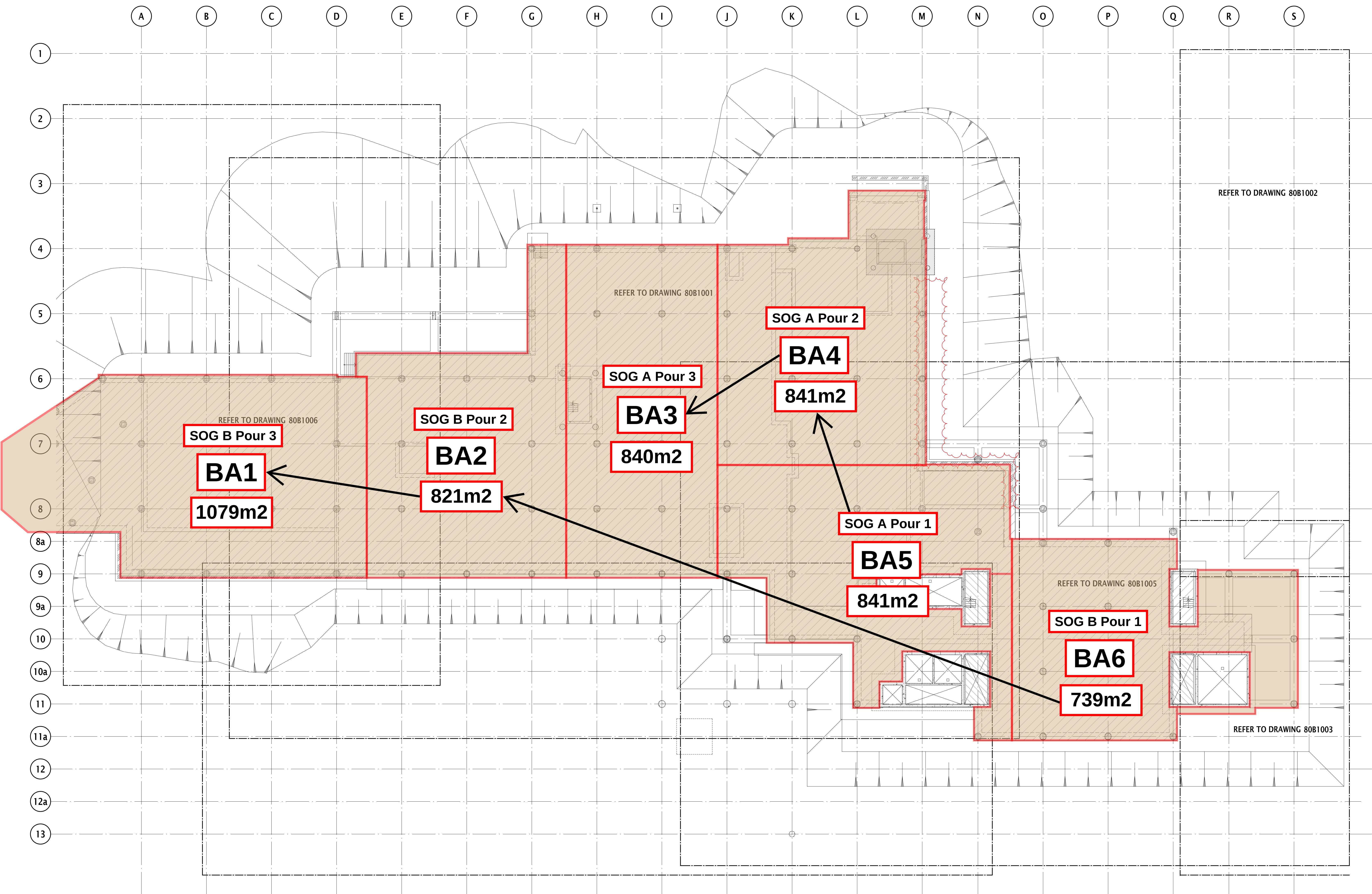
BASEMENT 1 OVERALL GENERAL ARRANGEMENT PLAN SCALE 1 : 200
