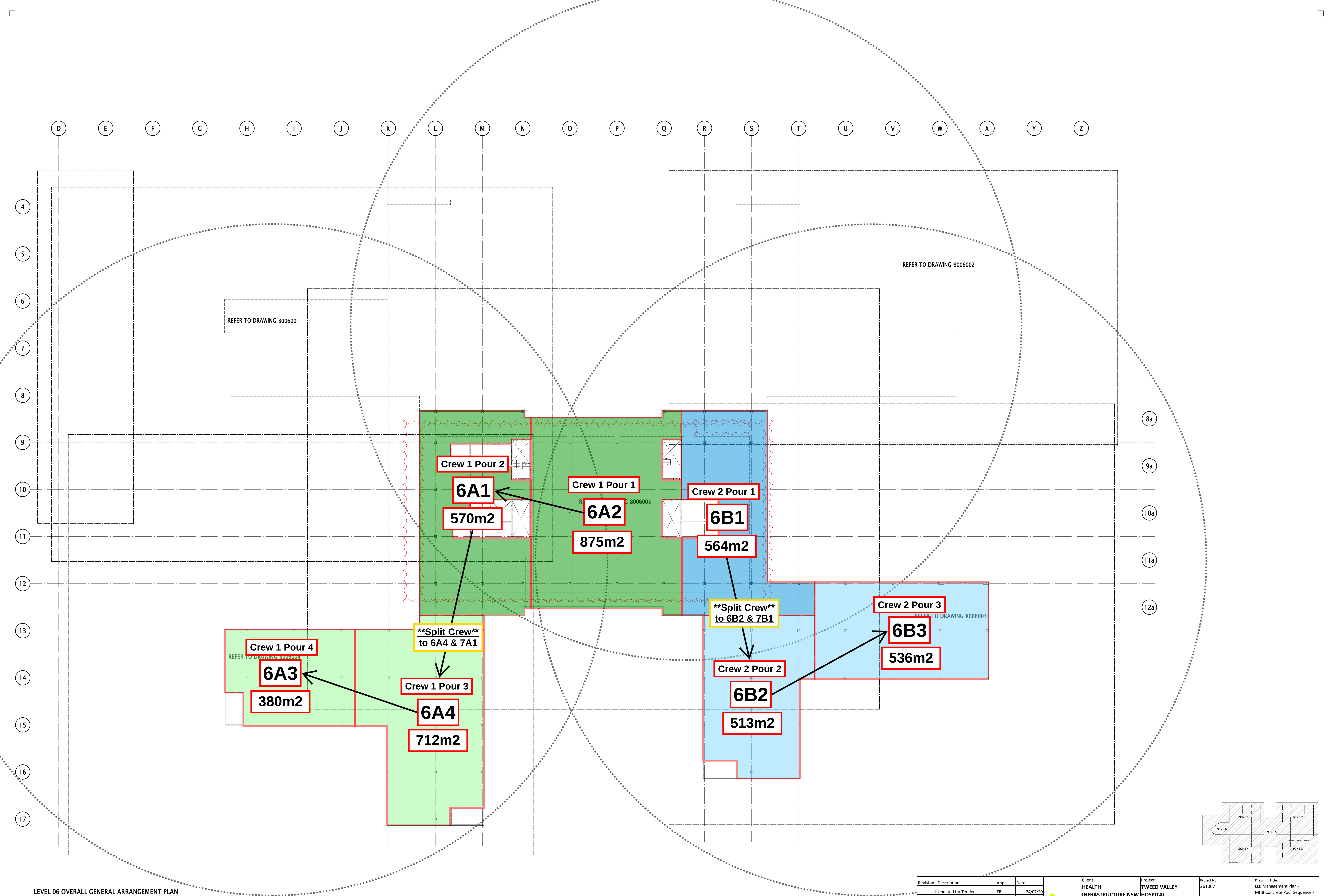
LEVEL 06 OVERALL GENERAL ARRANGEMENT PLAN
